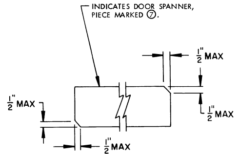
BEVEL-CUT
