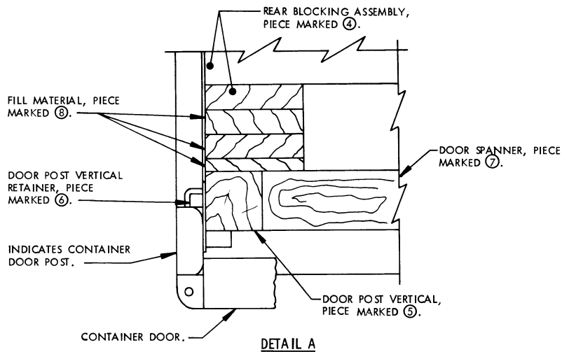
DETAIL A A PARTIAL PLAN VIEW OF THE LEFT REAR PORTION OF THE CONTAINER IS SHOWN DEPICTING THE PROPER POSITION OF THE DOOR POST VERTICAL AND ADJACENT DUNNAGE PIECES.
