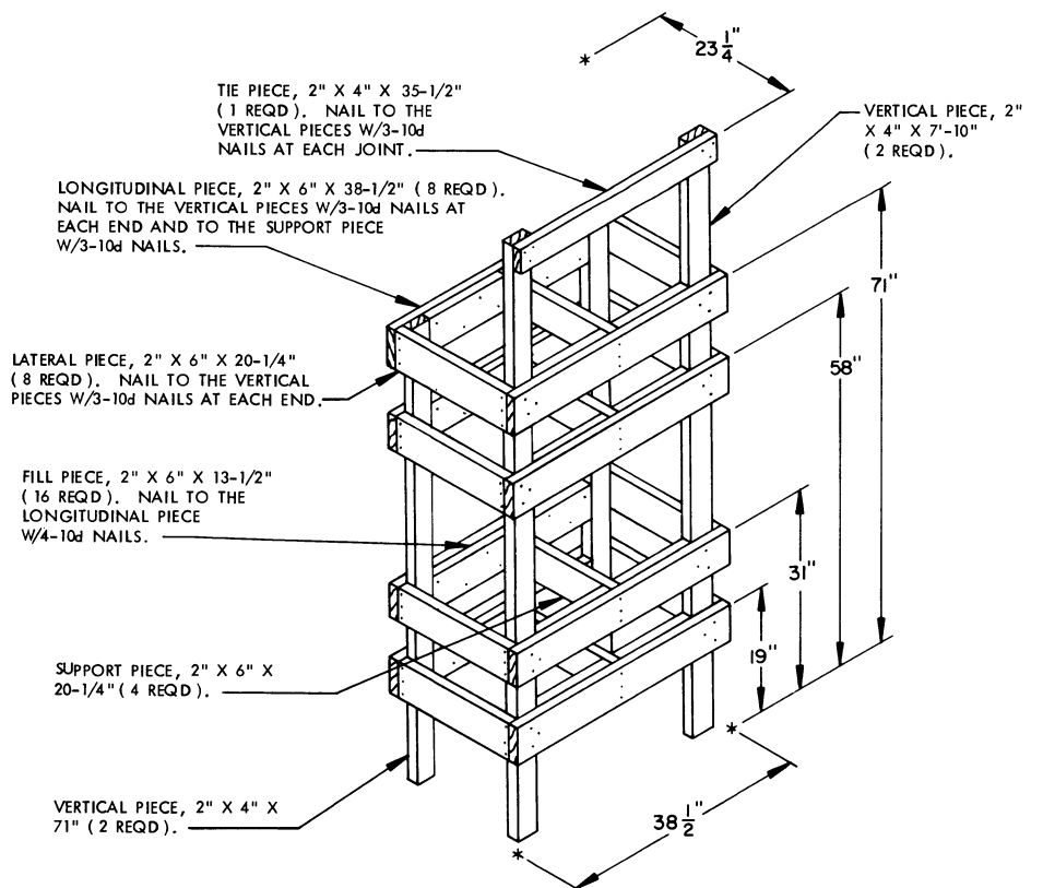
FILLER ASSEMBLY
