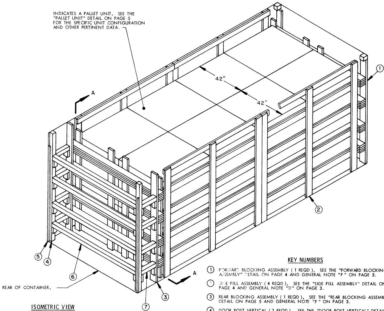
ISOMETRIC VIEW
