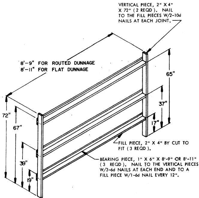
SIDE FILL GATE
