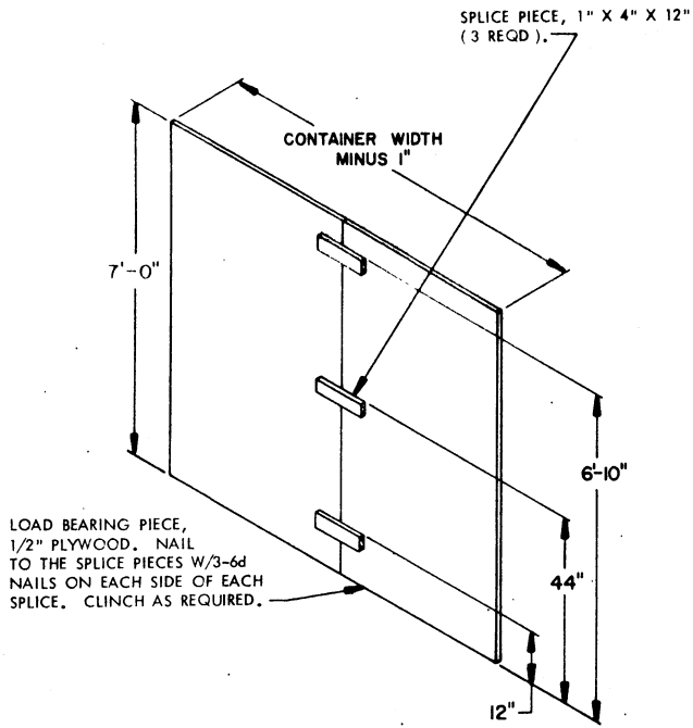
LOAD BEARING GATE
