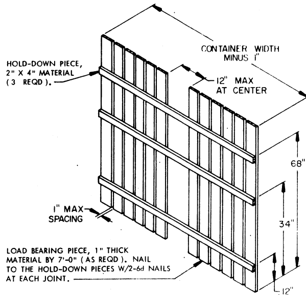
ALTERNATIVE LOAD BEARING GATE
