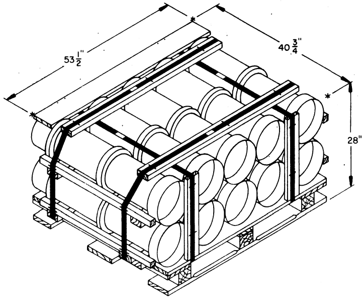
PALLET UNIT ( MODIFIED )
