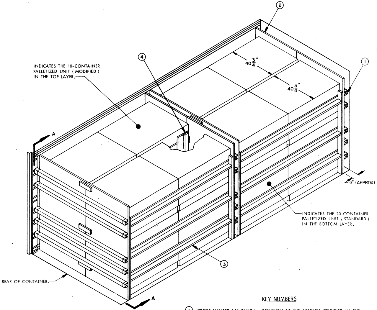
ISOMETRIC VIEW
