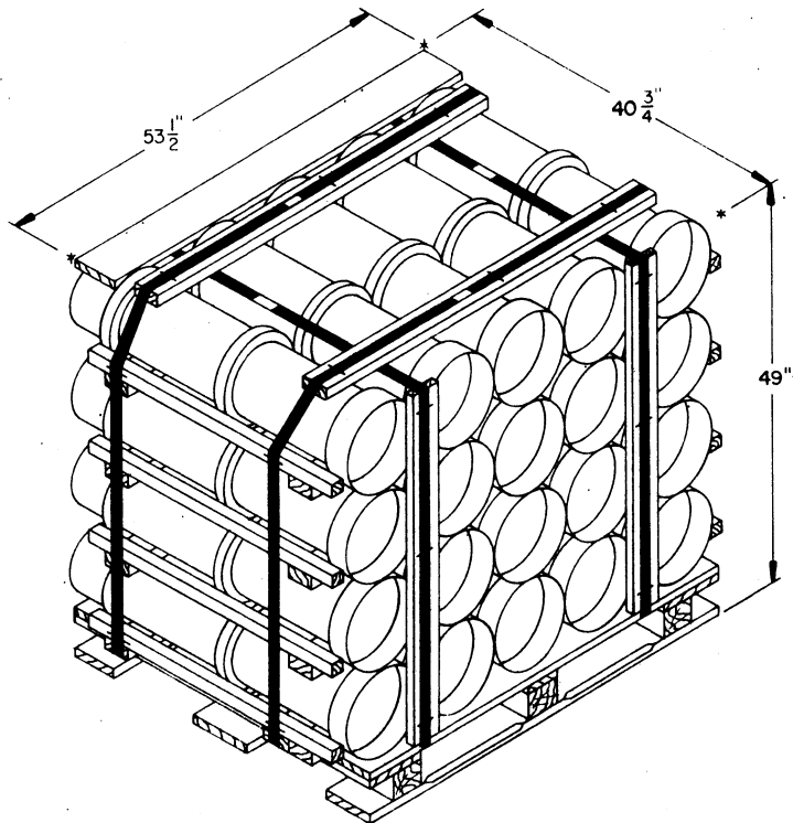
PALLET UNIT ( STANDARD )
