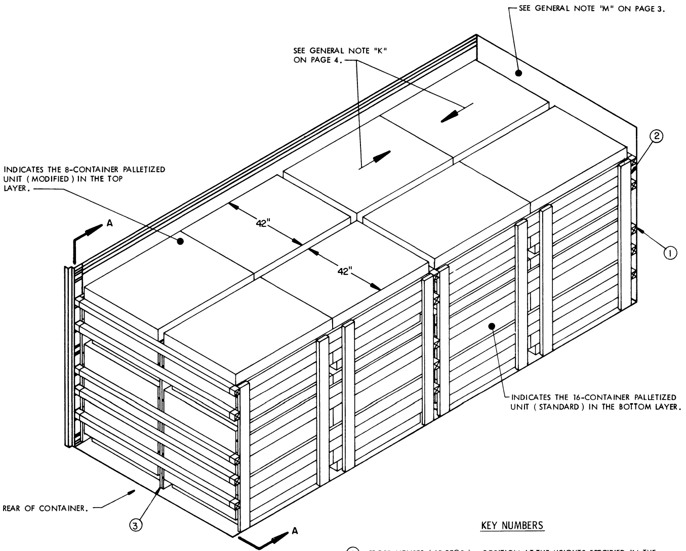
ISOMETRIC VIEW
