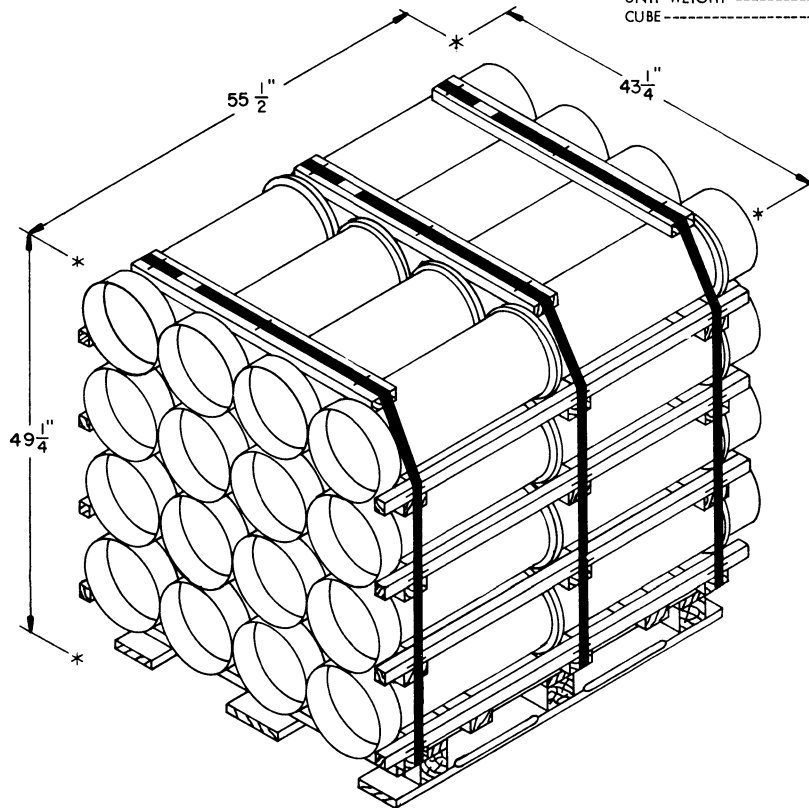
PALLET UNIT ( STANDARD ) FLAT DUNNAGE
