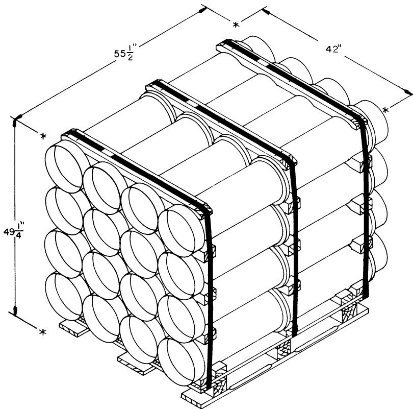
PALLET UNIT ( STANDARD ) ROUTED DUNNAGE
