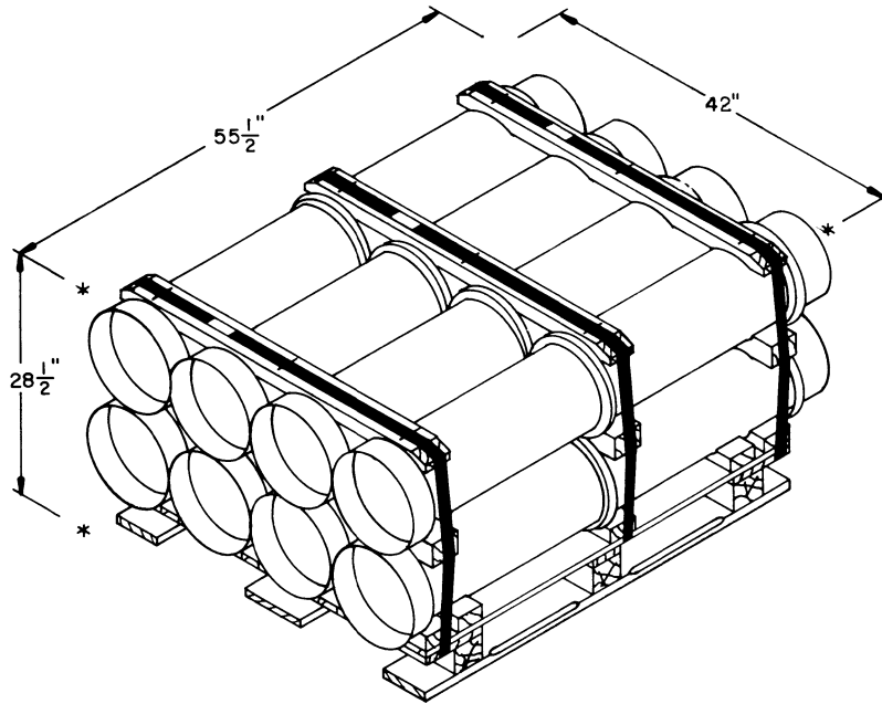
PALLET UNIT ( MODIFIED ) ROUTED DUNNAGE
