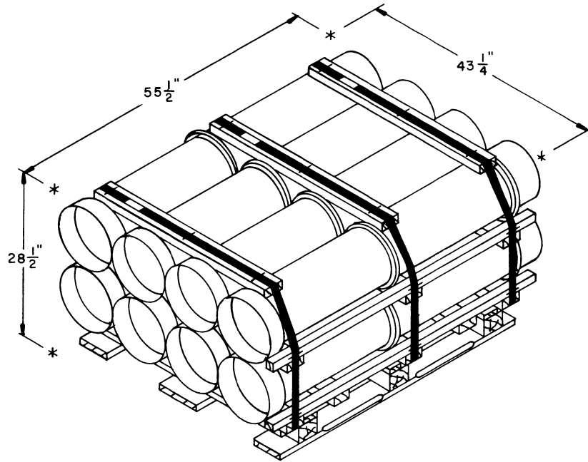
PALLET UNIT ( MODIFIED ) FLAT DUNNAGE
