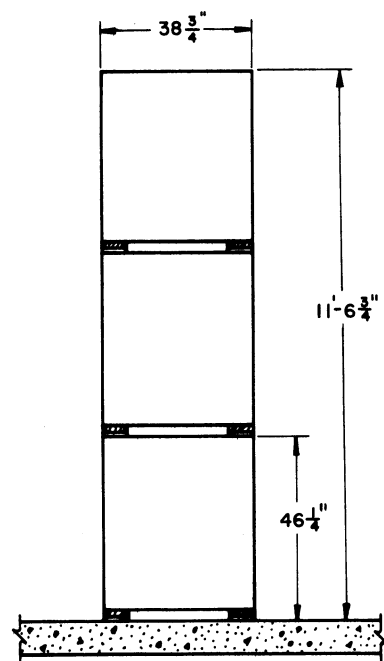
TYPICAL STACK
