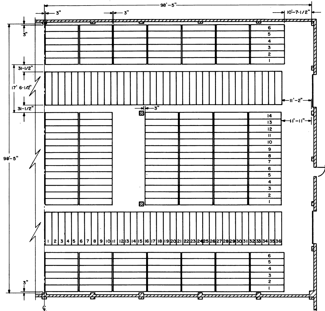
PLAN VIEW 1/4 WAREHOUSE
