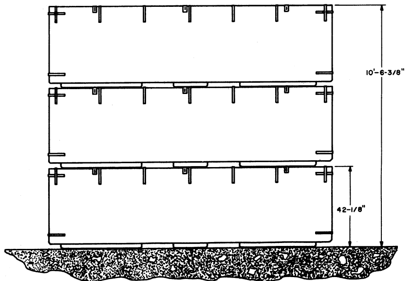
TYPICAL STACK
