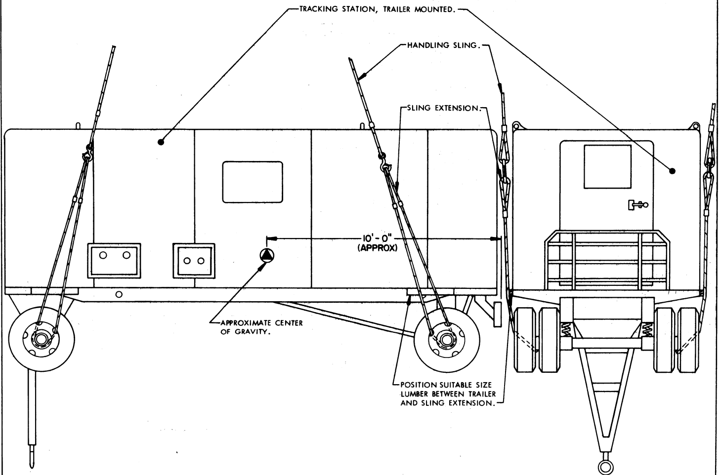
ELEVATION VIEW
