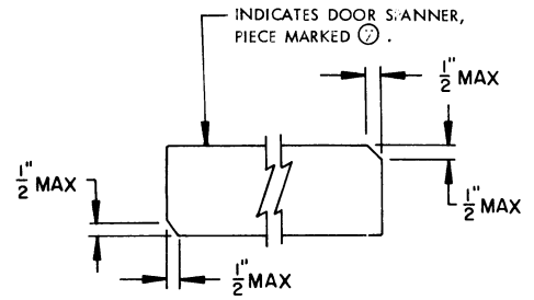
BEVEL-CUT
