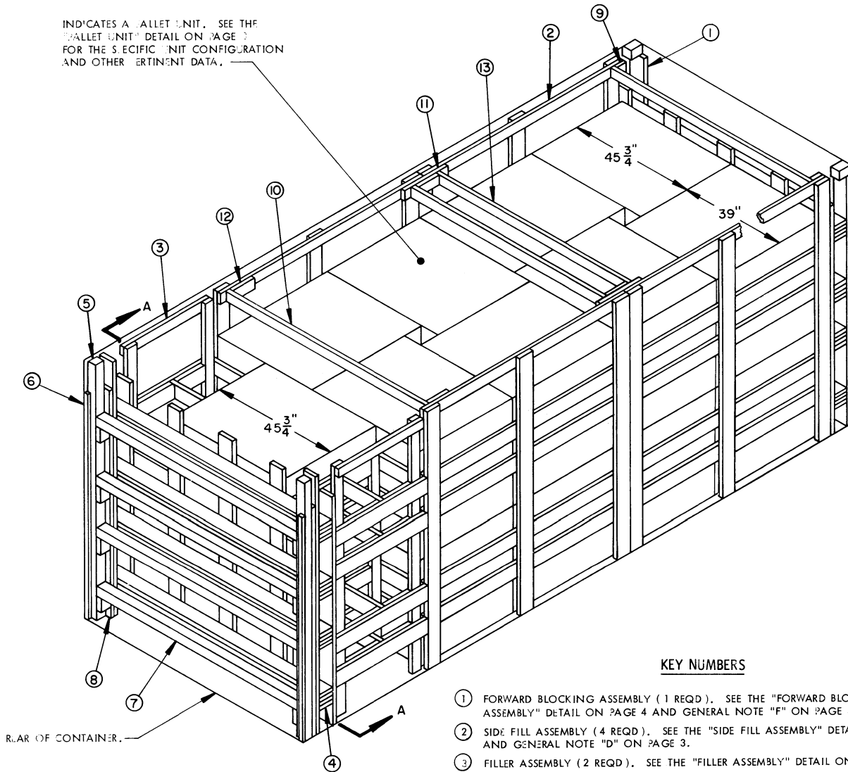
ISOMETRIC VIEW
