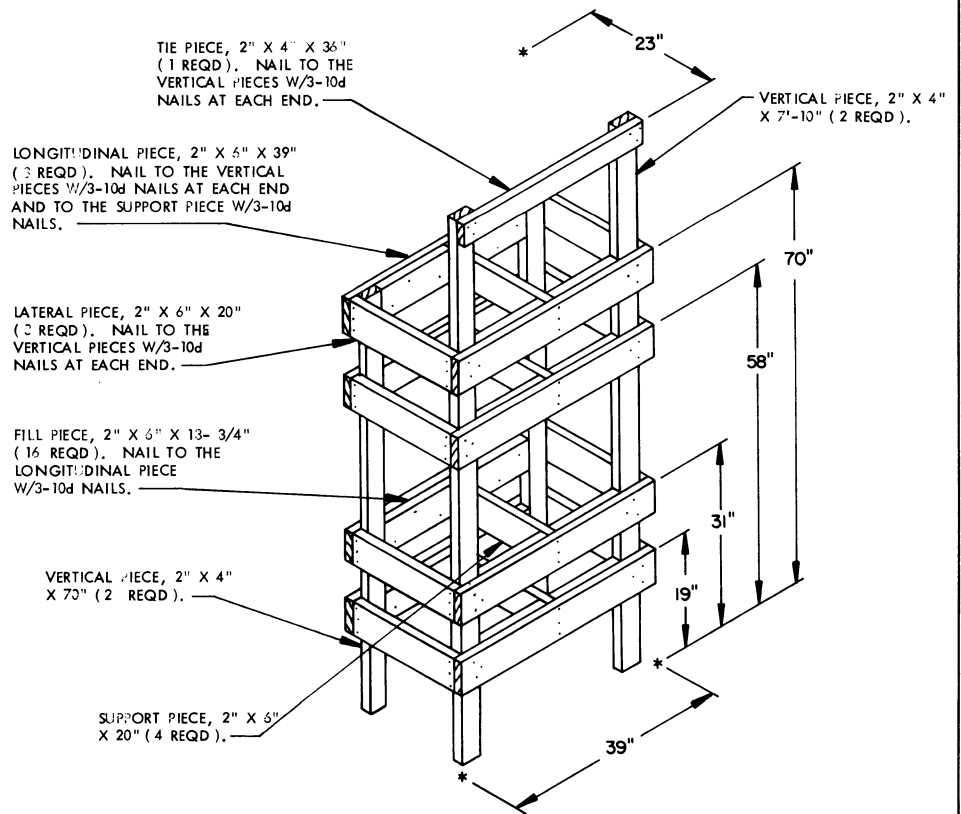
FILLER ASSEMBLY
