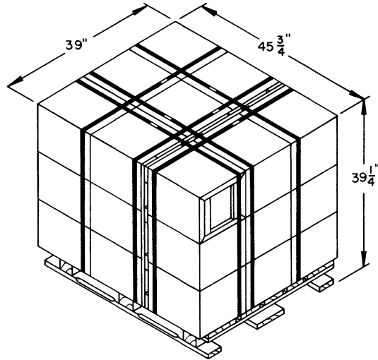
PALLET UNIT
