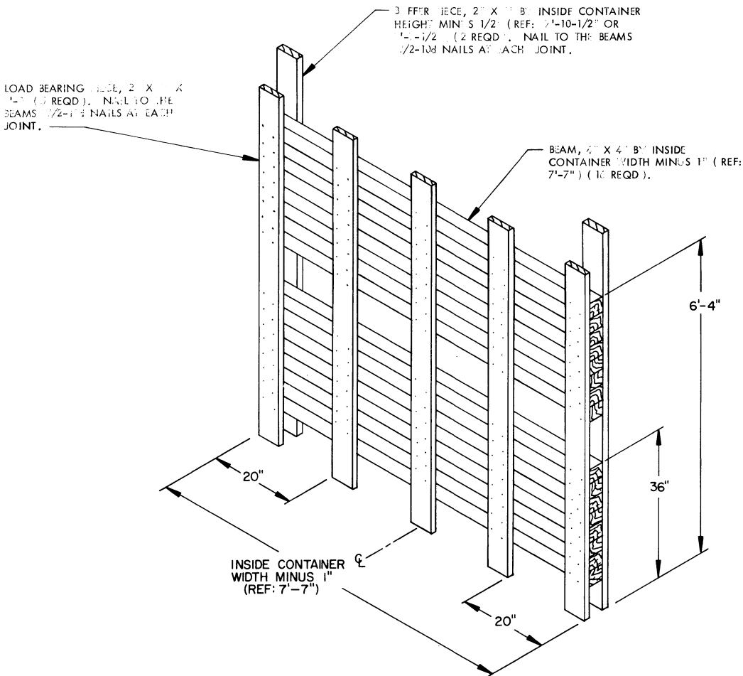
ALTERNATIVE FORWARD/REAR BLOCKING ASSEMBLY
