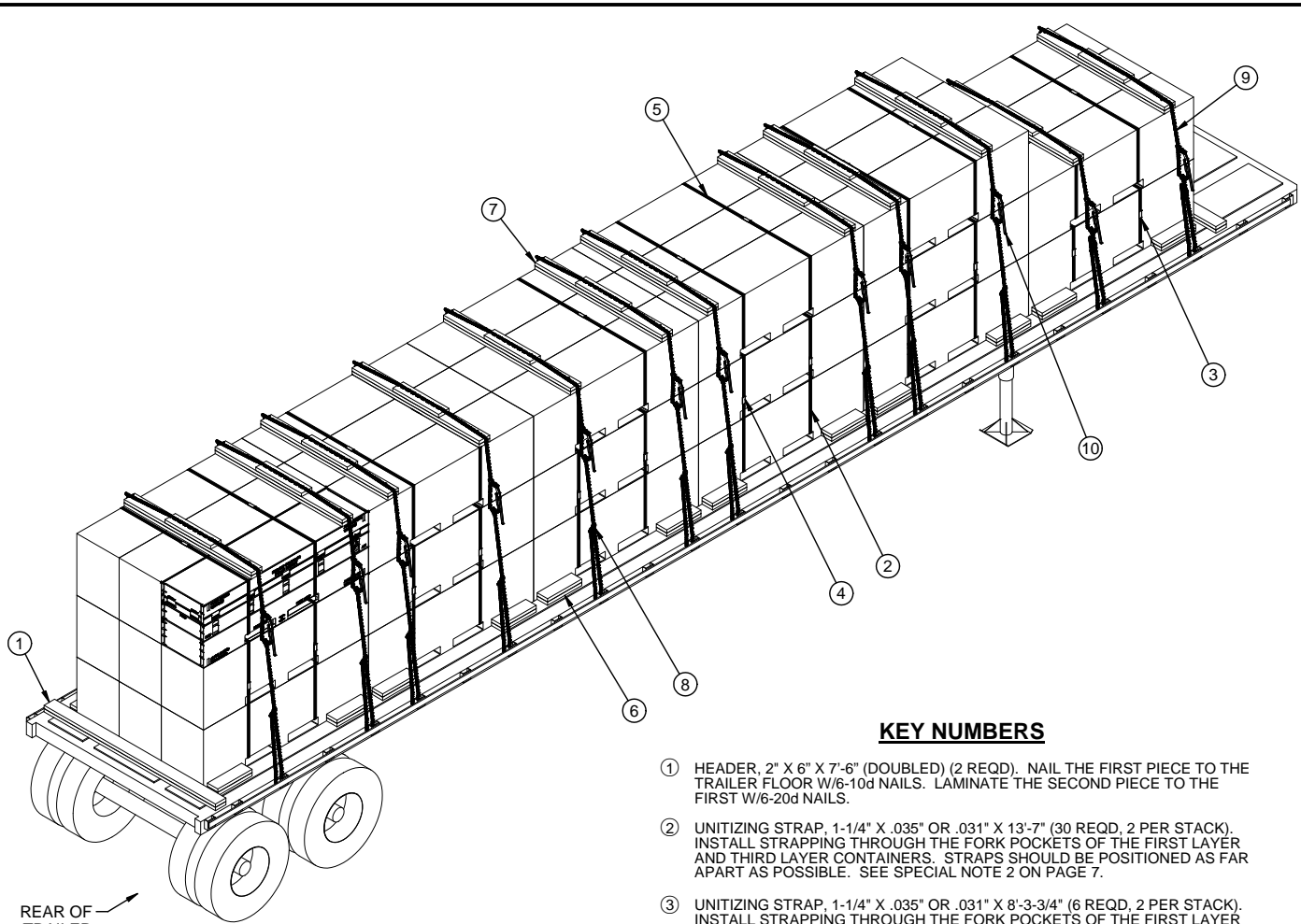
ISOMETRIC VIEW
