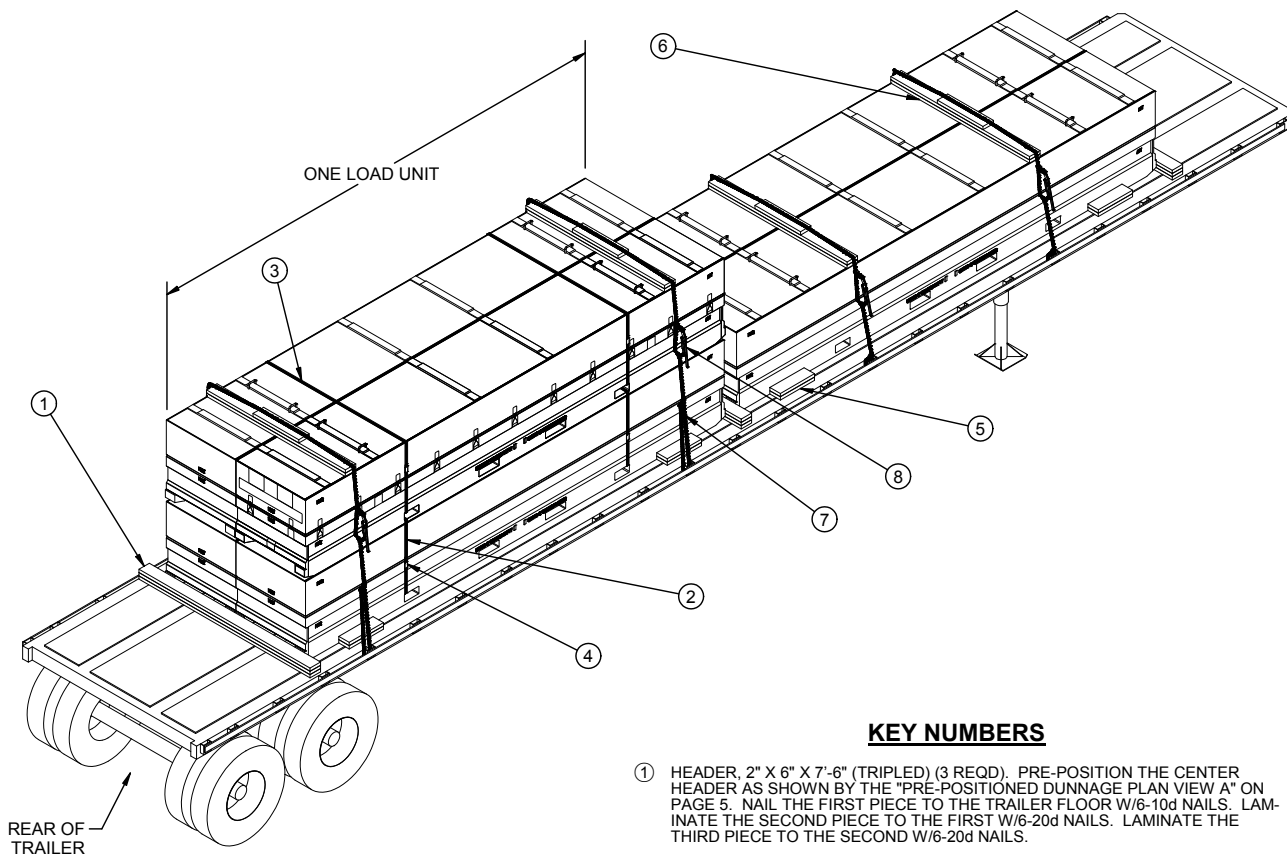
ISOMETRIC VIEW
