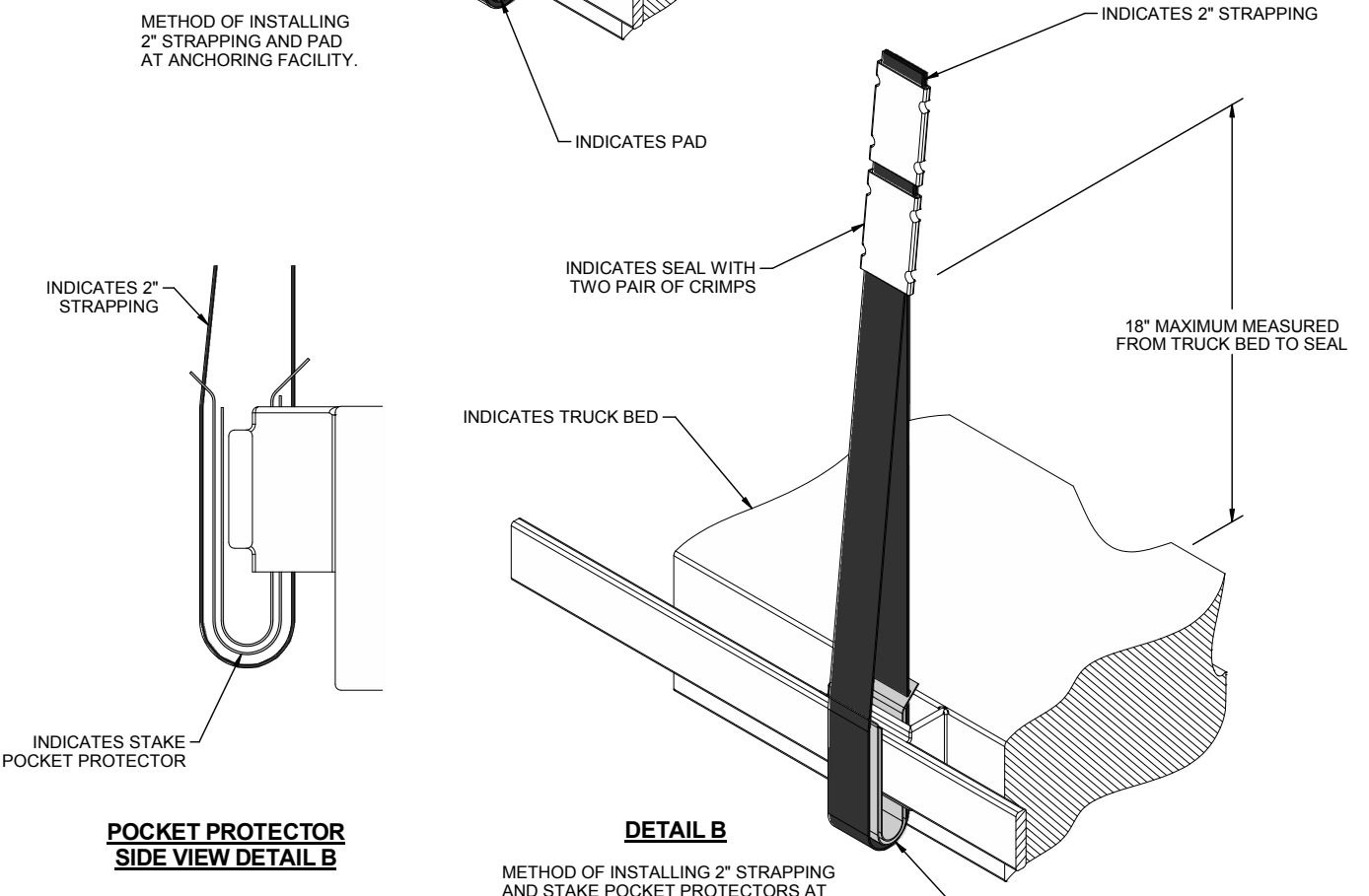
TWO STAKE POCKET PROTECTORS UNDER EACH ANCHORING FACILITY. SEE "POCKET PROTECTOR SIDE VIEW DETAIL B" AT LEFT.
