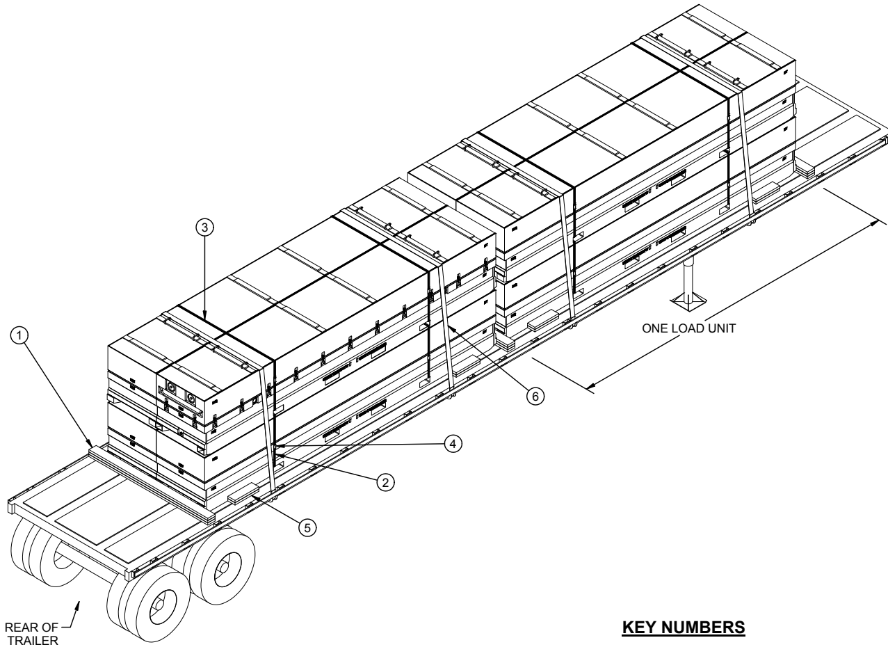
ISOMETRIC VIEW
