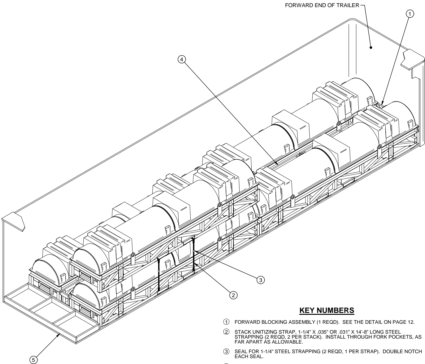
ISOMETRIC VIEW
