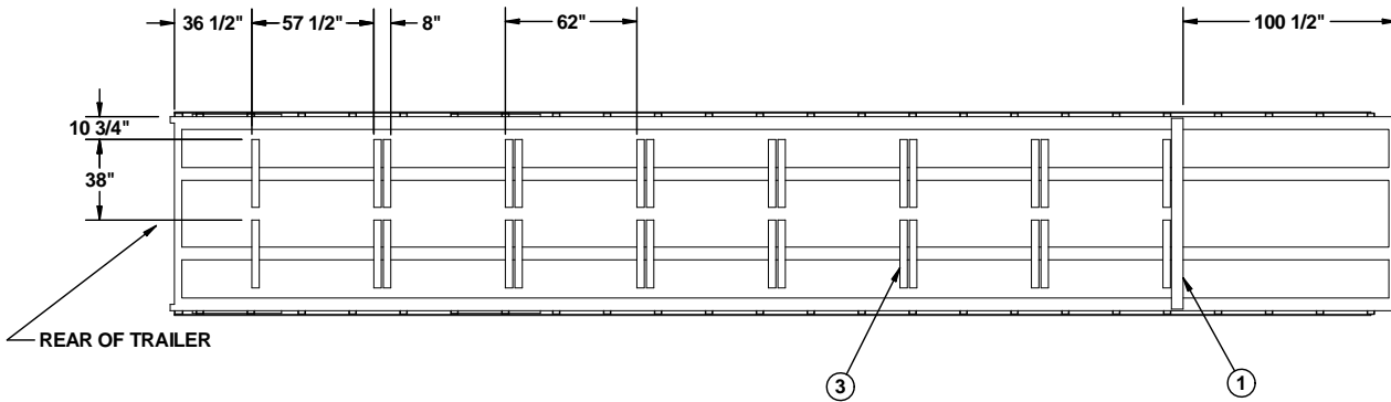
PRE-POSITIONED DUNNAGE PLAN VIEW B KEY NUMBERS REFER TO KEY NUMBERS ON PAGE 8
