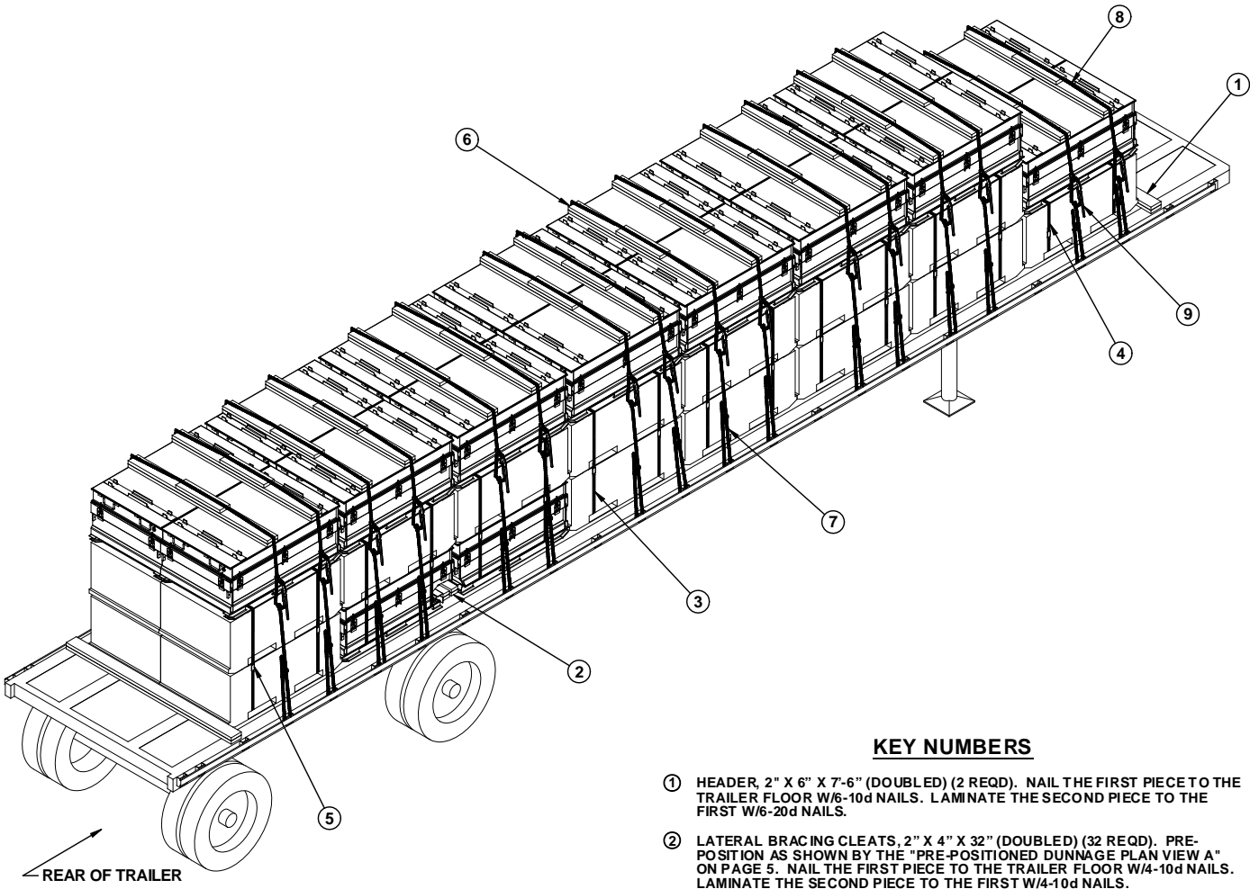
ISOMETRIC VIEW
