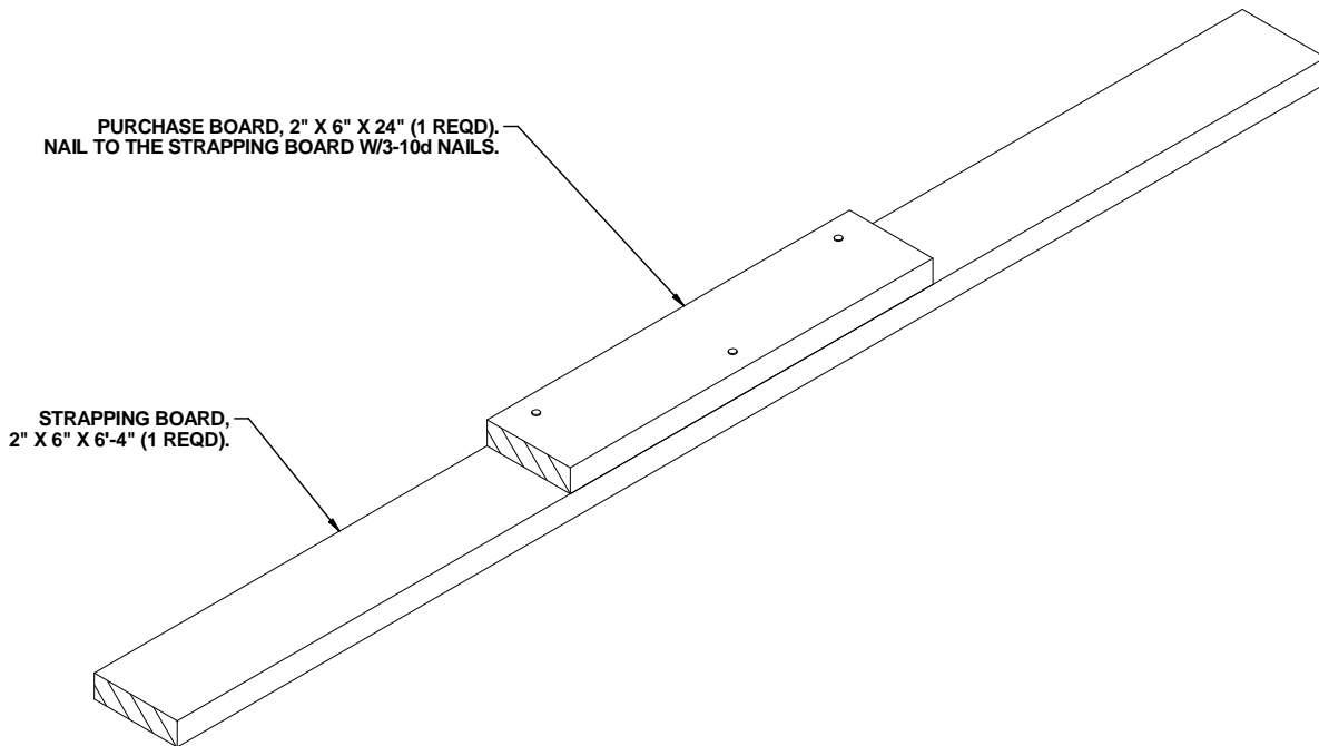
STRAPPING BOARD ASSEMBLY
