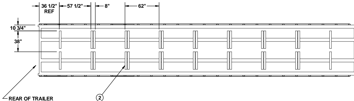
PRE-POSITIONED DUNNAGE PLAN VIEW A KEY NUMBERS REFER TO KEY NUMBERS ON PAGE 4 AND 6
