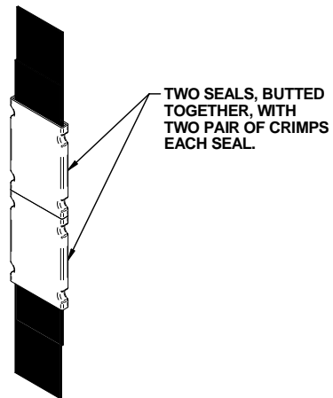
STRAP JOINT B
