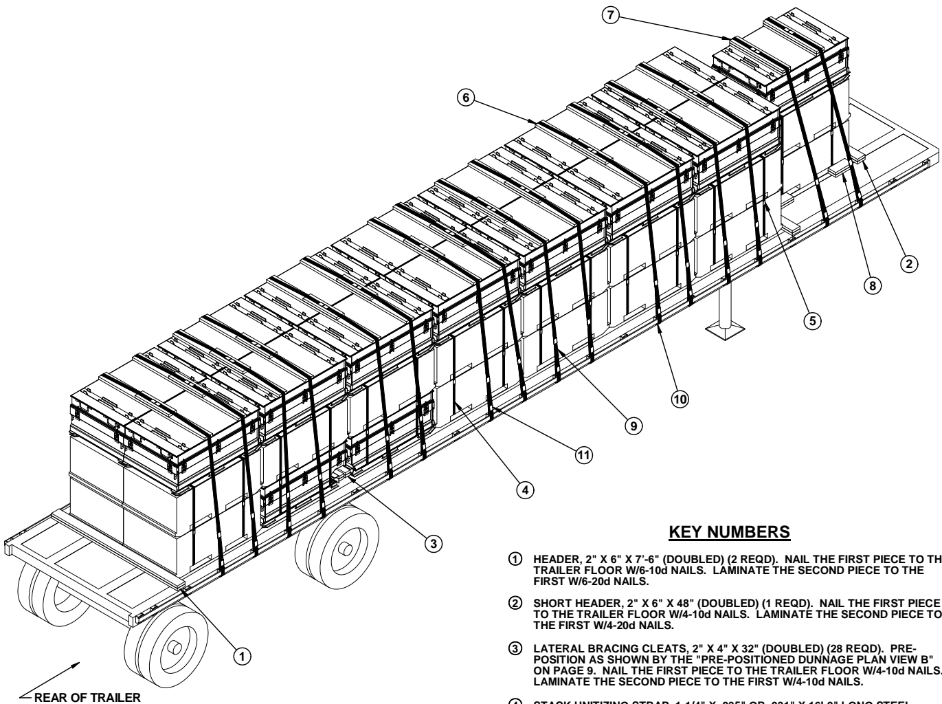
ISOMETRIC VIEW
