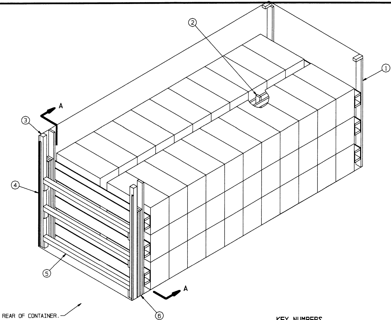
ISOMETRIC VIEW
