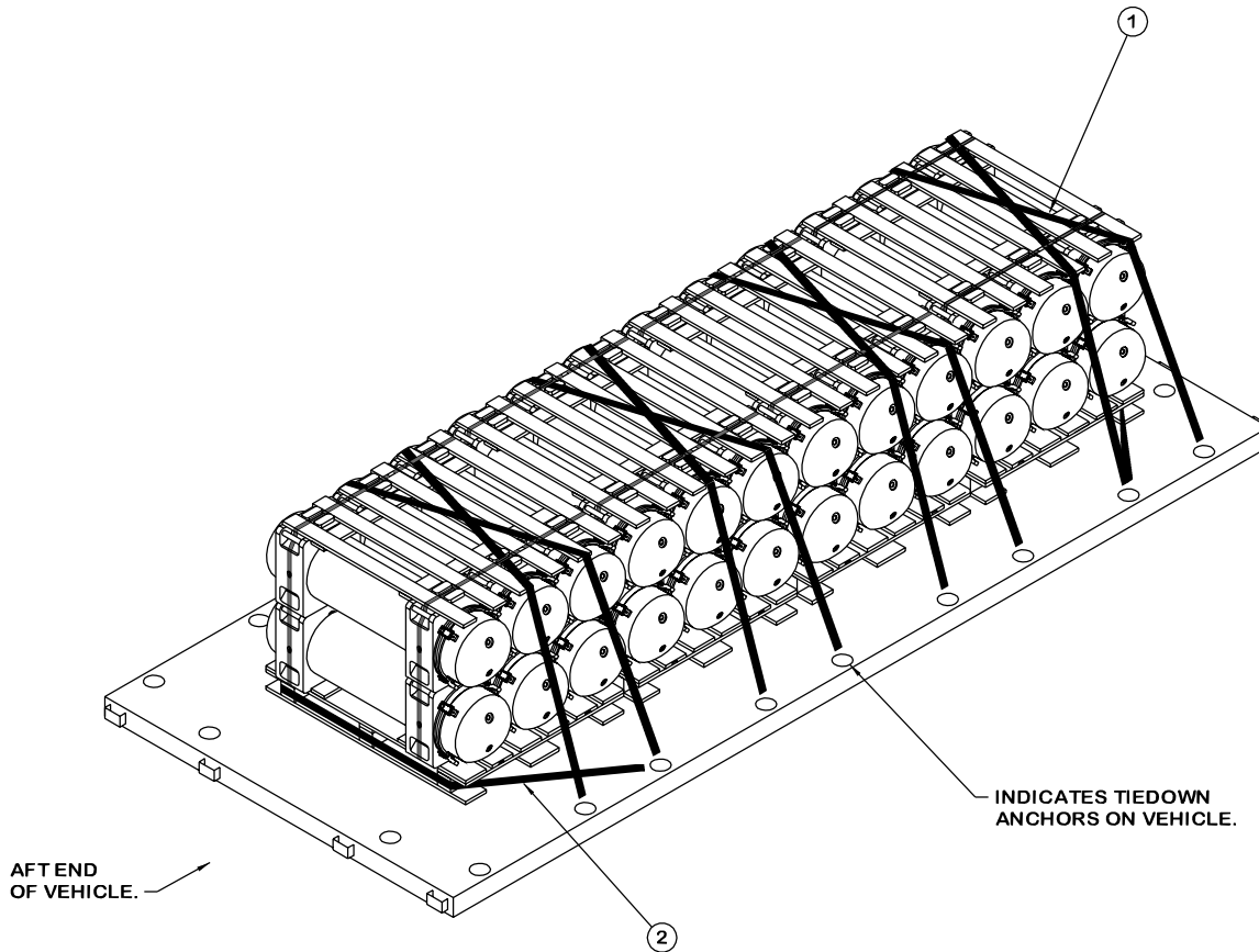
ISOMETRIC VIEW
