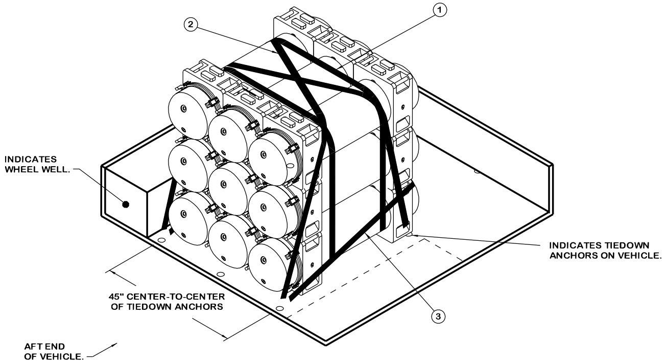
ISOMETRIC VIEW
