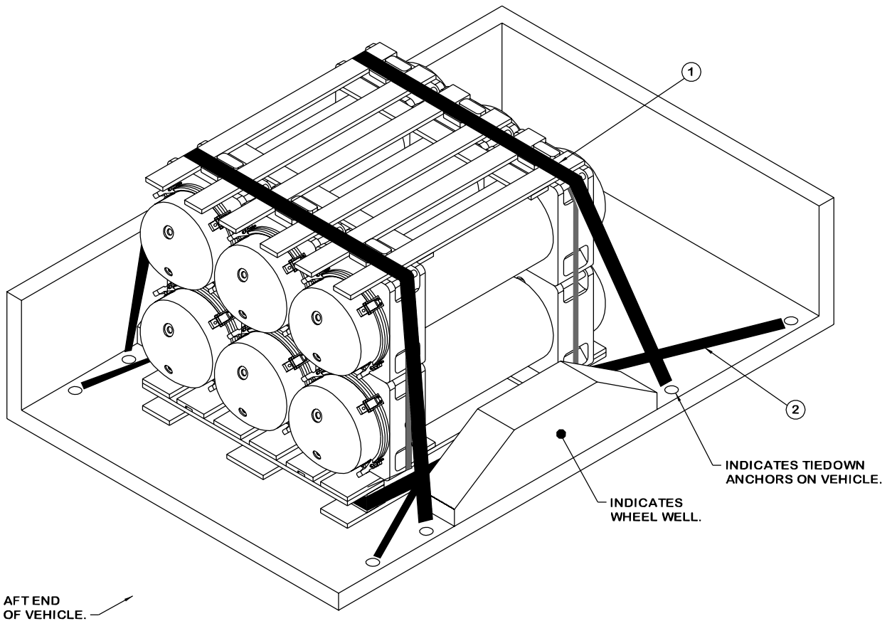
ISOMETRIC VIEW
