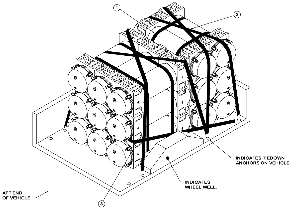
ISOMETRIC VIEW
