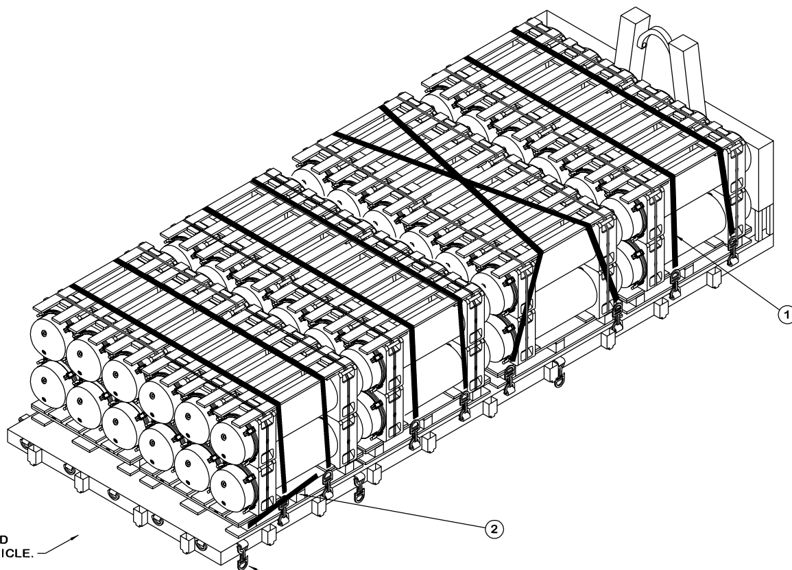
ISOMETRIC VIEW
