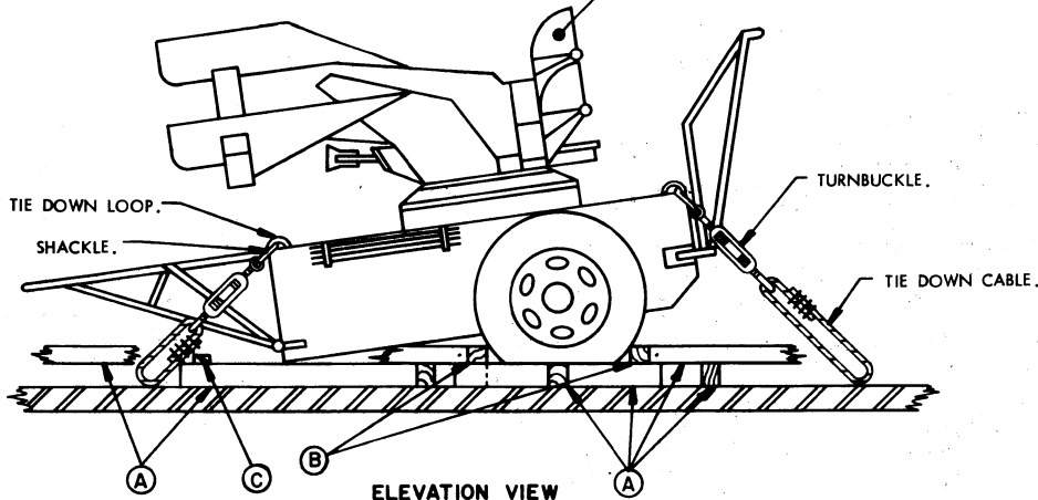
ELEVATION VIEW
