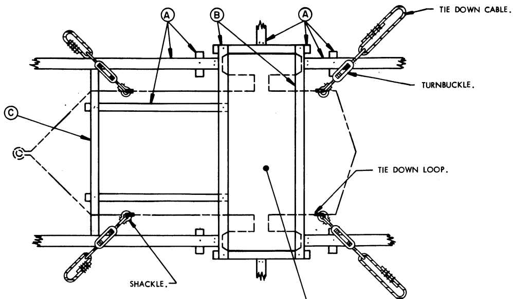
PLAN VIEW PHANTOM LINES INDICATE TRAILER AND TIRES.
