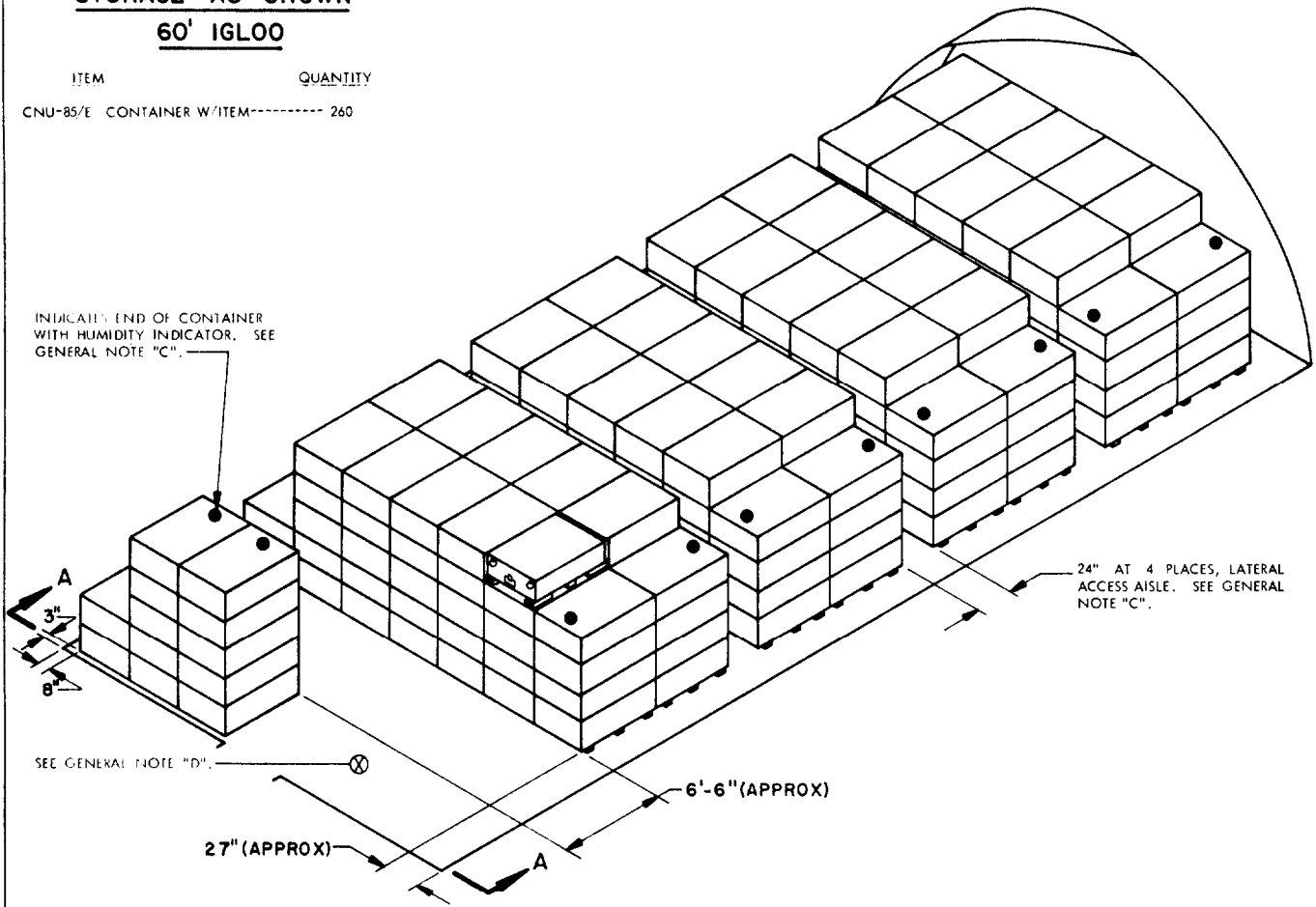
ISOMETRIC VIEW
