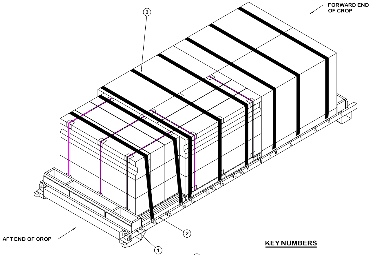
ISOMETRIC VIEW
