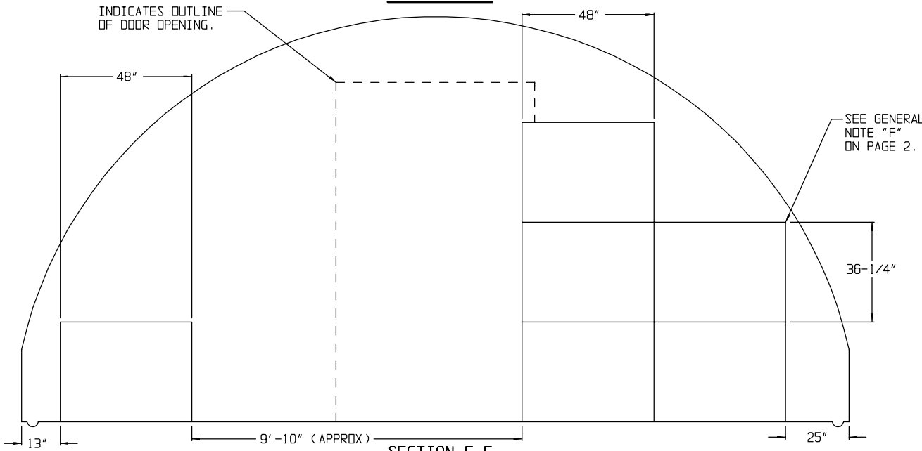
SECTION F-F ( "C" STACK, 6 PALLET UNITS )
