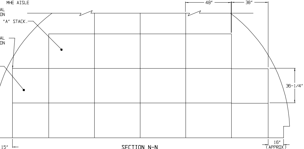
SECTION N-N
