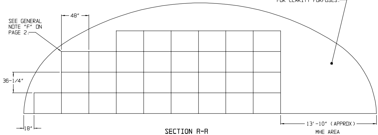
SECTION R-R
