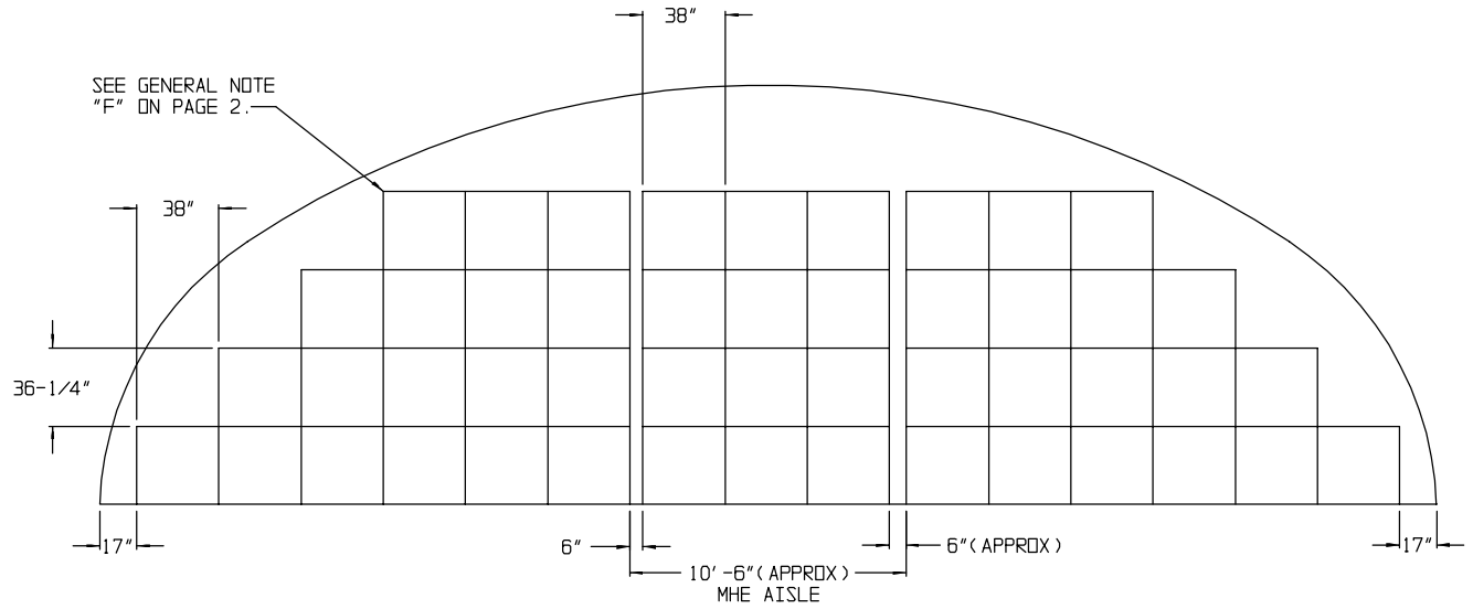
SECTION P-P
