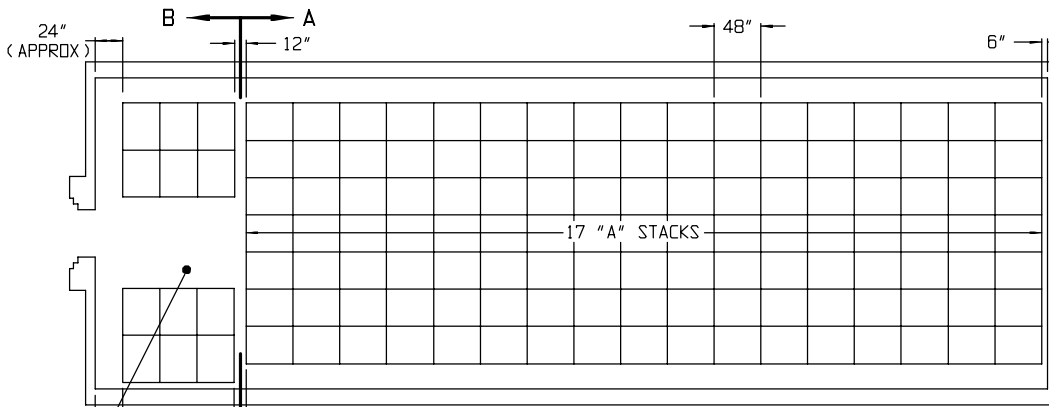
PLAN VIEW (81'-0" IGL00)
