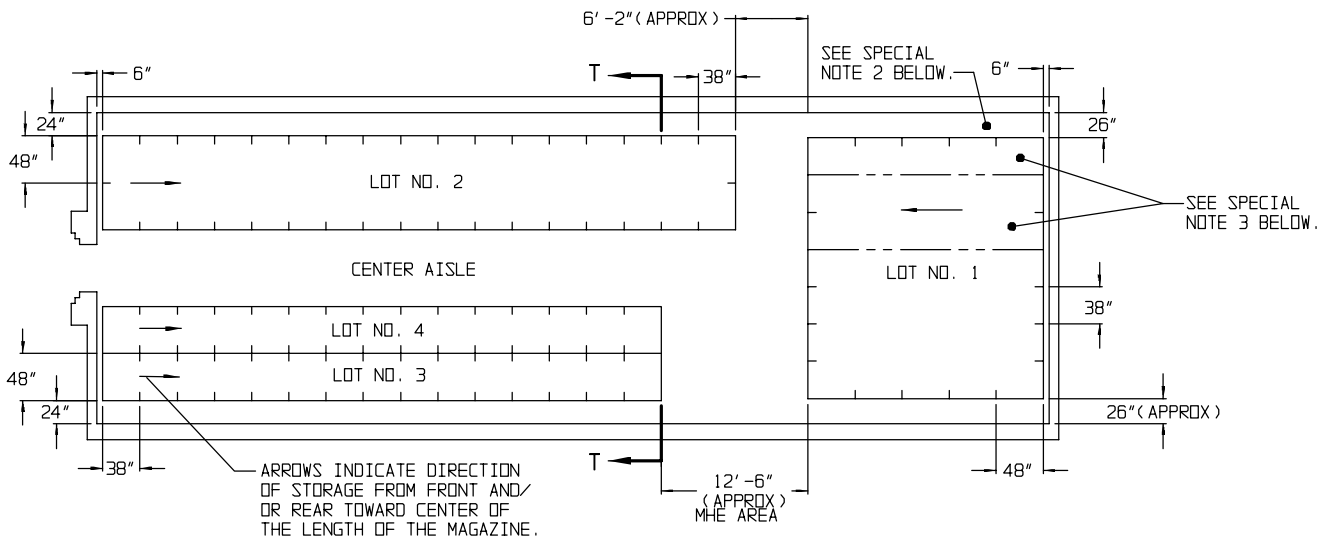
PLAN VIEW (81'-0" IGLOO SHOWN)
