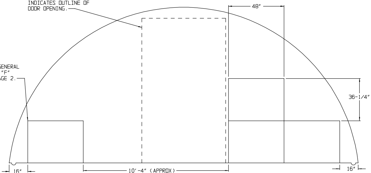
SECTION H-H
