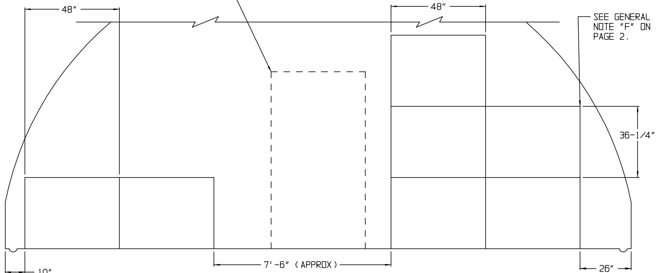
SECTION B-B
