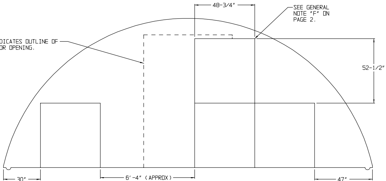
SECTION K-K
