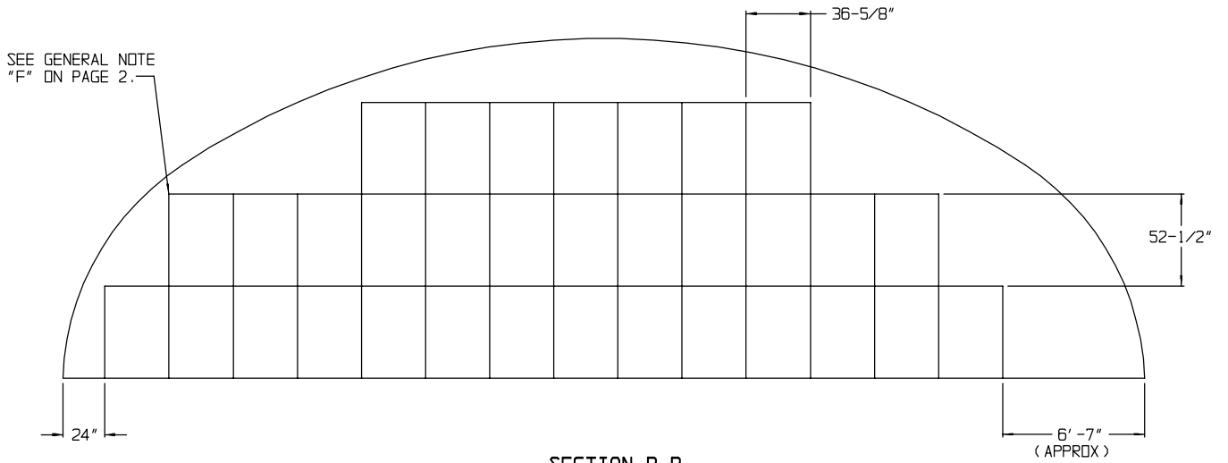
SECTION R-R
