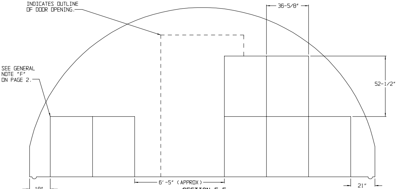
SECTION F-F ( "C" STACK, 7 PALLET UNITS )
