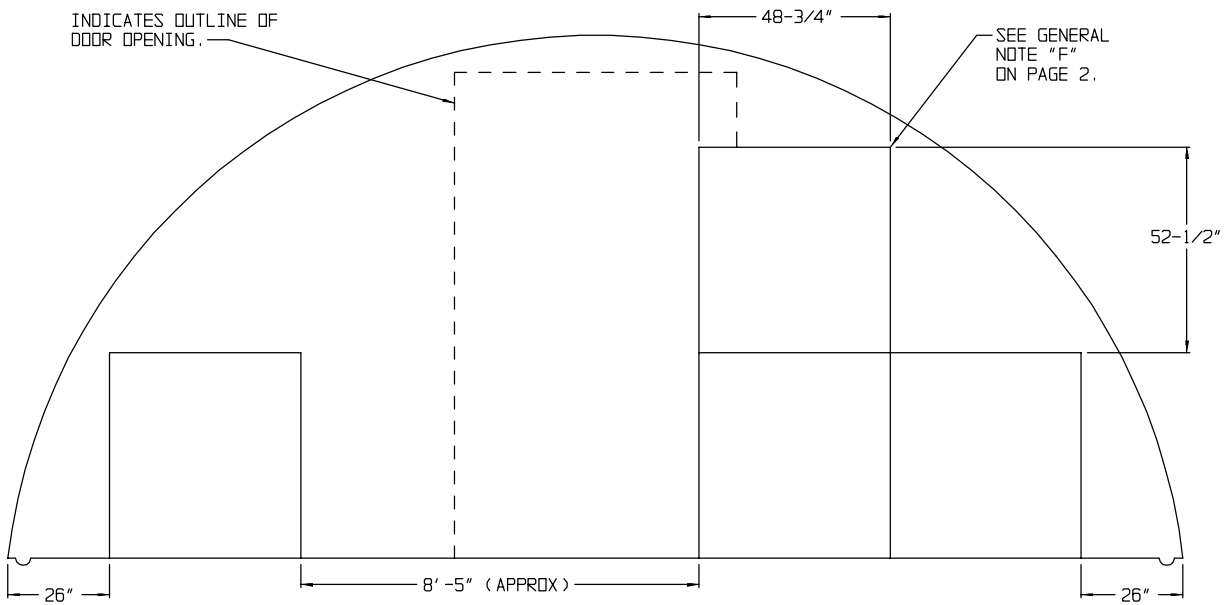
SECTION H-H ( "C" STACK, 4 PALLET UNITS )
