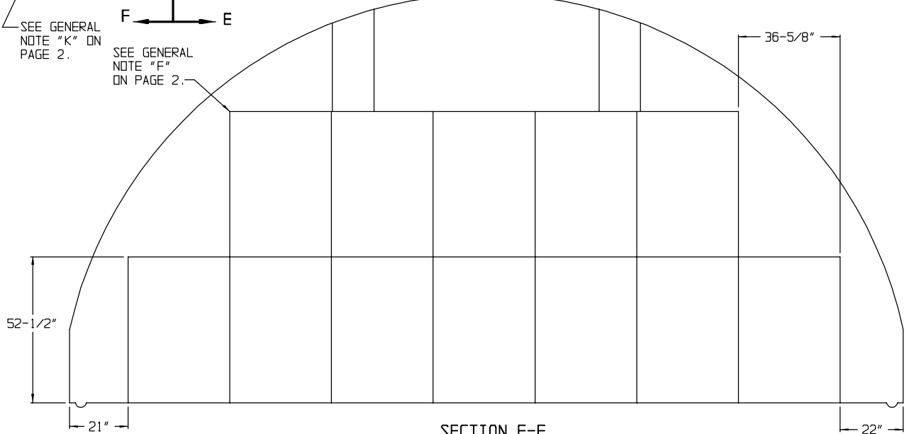
SECTION E-E ( "A" STACK, 12 PALLET UNITS )
