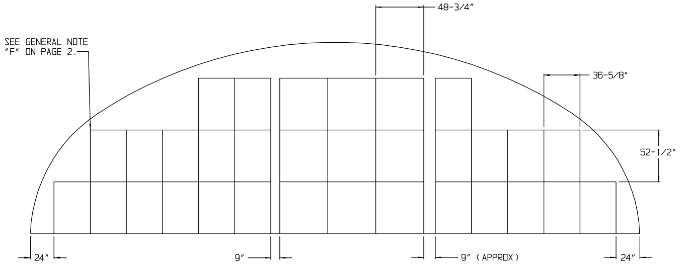
SECTION P-P
