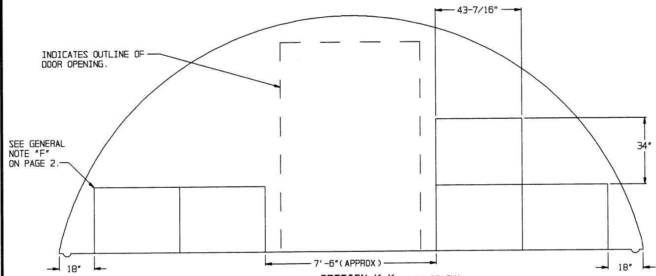
SECTION K-K ("B" STACK)
