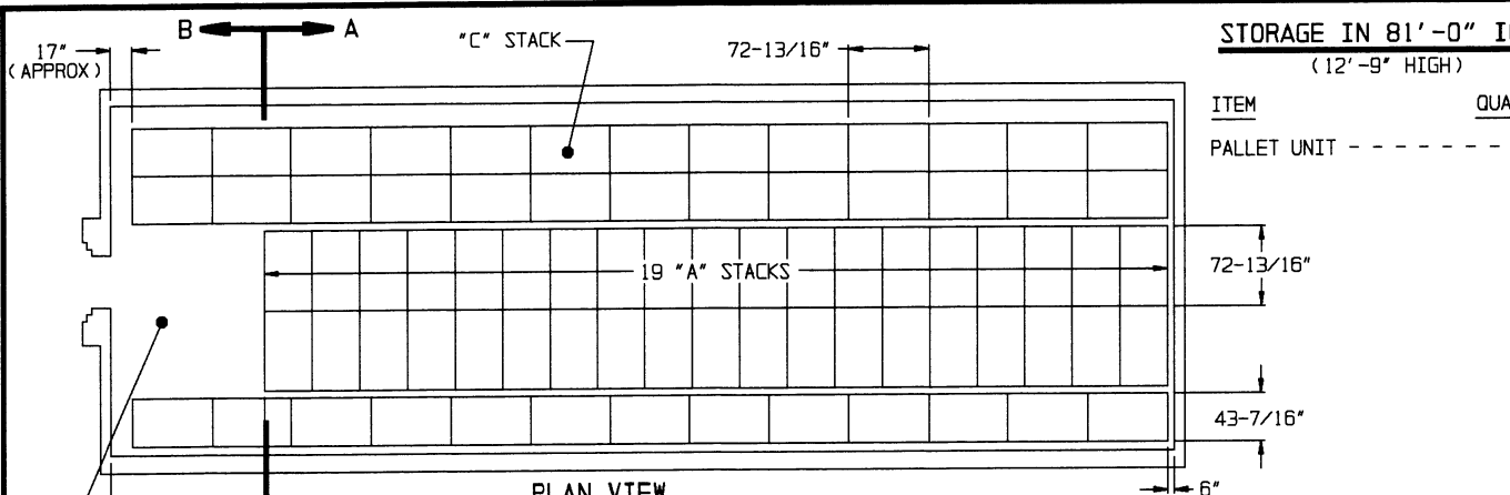
PLAN VIEW (81'-0" IGL00)
