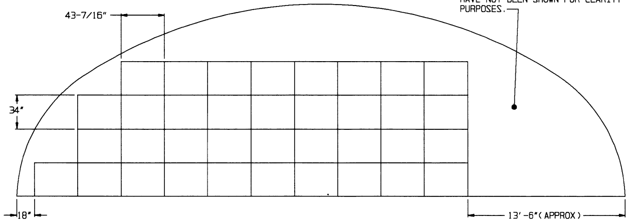
SECTION R-R
