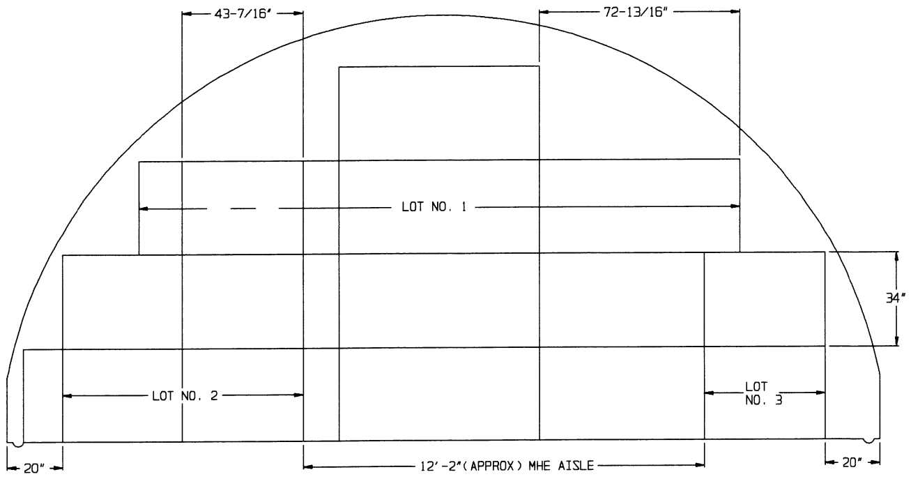
SECTION T-T
