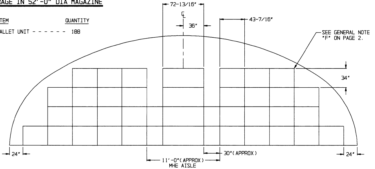
SECTION P-P
