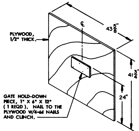
LOAD BEARING GATE C
