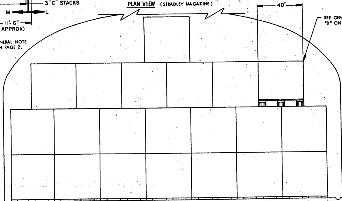
SECTION L-L ("A" STACK, 21 PALLET UNITS)
