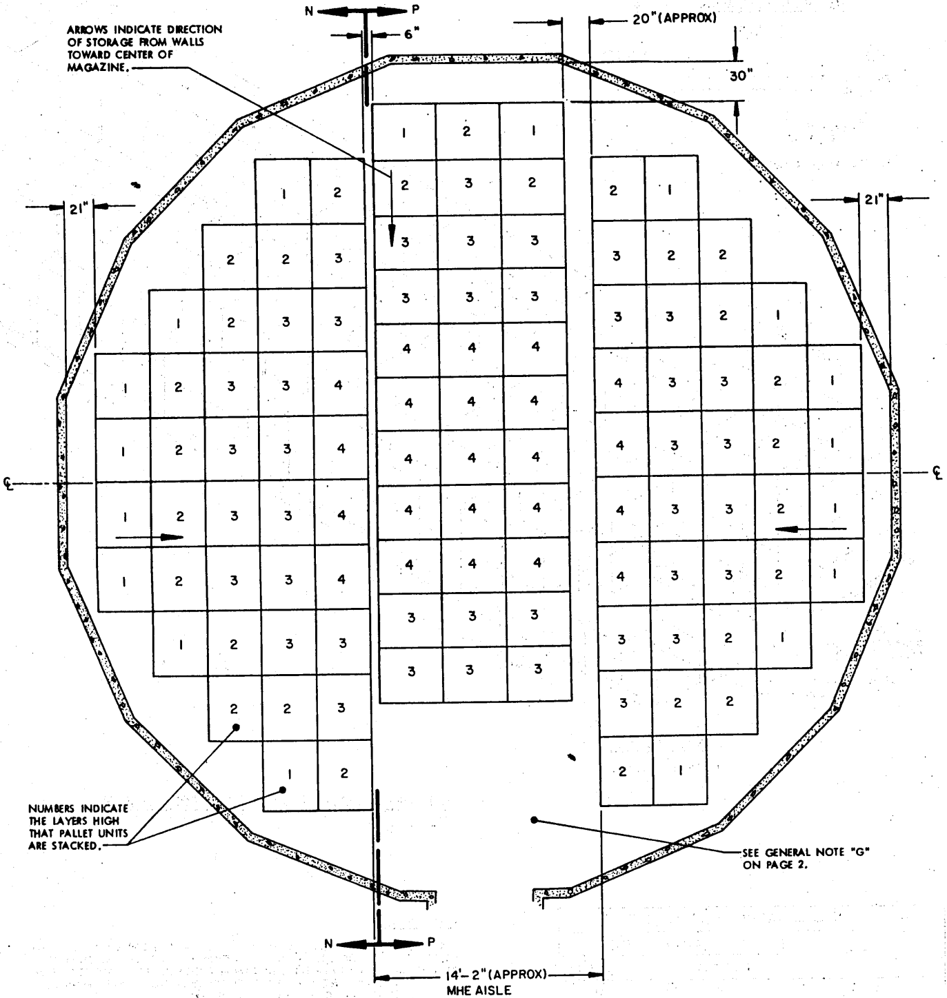
PLAN VIEW (52' DIA MAGAZINE)
