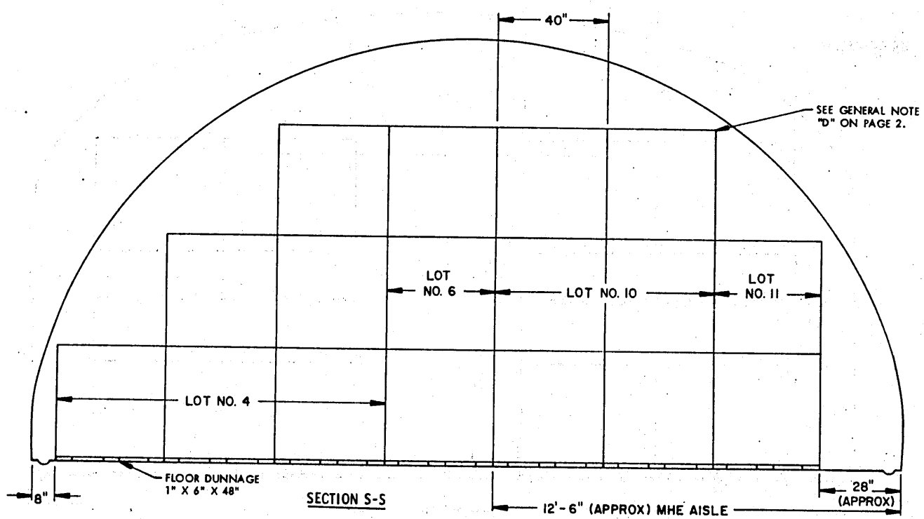
(81' IGLOO MAGAZINE SHOWN)
