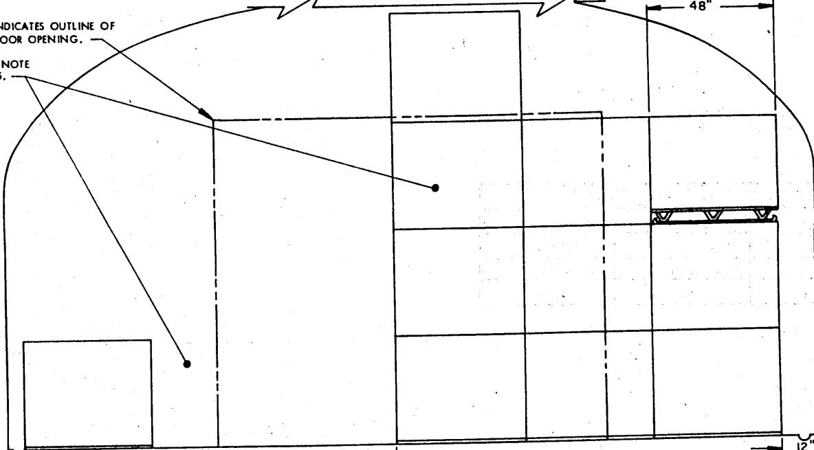
SECTION M-M ("C" STACK, 11 PALLET UNITS)
