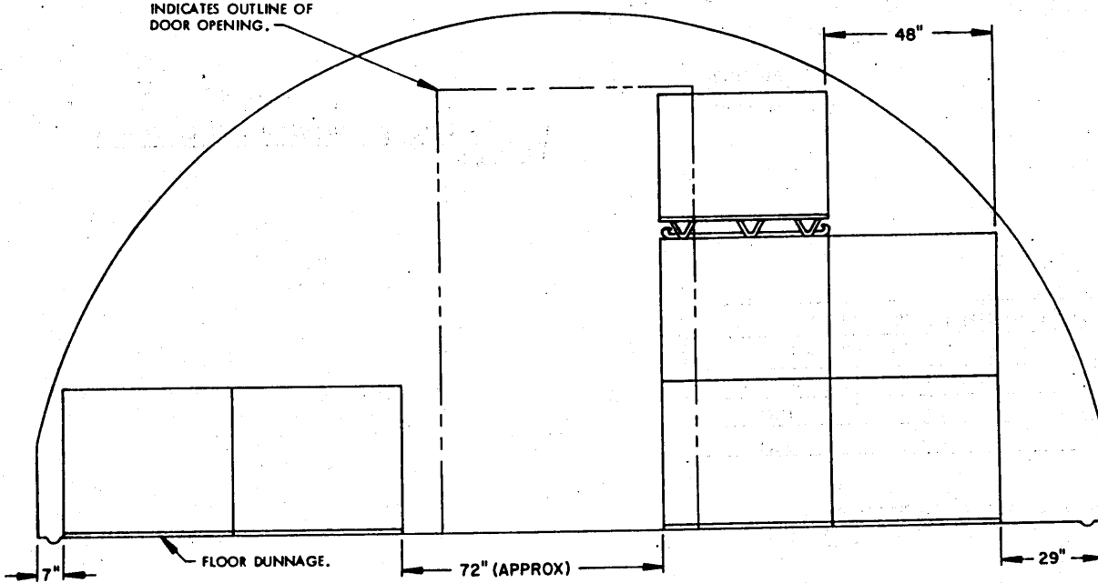
SECTION F-F ("C" STACK, 7 PALLET UNITS)
