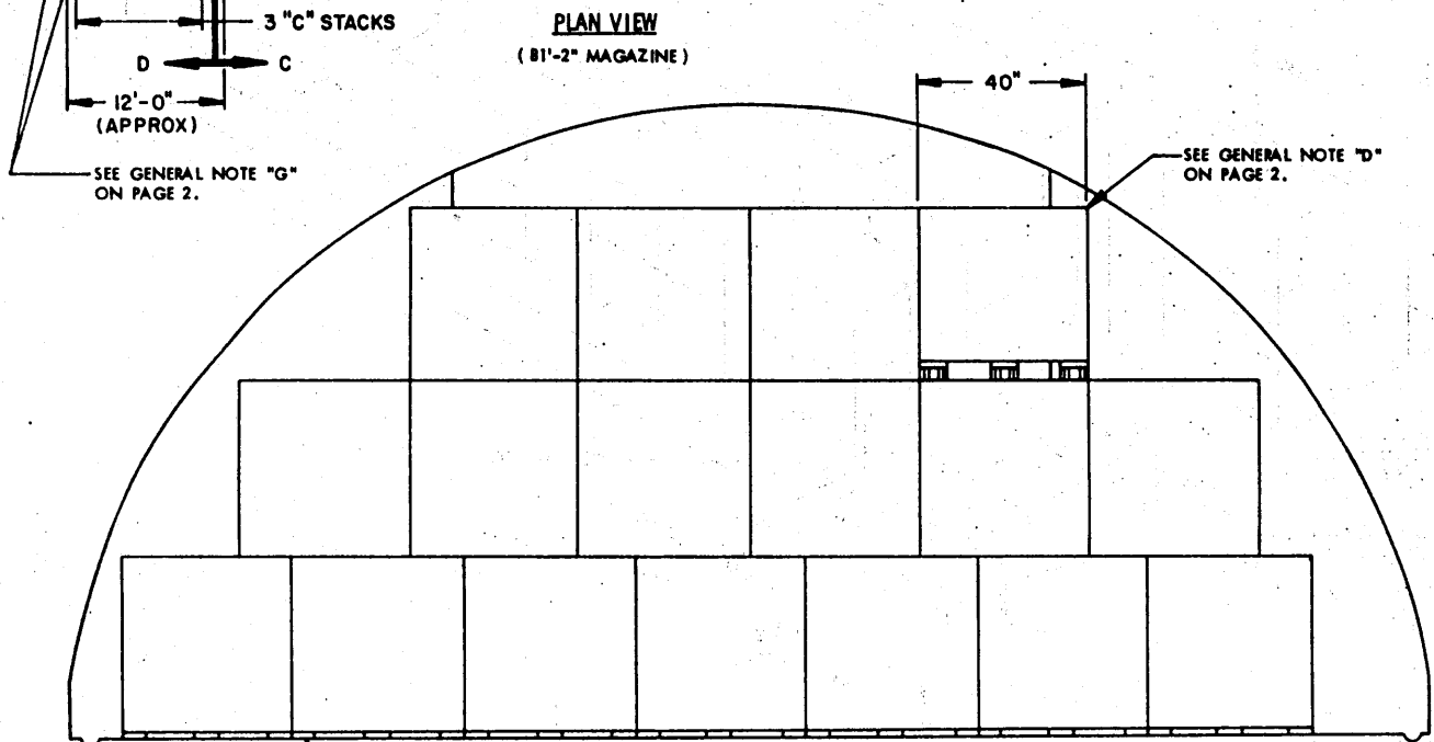
SECTION C-C ( "A" STACK, 17 PALLET UNITS )
