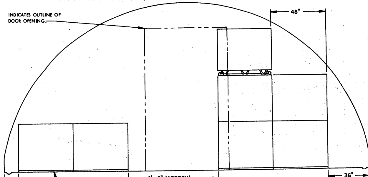
SECTION D-D ( "C" STACK, 7 PALLET UNITS )
