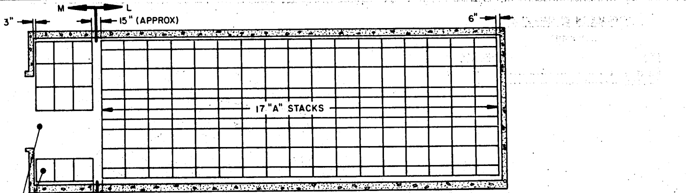
PLAN VIEW (STRADLEY MAGAZINE)
