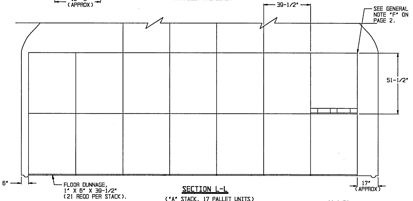
PLAN VIEW (STRADLEY MAGAZINE)
