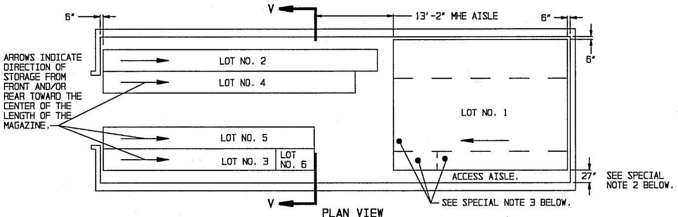
PLAN VIEW (STRADLEY MAGAZINE)
