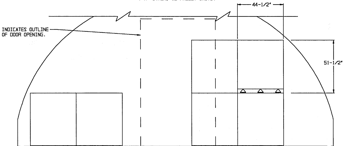
SECTION E-E ( "A" STACK, 12 PALLET UNITS )
