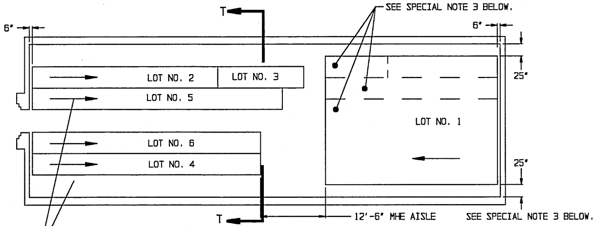
PLAN VIEW (81'-0" IGLOO MAGAZINE SHOWN)
