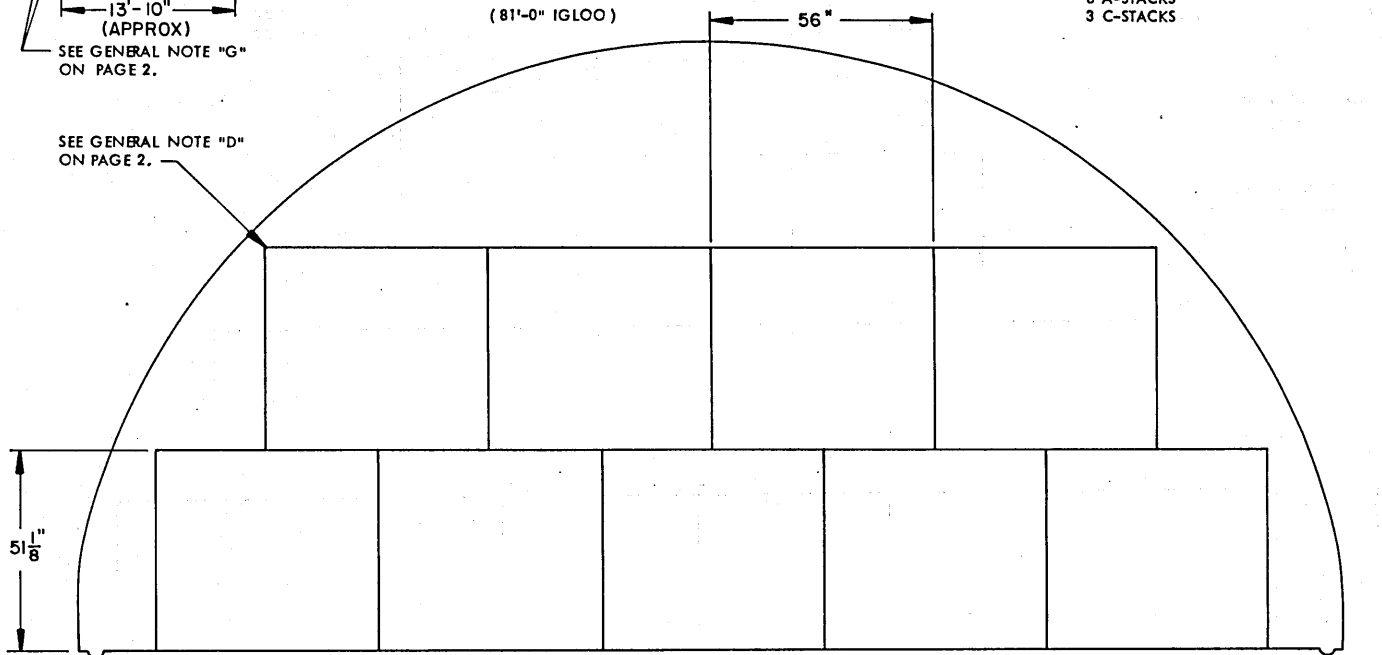
SECTION U7-U7 (*A" STACK, 9 PALLET UNITS)
