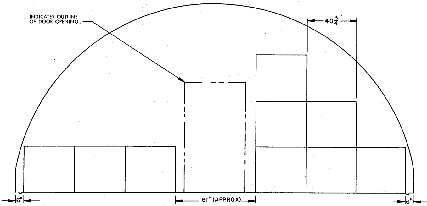
SECTION K6-K6 ( "C" STACK, 9 PALLET UNITS )
