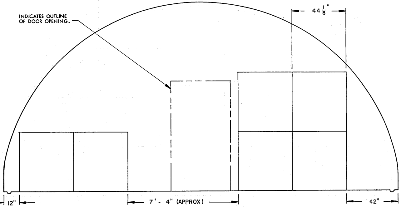
SECTION B4-B4 ( "C" STACK, 6 PALLET UNITS ) STORAGE PROCEDURES FOR UNIT NO. 41
