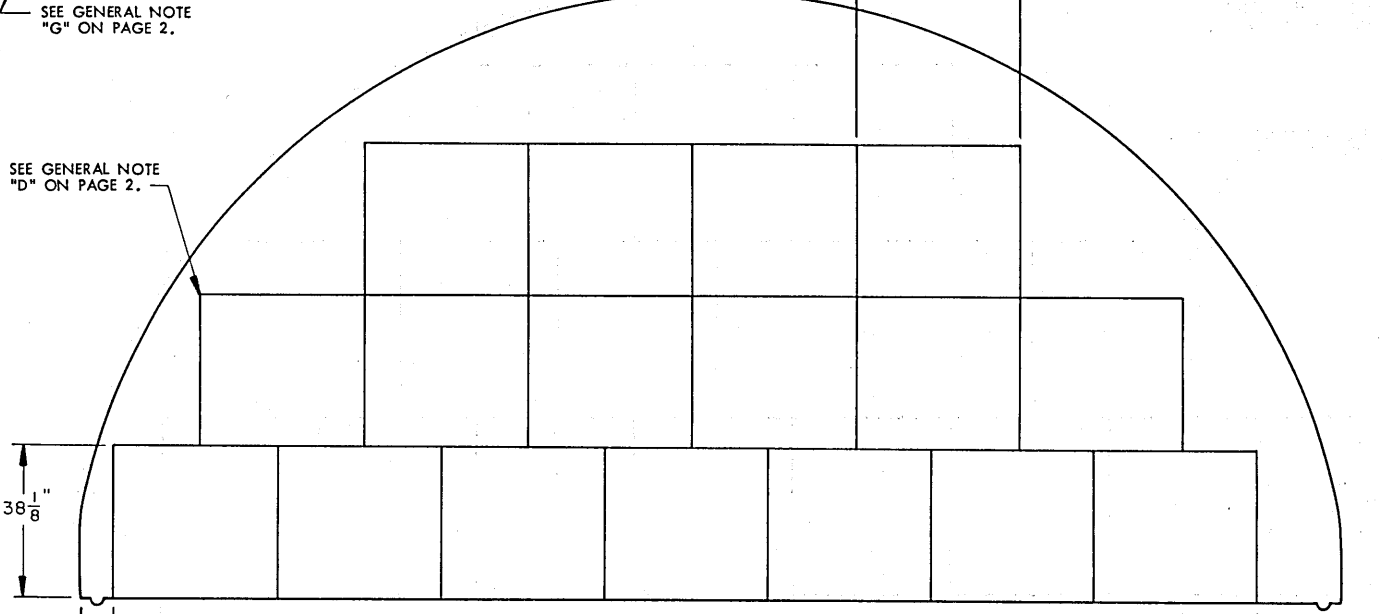
SECTION Z2-Z2 ( "A" STACK, 17 PALLET UNITS )
