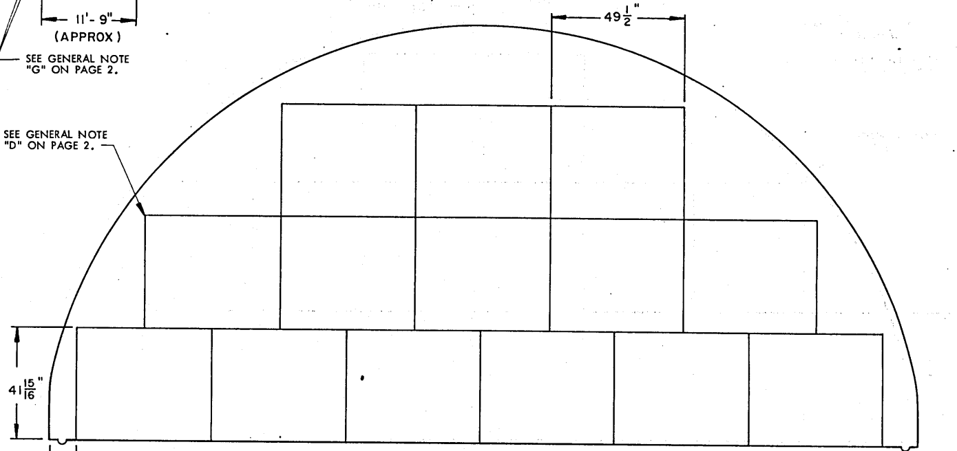
SECTION H3-H3 ("A" STACK, 14 PALLET UNITS)
