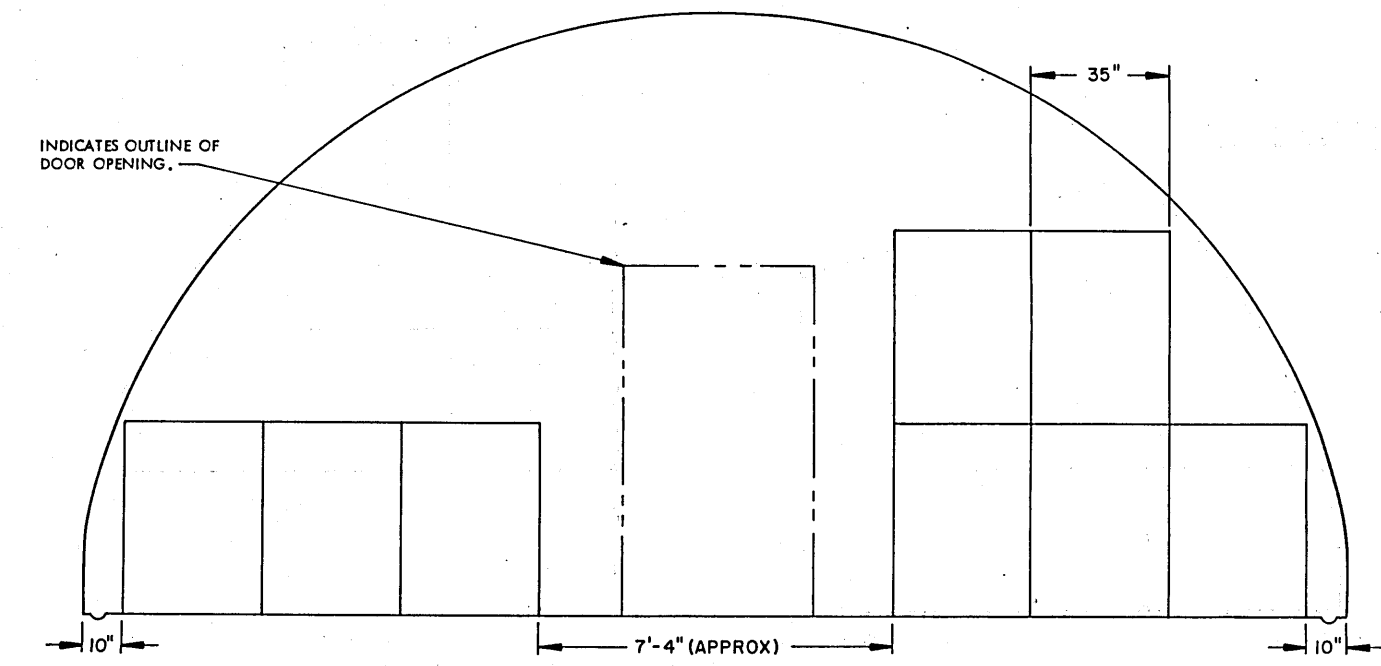
SECTION Q8-Q8 ("C" STACK, 8 PALLET UNITS)
