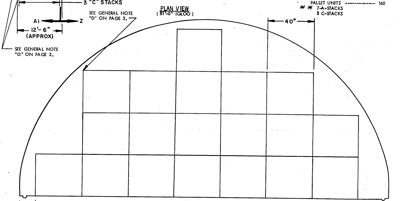
PLAN VIEW (81'-0" IGLOO) SECTION Z-Z ("A" STACK, 19 PALLET UNITS) SECTION A1-A1 ("C" STACK, 9 PALLET UNITS)
