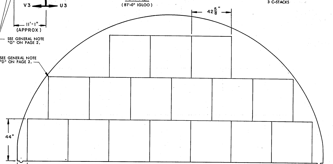
SECTION U3-U3 ( "A" STACK, 16 PALLET UNITS )
