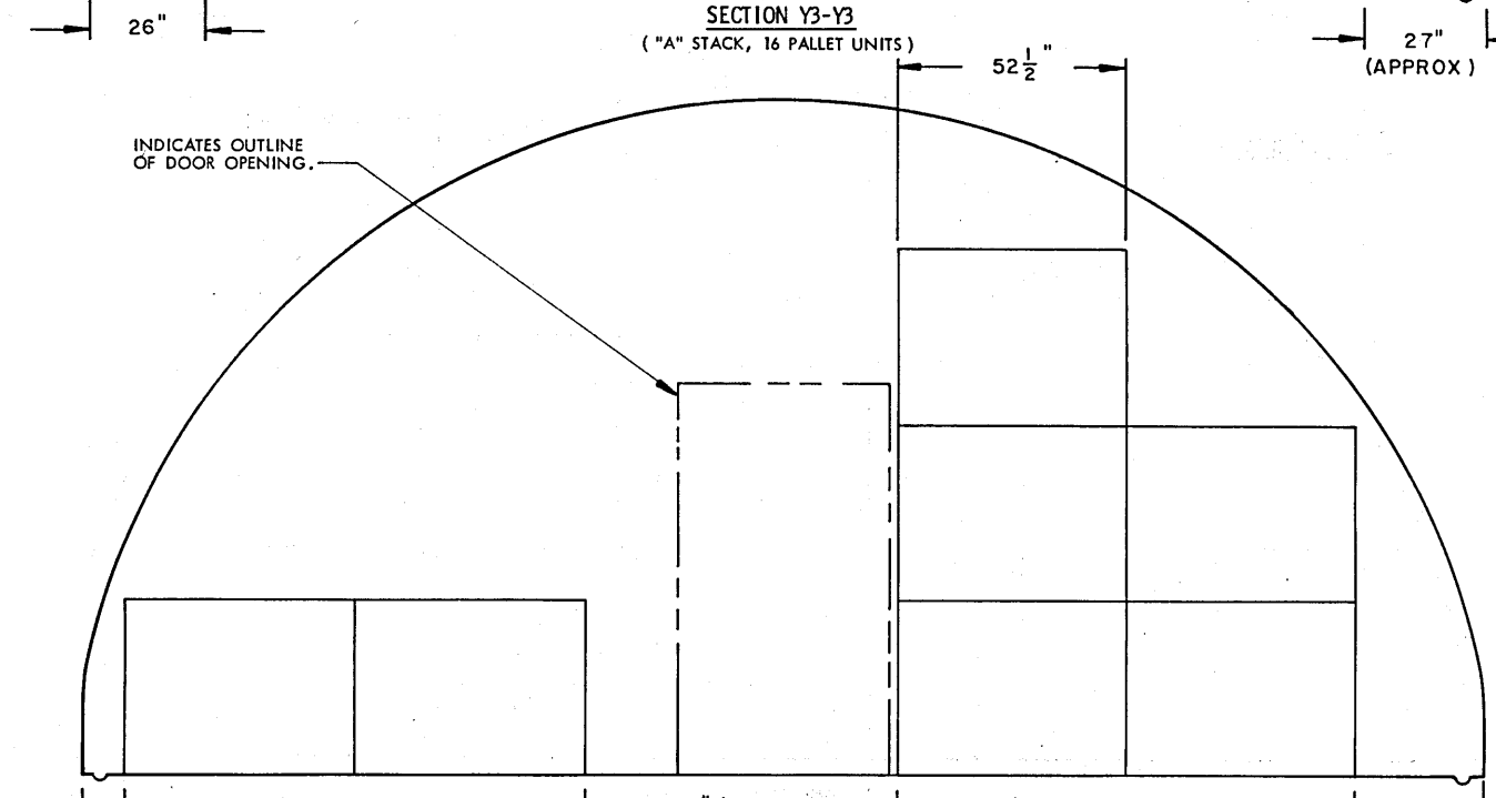
SECTION Z3-Z3 ( "C" STACK, 7 PALLET UNITS )
