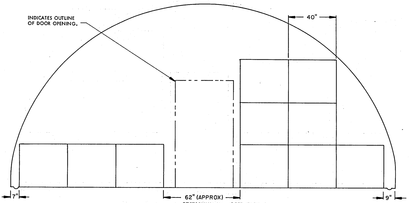
SECTION U4-U4 ( "C" STACK, 10 PALLET UNITS )
