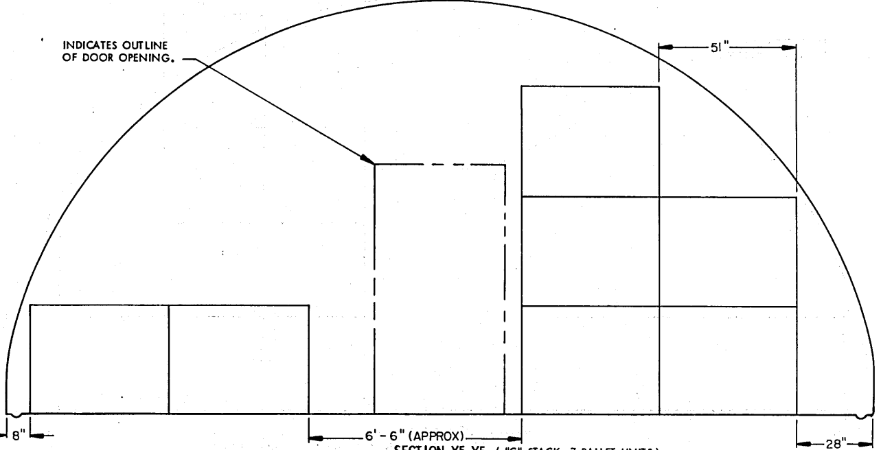
SECTION X5-X5 ( "C" STACK, 7 PALLET UNITS )
