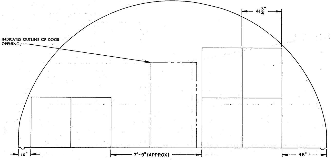
SECTION M8-M8 ( "C" STACK, 6 PALLET UNITS )
