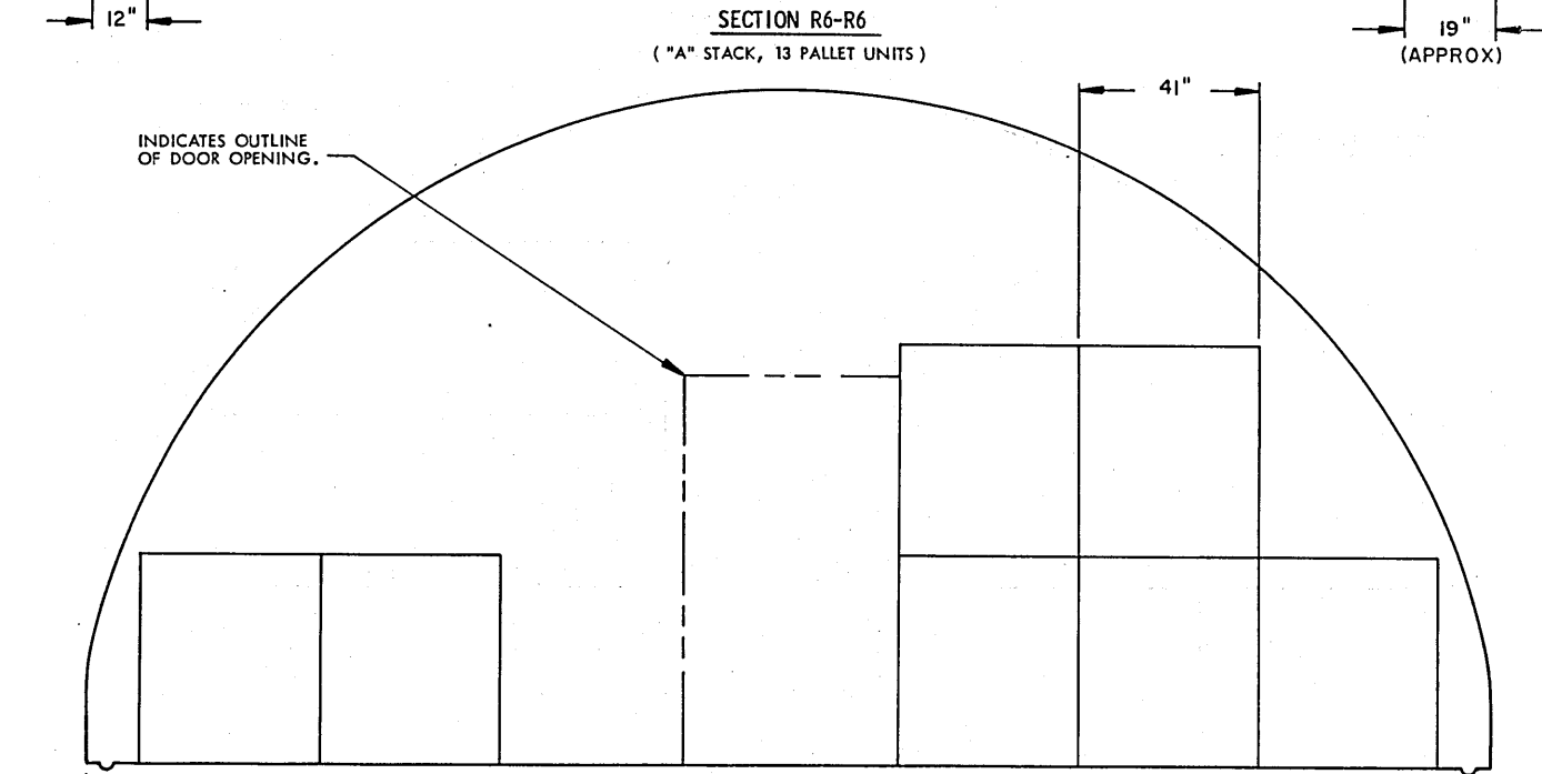
SECTION S6-S6 ( "C" STACK, 7 PALLET UNITS ) STORAGE PROCEDURES FOR UNIT NO. 57 ( INCREASED-HEIGHT UNIT )
