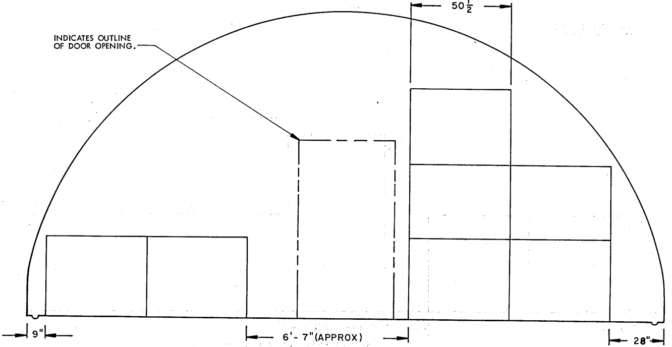
SECTION D4-D4 ("C" STACK, 7 PALLET UNITS) STORAGE PROCEDURES FOR UNIT NO. 41 (DECREASED-HEIGHT UNIT)
