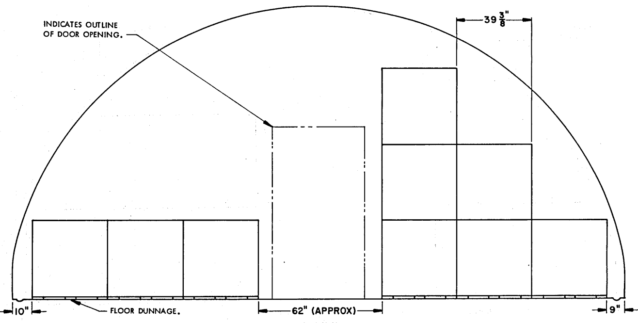
SECTION U-U ( "C" STACK, 9 PALLET UNITS) STORAGE PROCEDURES FOR UNIT NO. 10
