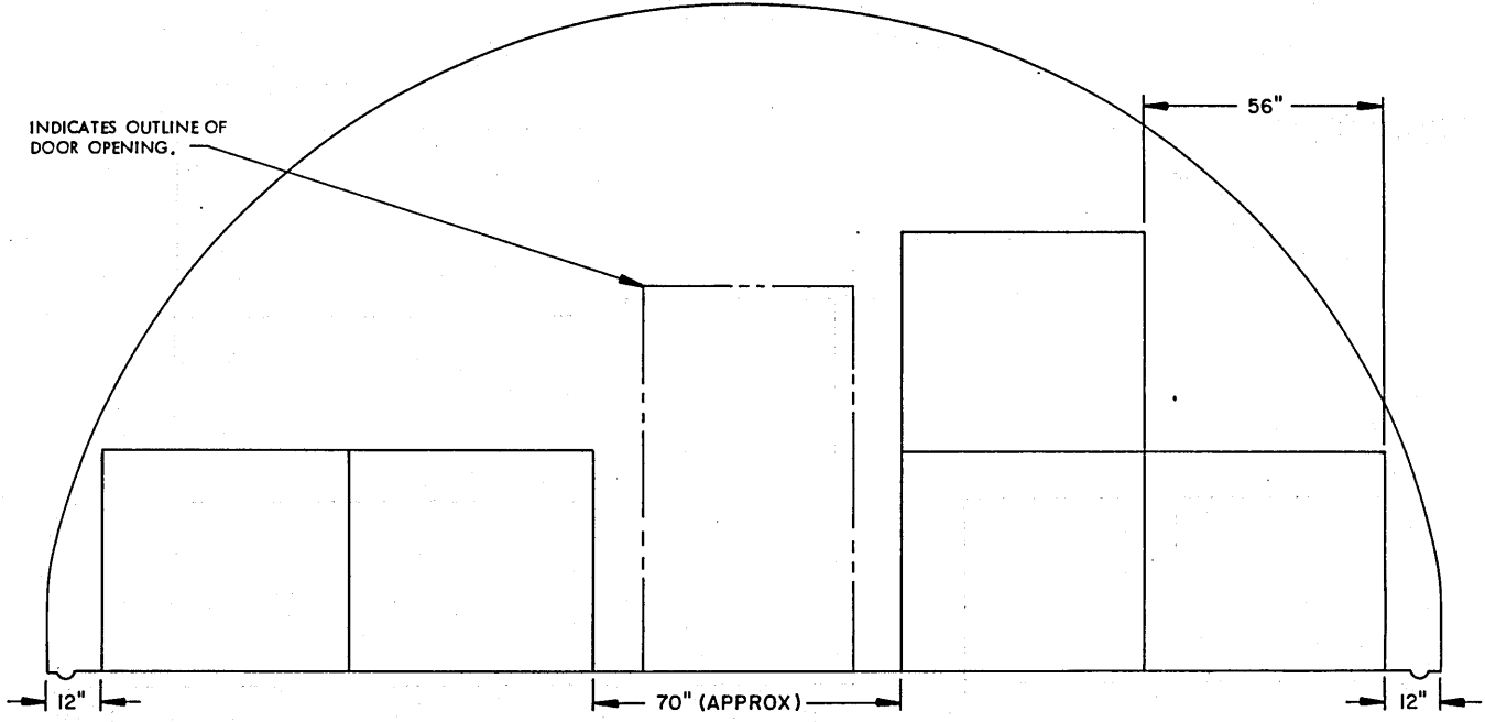
SECTION V7-V7 ("C" STACK, 5 PALLET UNITS)
