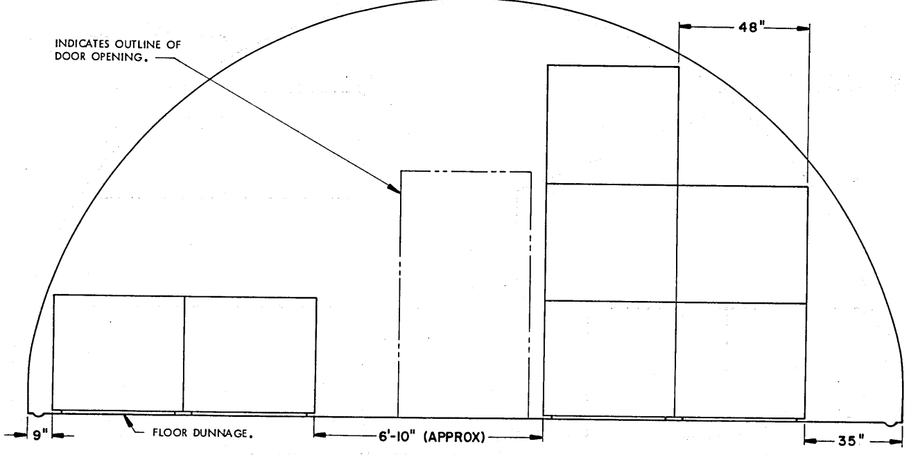
SECTION O-O ( "C" STACK, 7 PALLET UNITS ) STORAGE PROCEDURES FOR UNIT NO. 7
