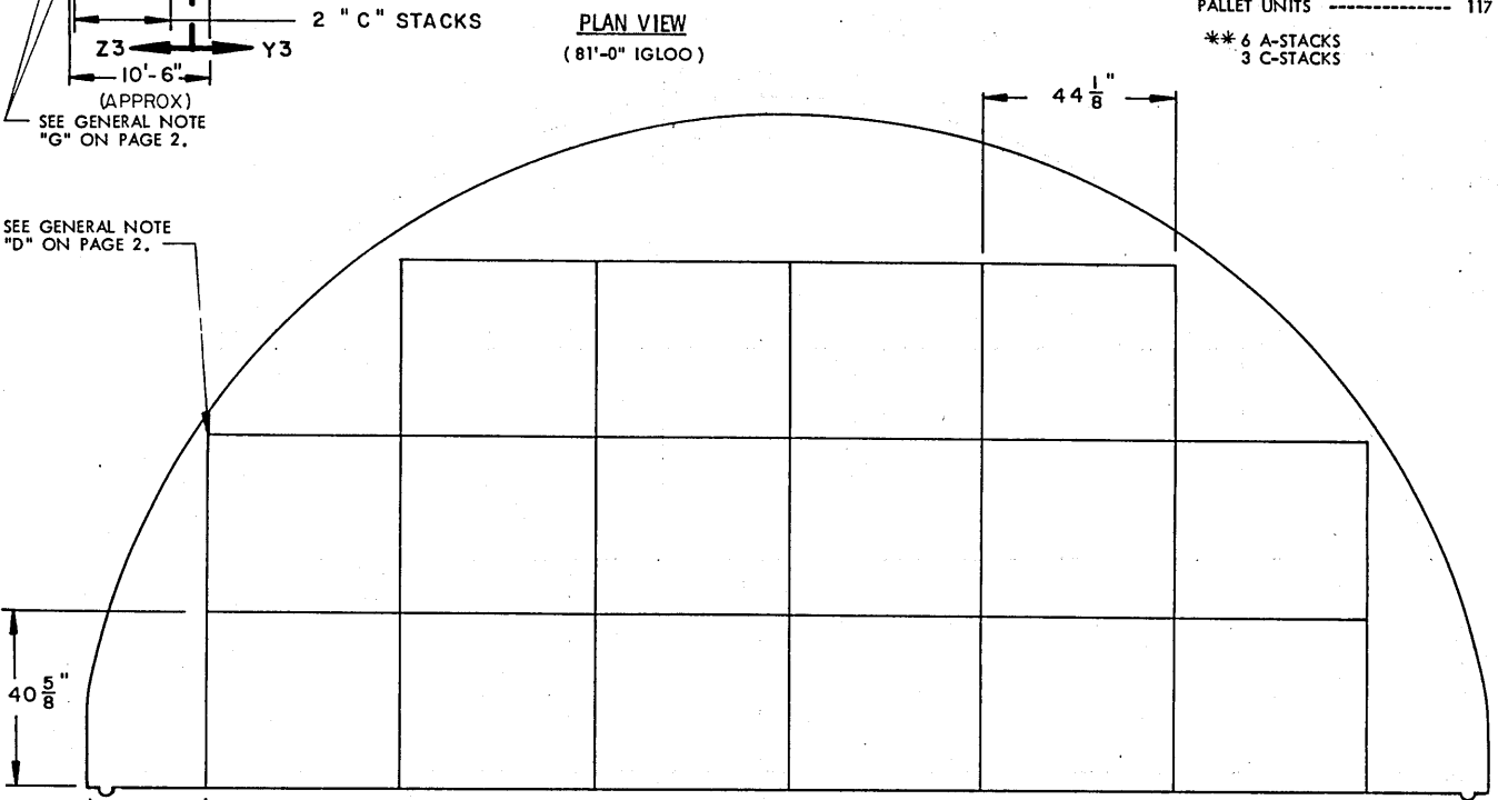
SECTION Y3-Y3 ( "A" STACK, 16 PALLET UNITS )
