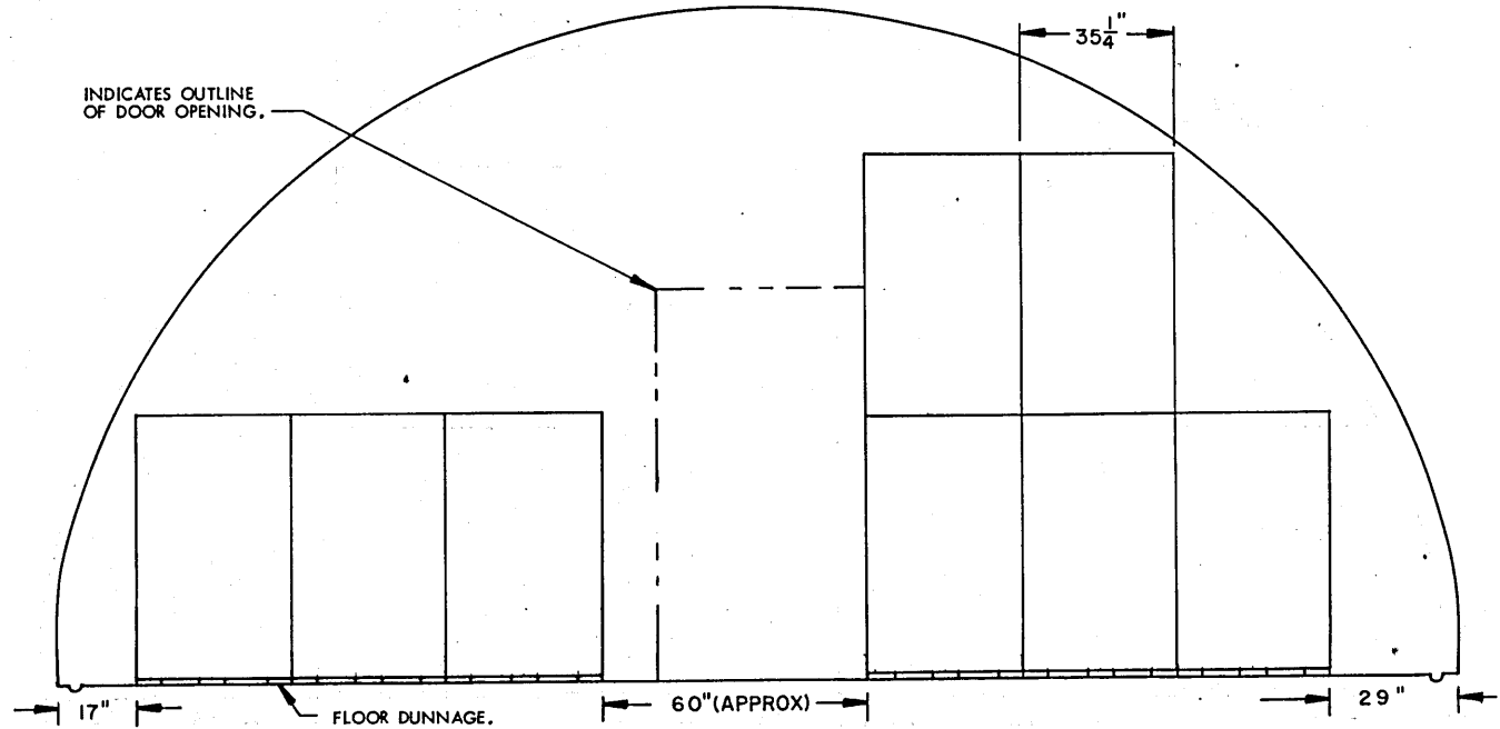
SECTION T1-T1 (* "C" STACK, 8 PALLET UNITS) STORAGE PROCEDURES FOR UNIT NO. 22
