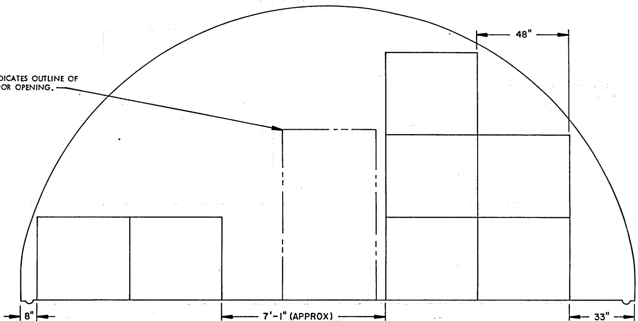
SECTION F8-F8 ( "C" STACK, 7 PALLET UNITS )
