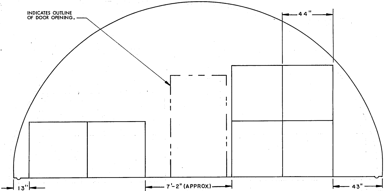
SECTION F4-F4 ( "C" STACK, 6 PALLET UNITS )
