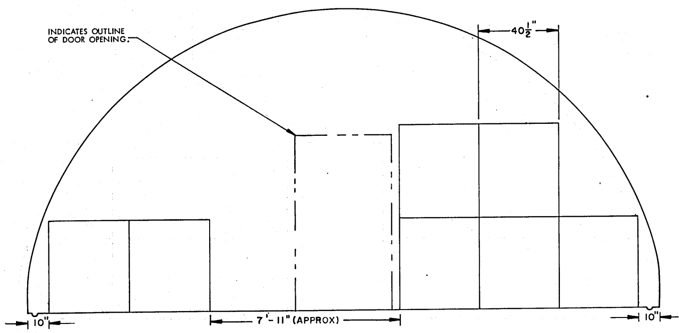
SECTION P3-P3 ( "C" STACK, 7 PALLET UNITS )
