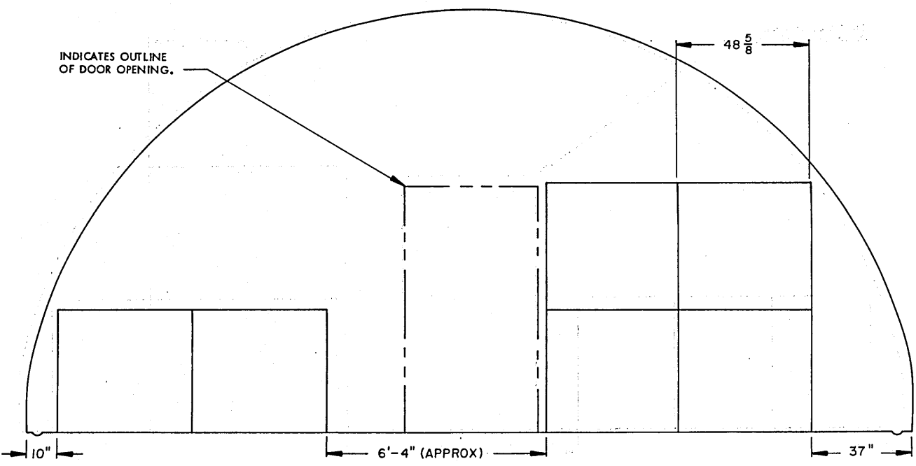
SECTION C7-C7 ( "C" STACK, 6 PALLET UNITS)
