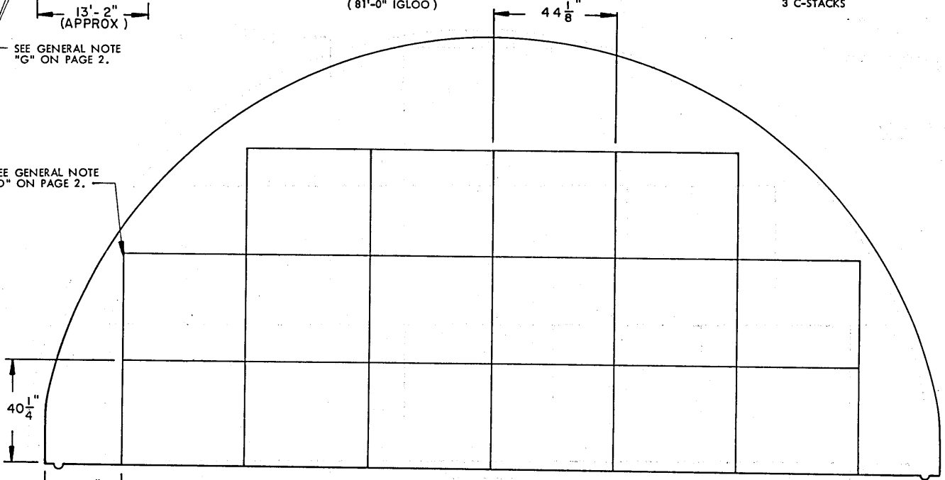
SECTION C4-C4 ("A" STACK, 16 PALLET UNITS)
