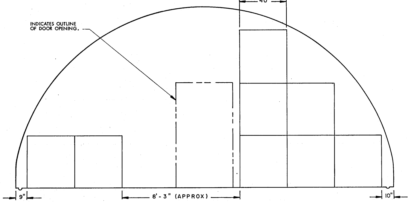
SECTION C3-C3 ( "C" STACK, 8 PALLET UNITS ) STORAGE PROCEDURES FOR UNIT NO. 35
