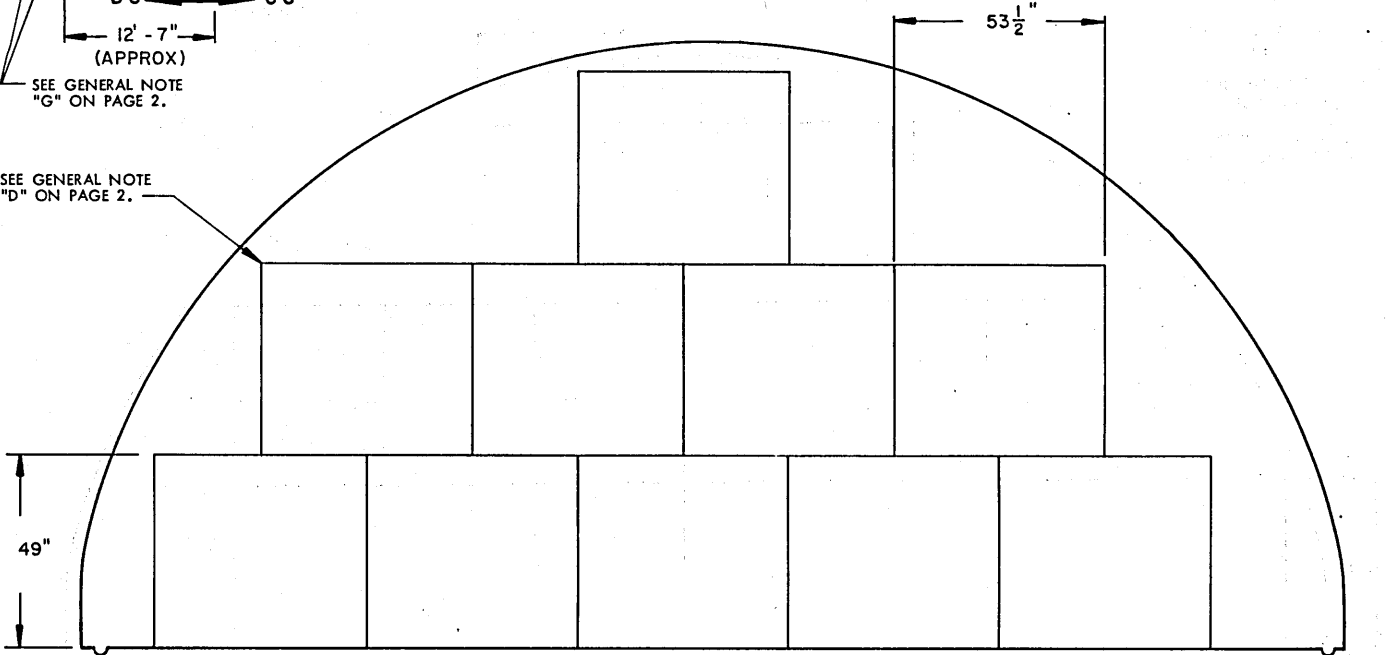
SECTION C6-C6 (*A" STACK, 10 PALLET UNITS)
