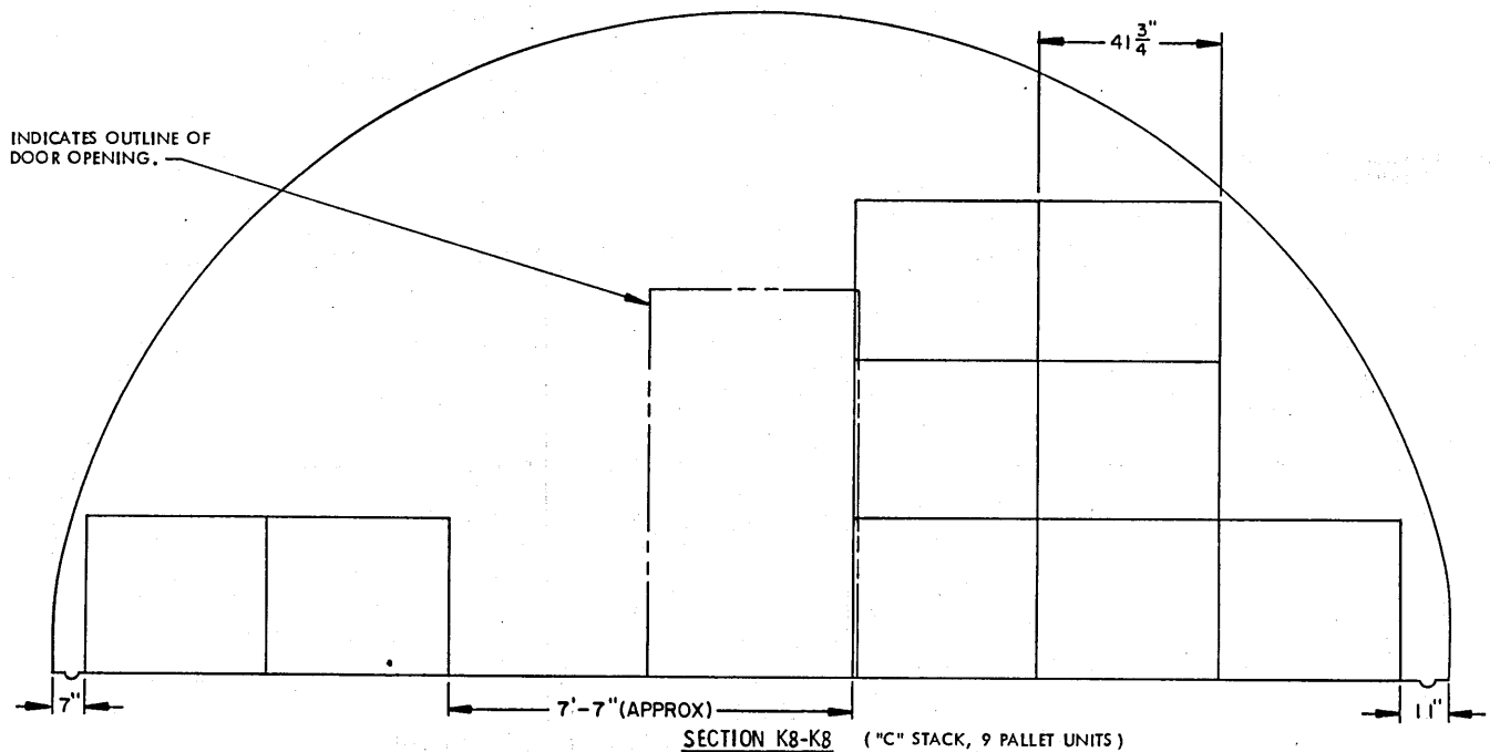
SECTION K8-K8 ("C" STACK, 9 PALLET UNITS)
