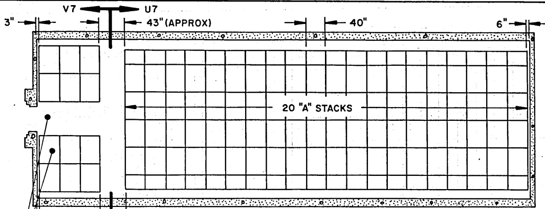
PLAN VIEW (81'-0" IGLOO)
