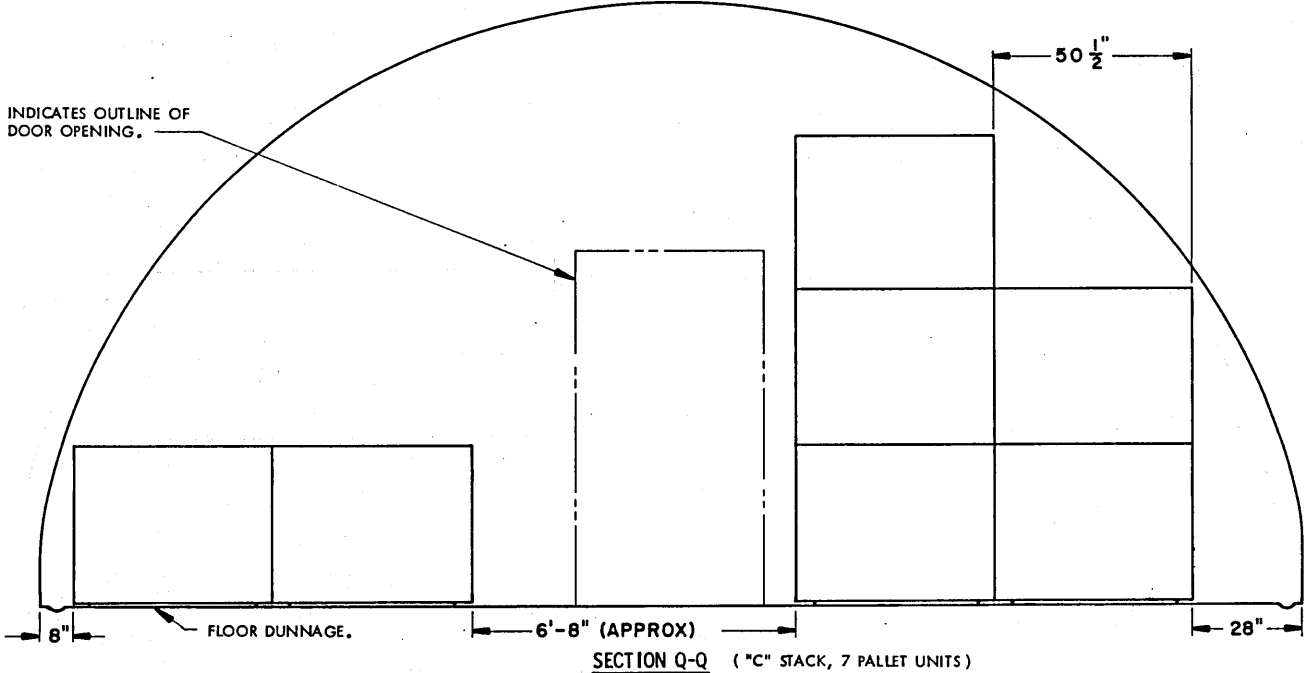
SECTION Q-Q ( "C" STACK, 7 PALLET UNITS )
