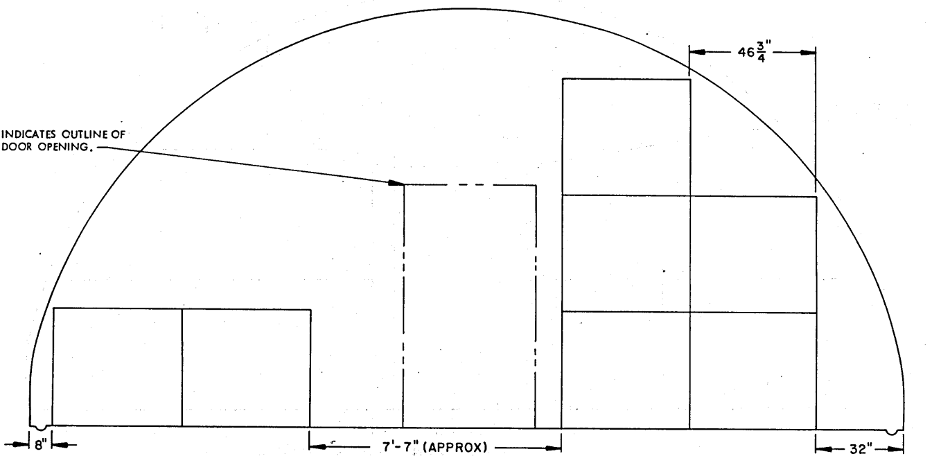
SECTION X7-X7 ("C" STACK, 7 PALLET UNITS)
