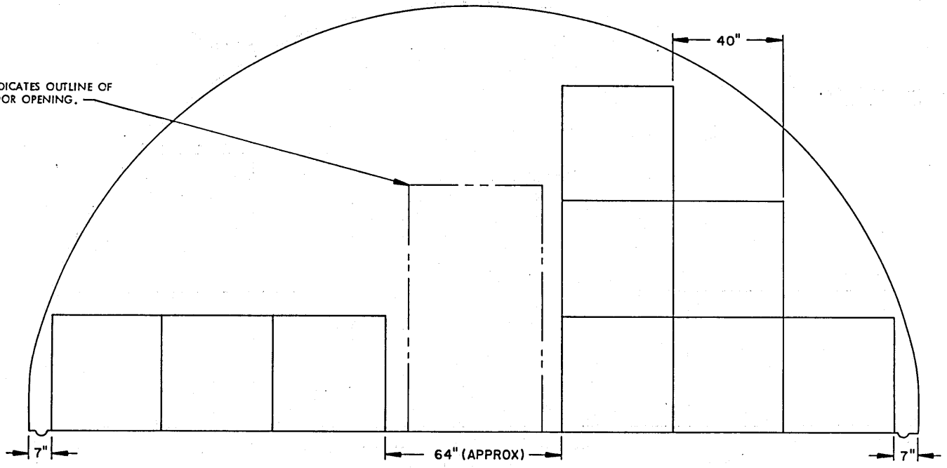
SECTION T7-T7 ( "C" STACK, 9 PALLET UNITS )
