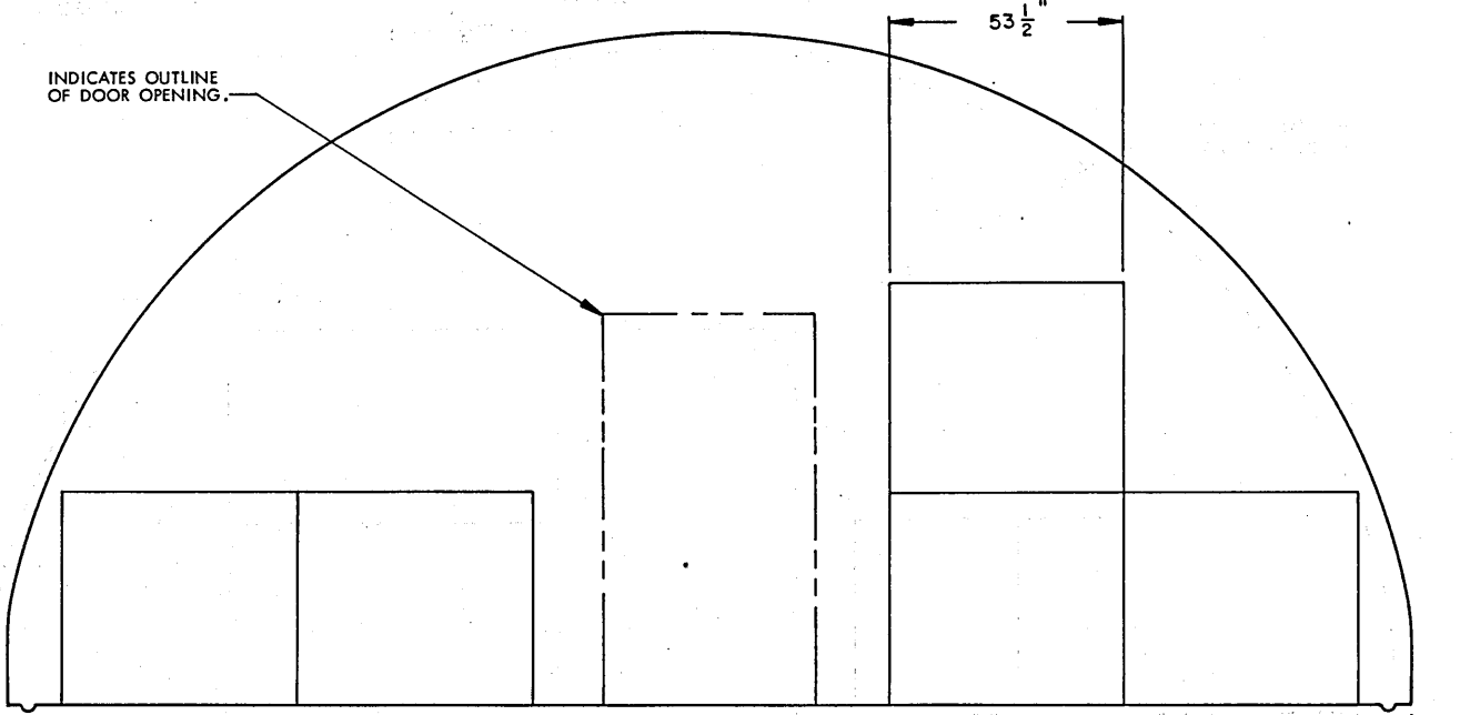
SECTION D6-D6 (*C" STACK, 5 PALLET UNITS) STORAGE PROCEDURES FOR UNIT NO. 54
