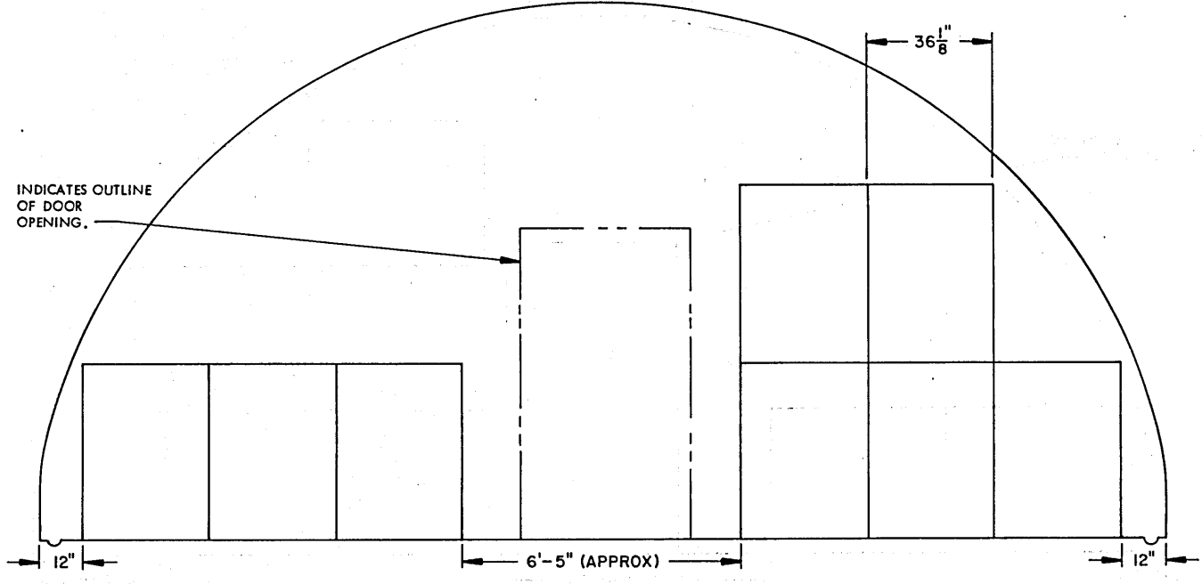
SECTION H8-H8 ( "C" STACK, 8 PALLET UNITS )
