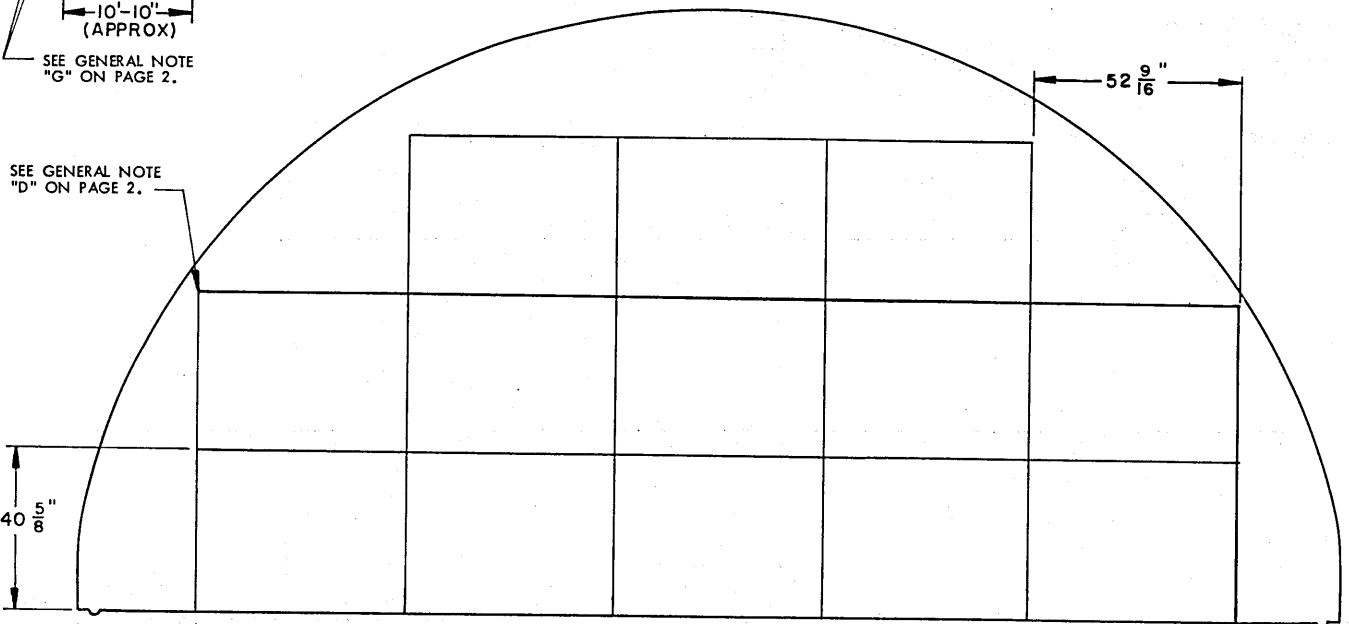
SECTION G4-G4 ( "A" STACK, 13 PALLET UNITS )
