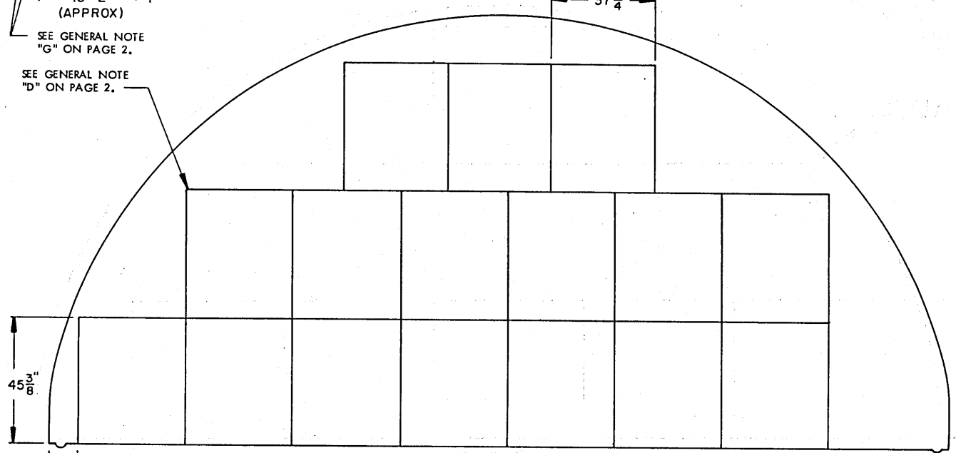
SECTION A6-A6 ( "A" STACK, 16 PALLET UNITS )
