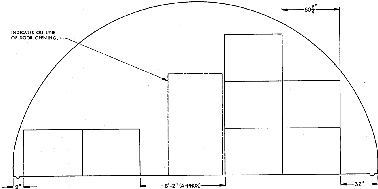
SECTION D-D ( "C" STACK, 7 PALLET UNITS ) STORAGE PROCEDURES FOR UNIT NO. 2
