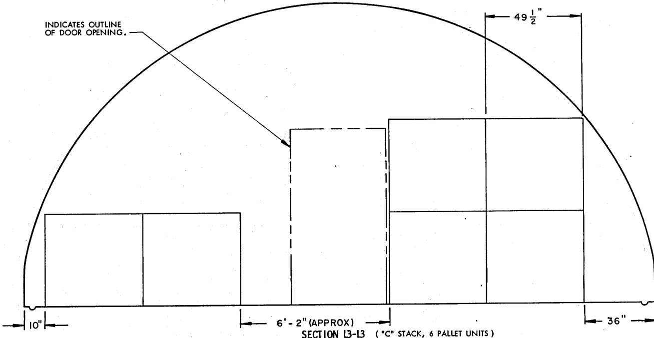
SECTION L3-L3 ( "C" STACK, 6 PALLET UNITS ) STORAGE PROCEDURES FOR UNIT NO. 37
