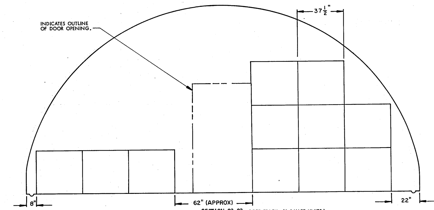
SECTION G3-G3 ( "C" STACK, 11 PALLET UNITS ) STORAGE PROCEDURES FOR UNIT NO. 36
