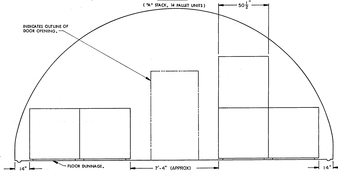
SECTION M-M ( "C" STACK, 5 PALLET UNITS )
