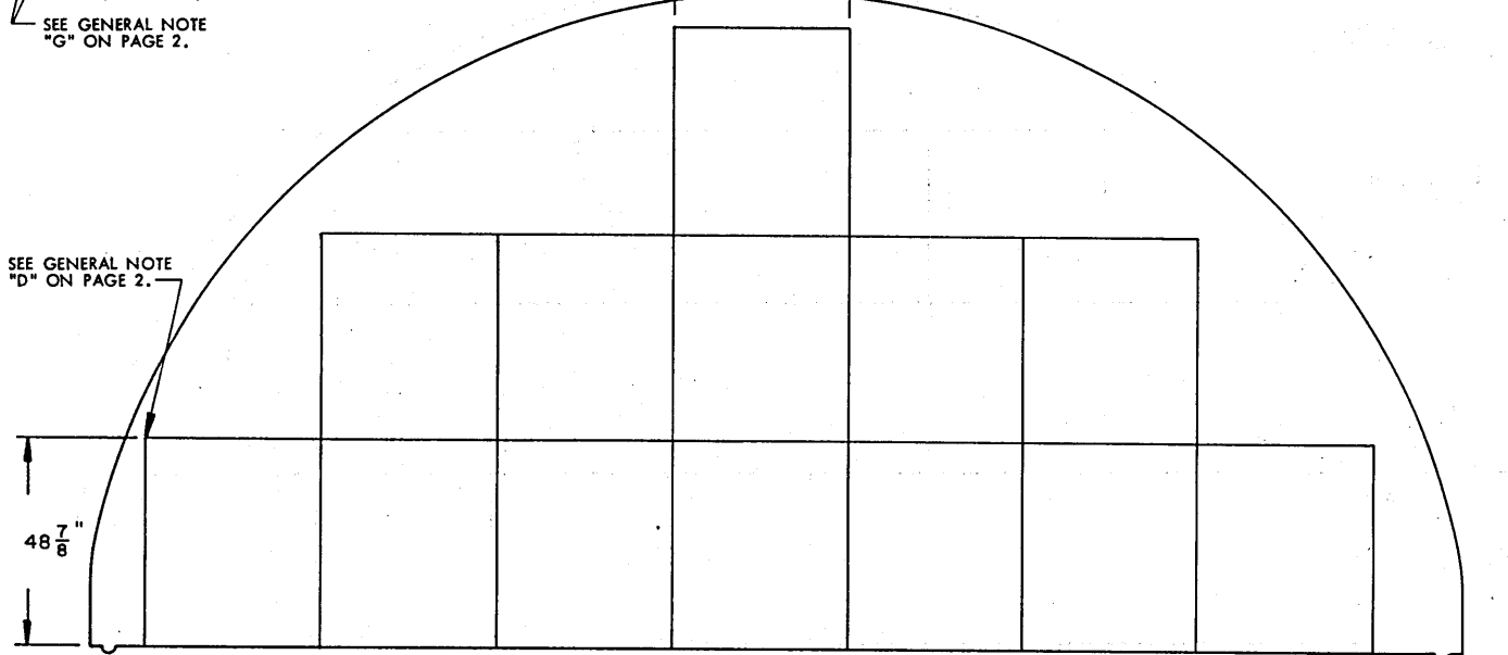
SECTION R6-R6 ( "A" STACK, 13 PALLET UNITS )
