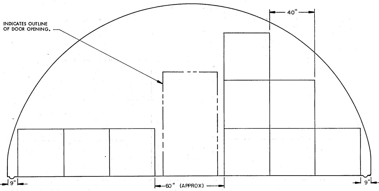
SECTION W4-W4 ("C" STACK, 9 PALLET UNITS)
