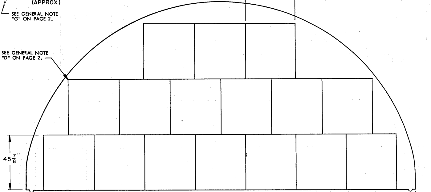
SECTION X2-X2 ( "A" STACK, 16 PALLET UNITS )
