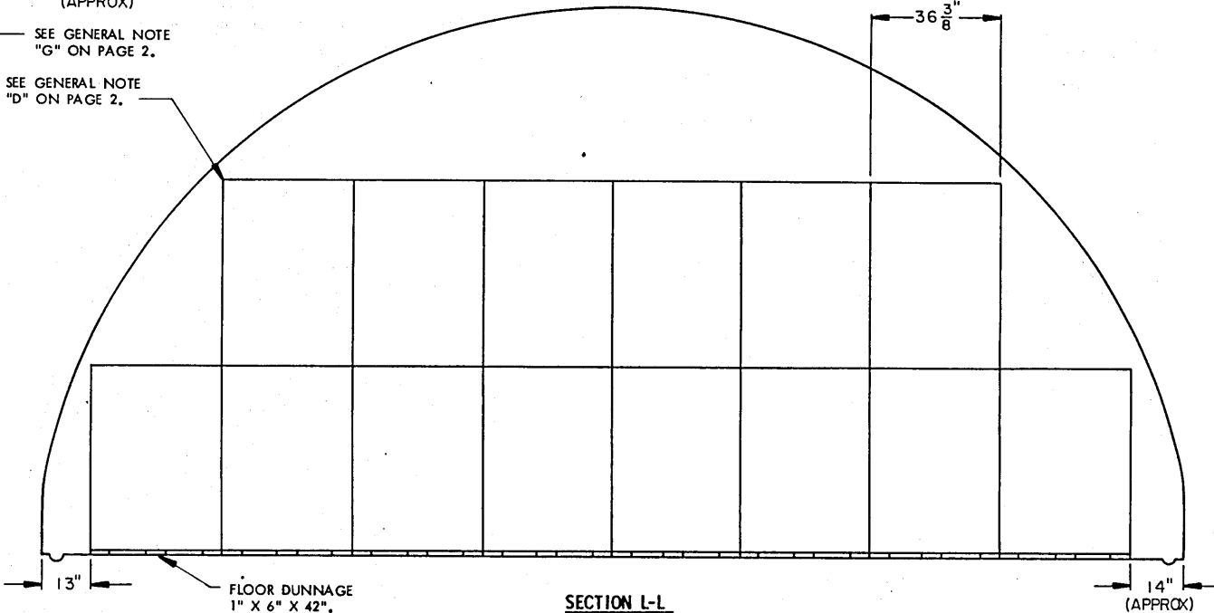
SECTION L-L ( "A" STACK, 14 PALLET UNITS )
