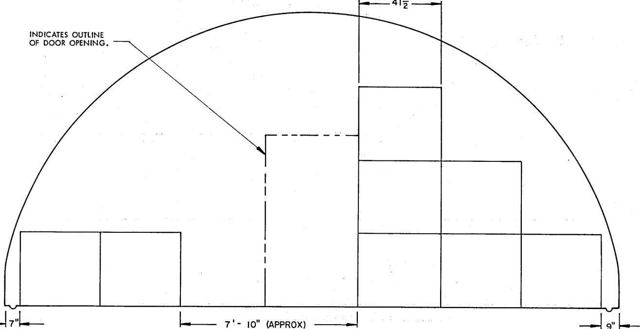
SECTION A3-A3 ( "C" STACK, 8 PALLET UNITS )
