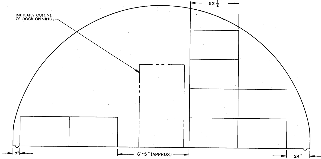
SECTION V1-V1 ( "C" STACK, 8 PALLET UNITS )
