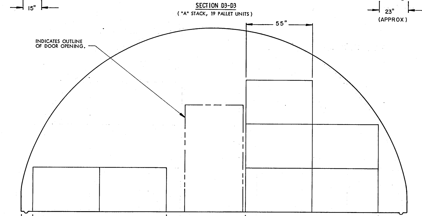
SECTION E3-E3 ( "C" STACK, 7 PALLET UNITS )
