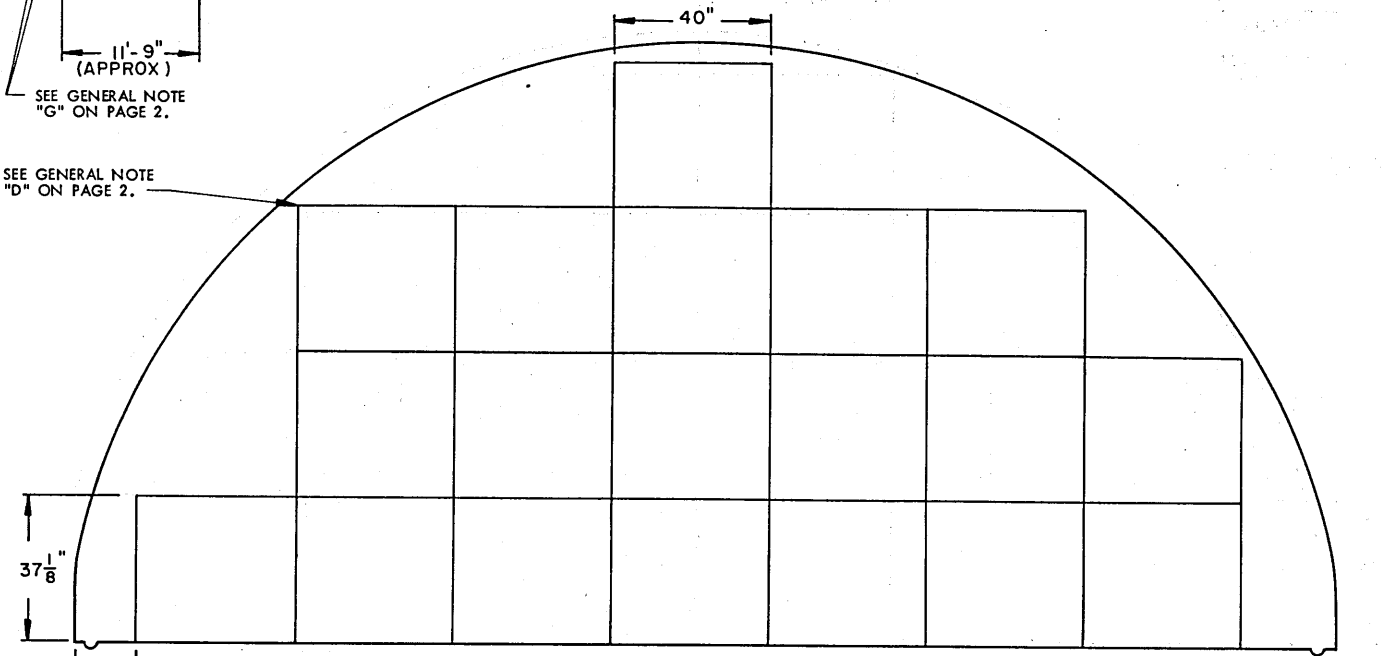
SECTION D3-D3 ( "A" STACK, 19 PALLET UNITS )
