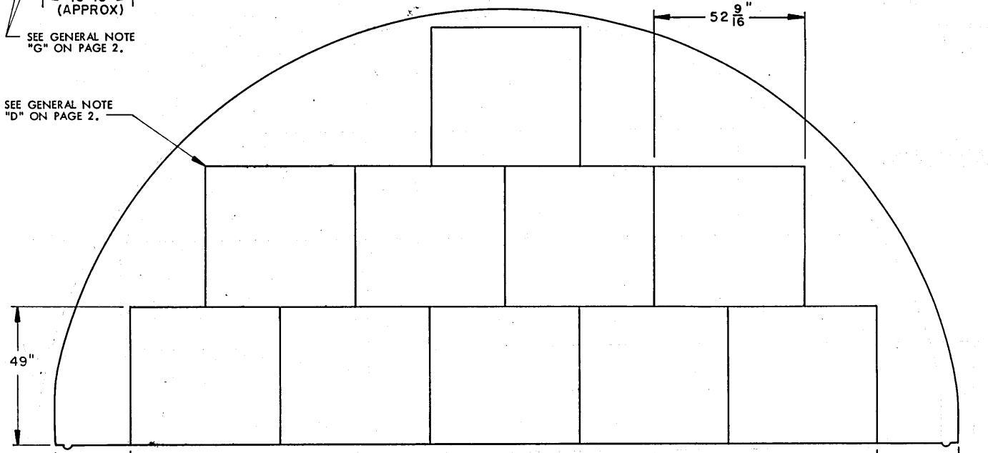
SECTION E4-E4 ( "A" STACK, 10 PALLET UNITS )
