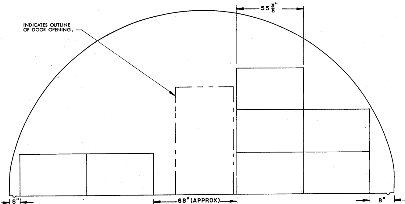
SECTION M2-M2 ( "C" STACK, 7 PALLET UNITS )
