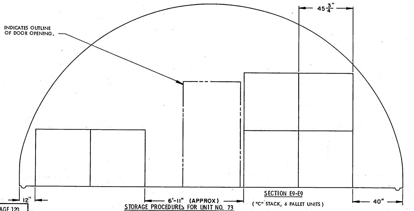
SECTION D9-D9 ( "A" STACK, 16 PALLET UNITS )
