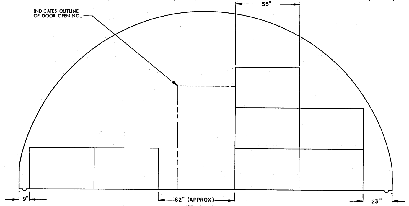
SECTION L5-L5 ( "C" STACK, 7 PALLET UNITS )
