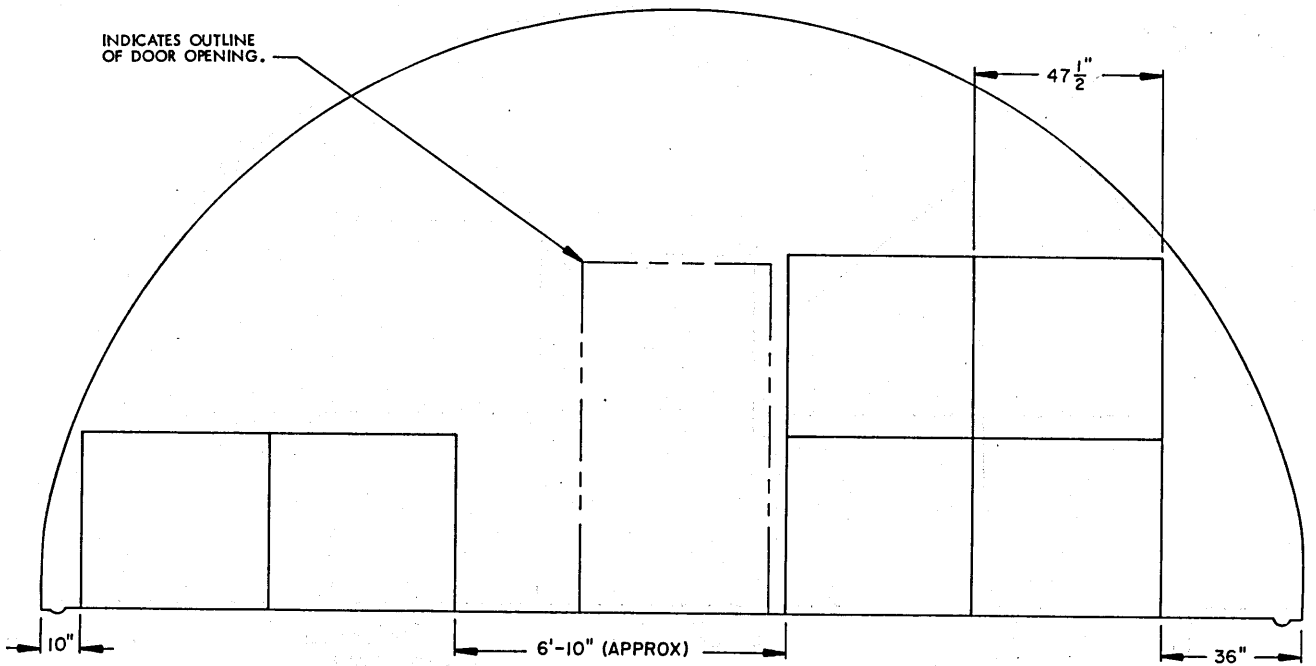
SECTION P5-P5 ( "C" STACK, 6 PALLET UNITS )
