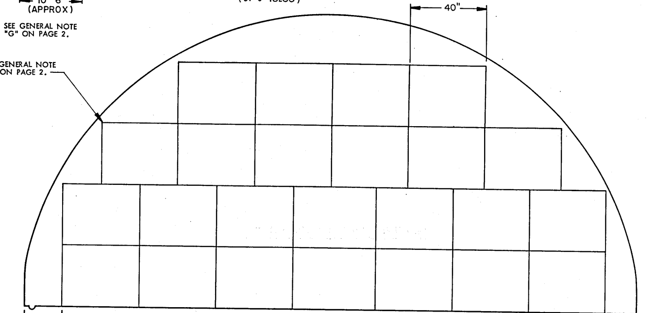
SECTION U1-U1 ( "A" STACK, 24 PALLET UNITS )
