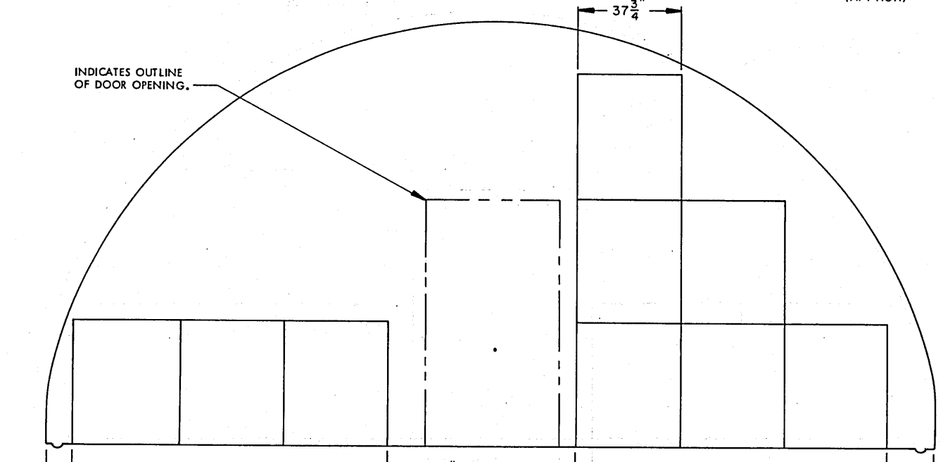
SECTION B6-B6 ( "C" STACK, 9 PALLET UNITS )
