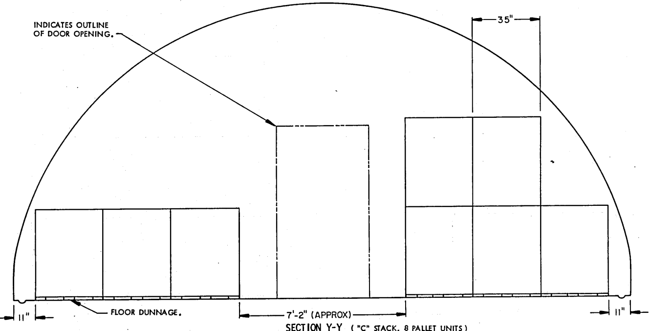
SECTION Y-Y ( "C" STACK, 8 PALLET UNITS )
