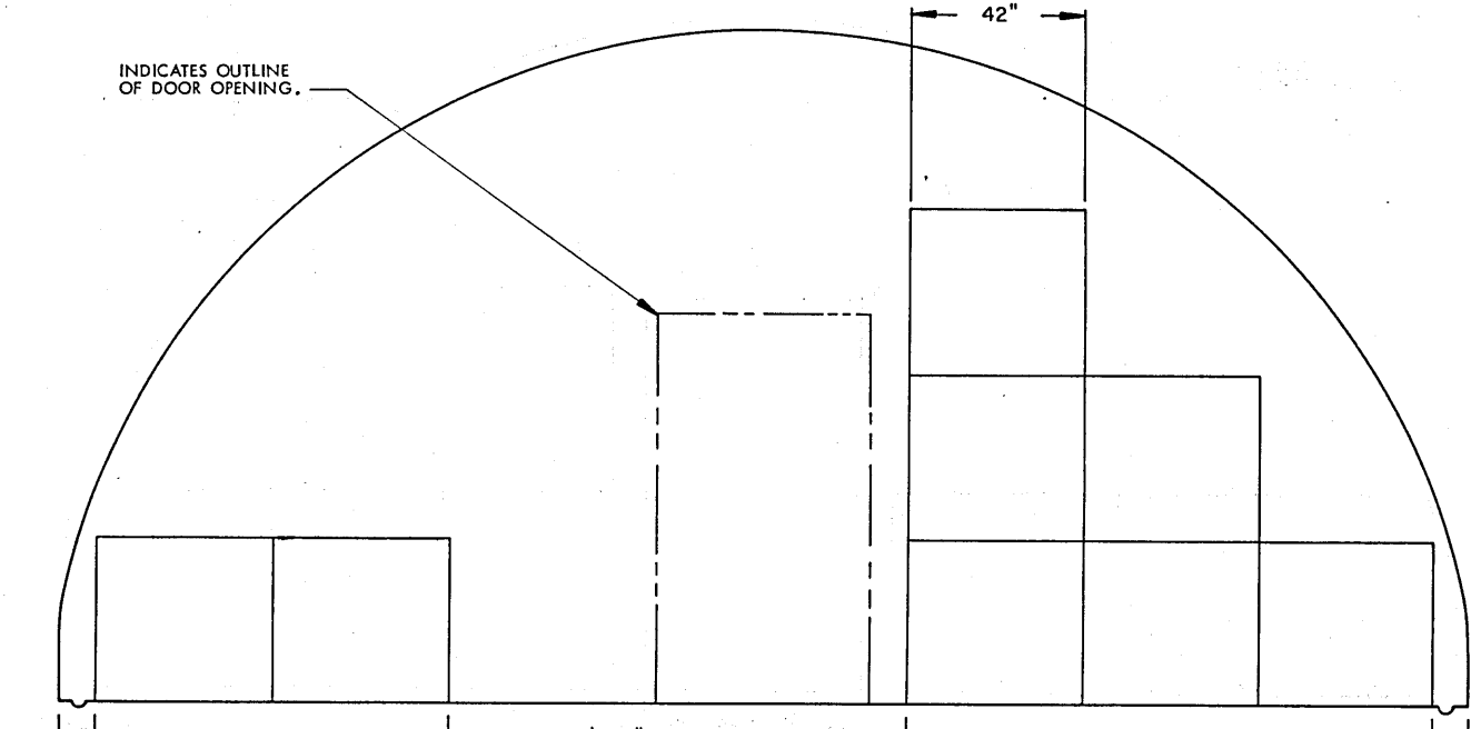
SECTION M4-M4 ( "C" STACK, 8 PALLET UNITS )
