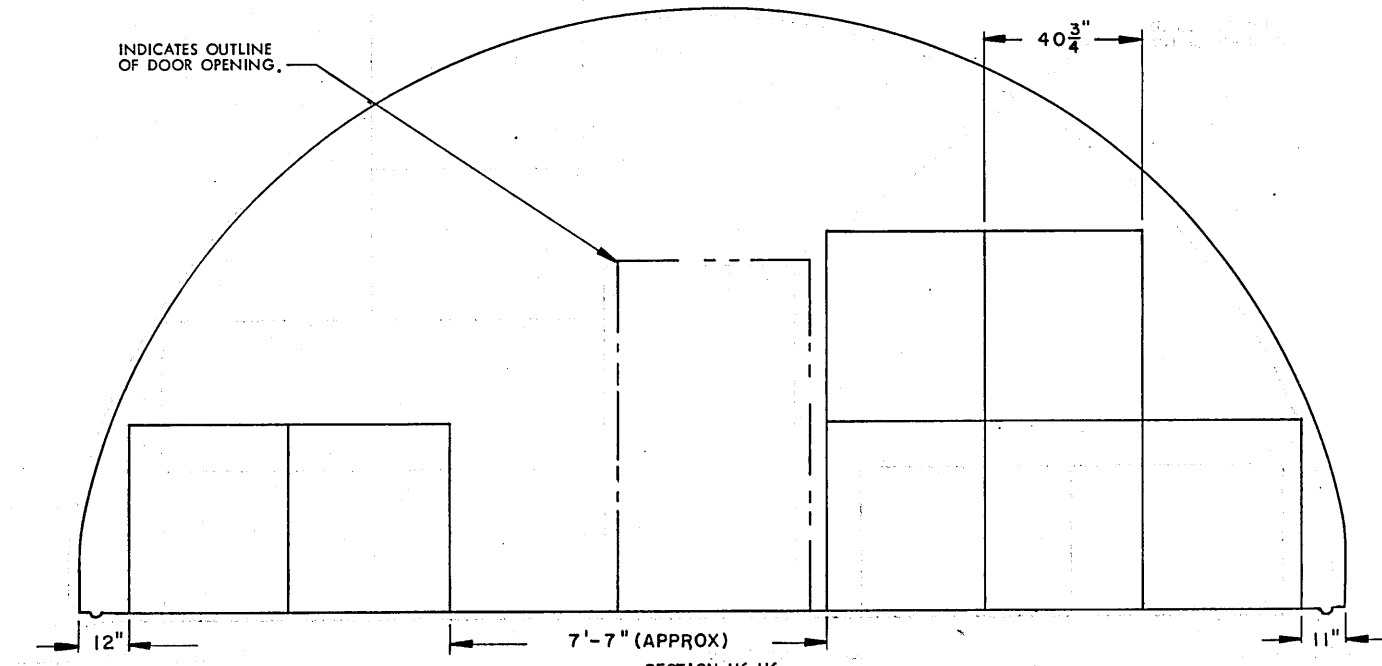
SECTION H6-H6 ( "C" STACK, 7 PALLET UNITS )
