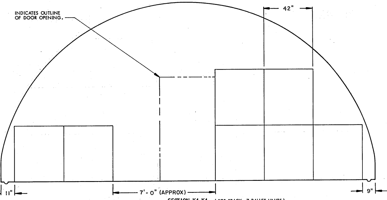
SECTION K4-K4 ( "C" STACK, 7 PALLET UNITS ) STORAGE PROCEDURES FOR UNIT NO. 43
