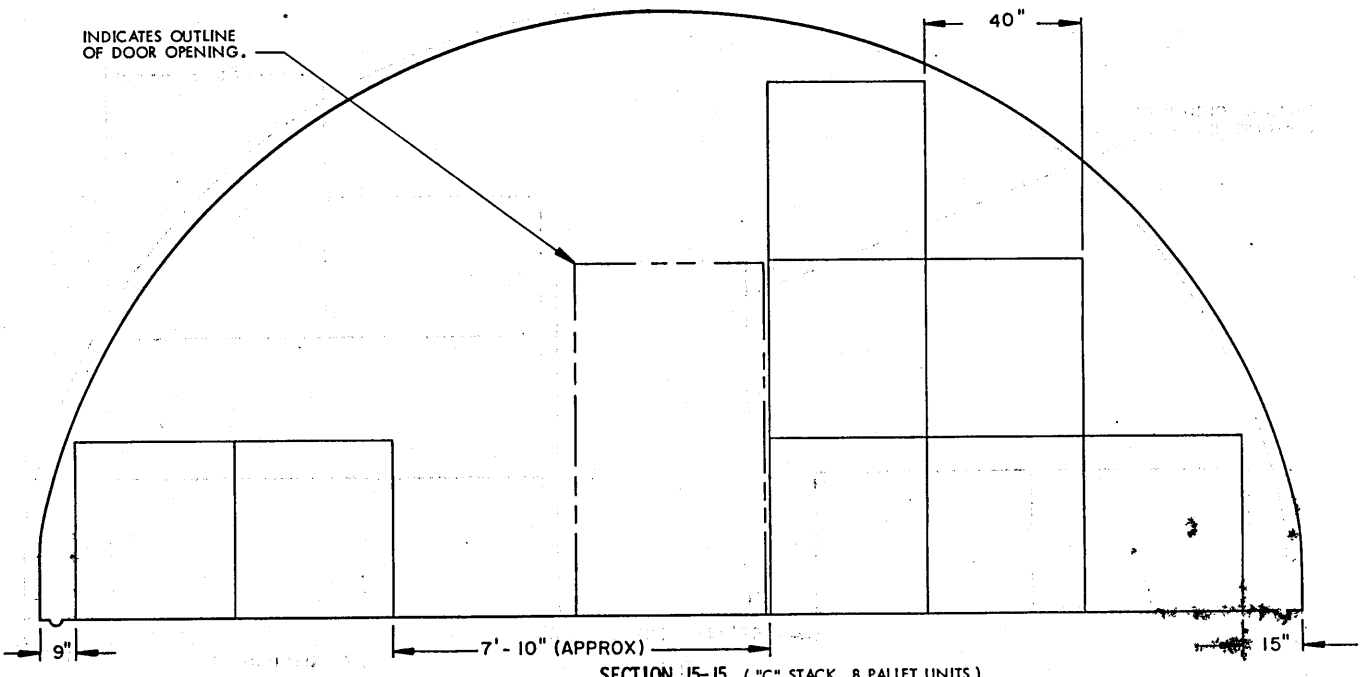
SECTION J5-J5 ( "C" STACK, 8 PALLET UNITS )
