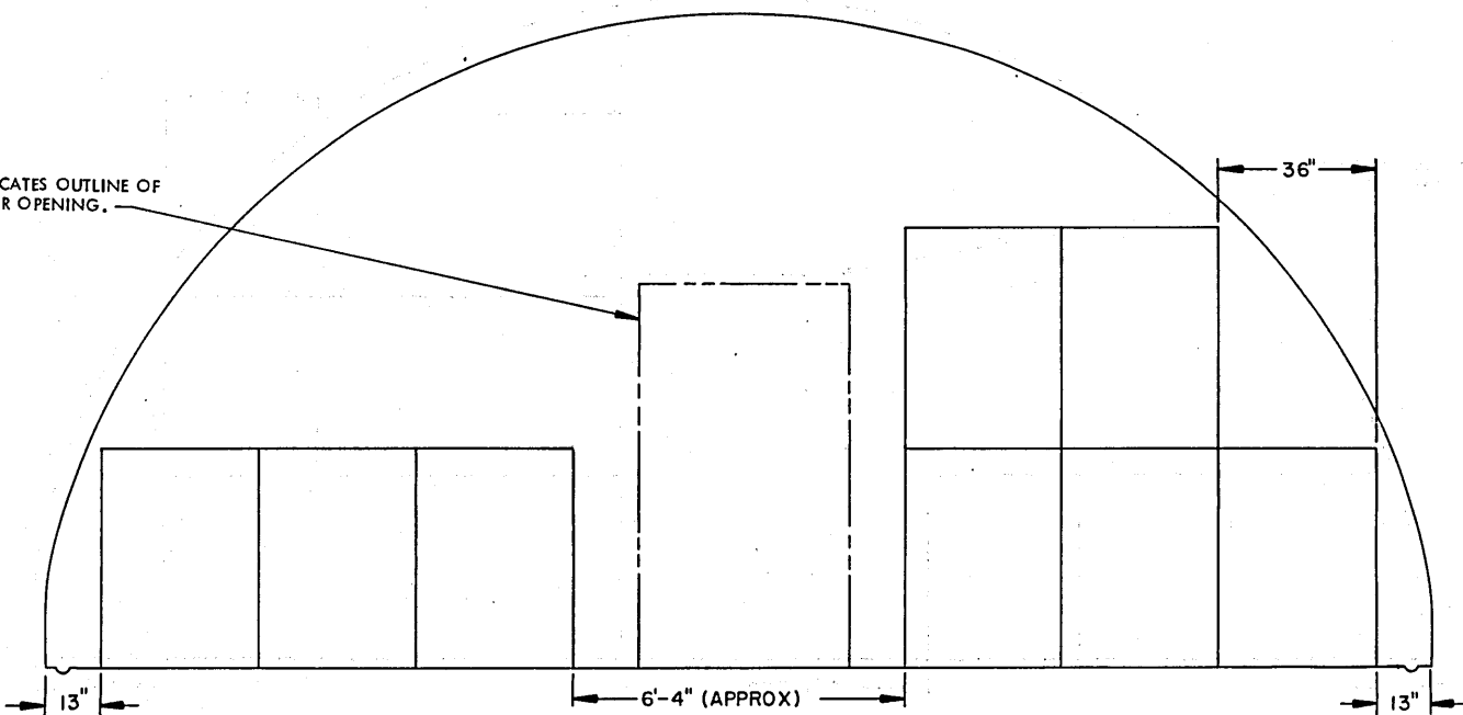
SECTION U8-U8 ( "C" STACK, 8 PALLET UNITS )
