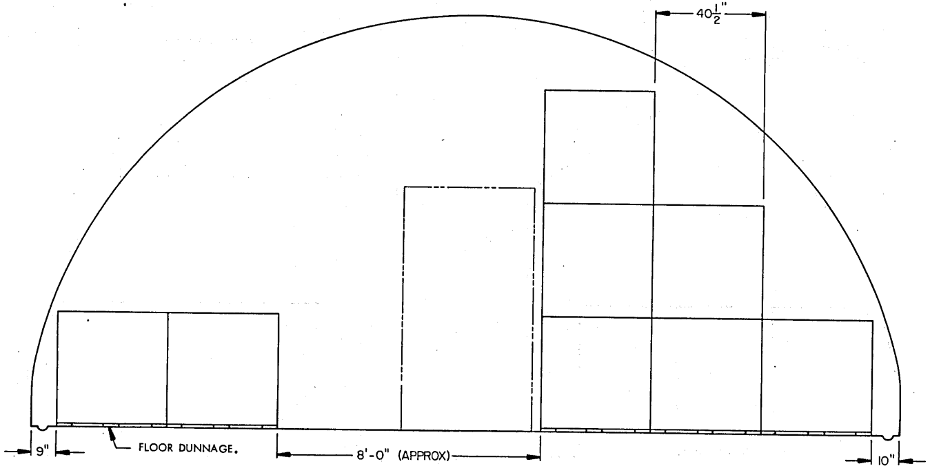
SECTION W-W ( "C" STACK, 8 PALLET UNITS ) STORAGE PROCEDURES FOR UNIT NO. 11
