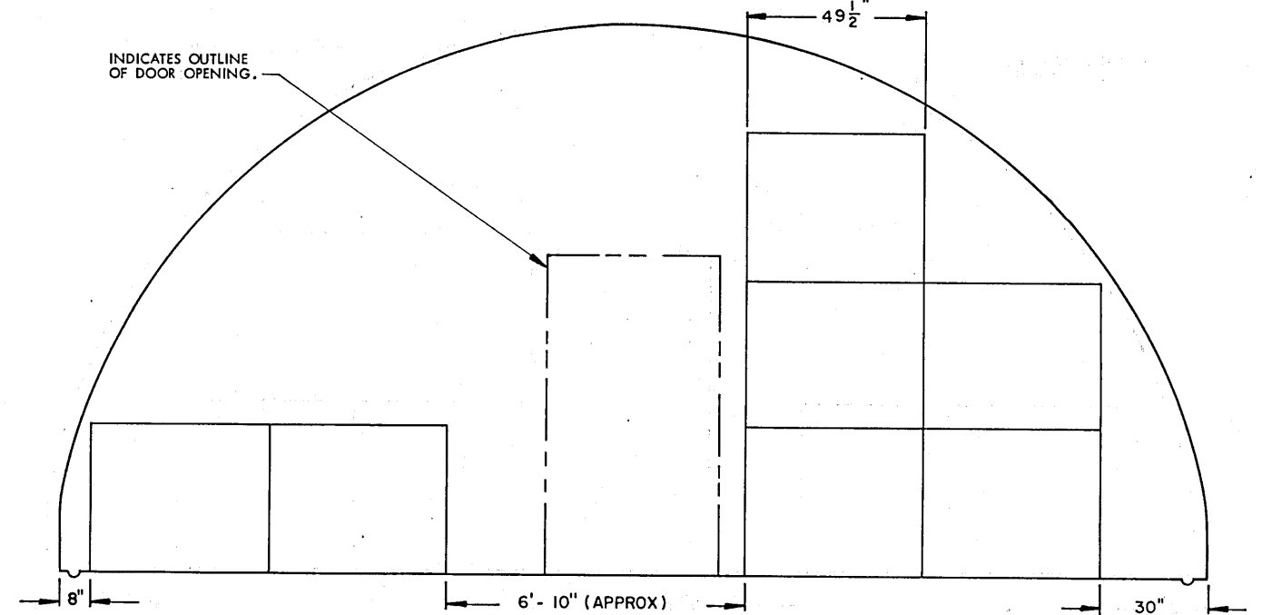
SECTION J3-J3 ("C" STACK, 7 PALLET UNITS)
