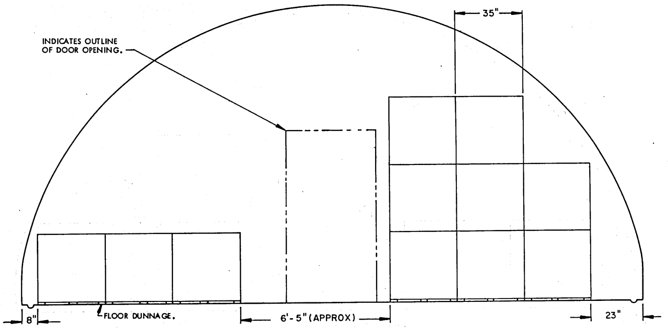
SECTION G1-G1 ( "C" STACK, 11 PALLET UNITS) STORAGE PROCEDURES FOR UNIT NO. 16
