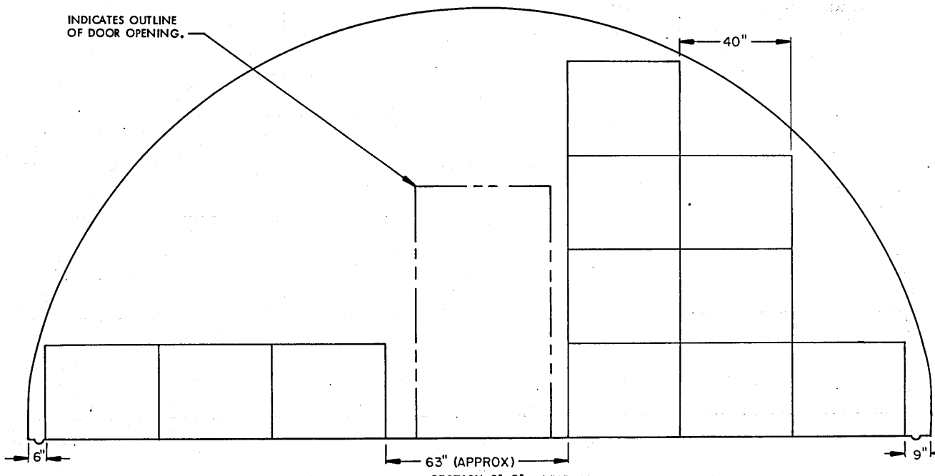
SECTION C1-C1 ( "C" STACK, 11 PALLET UNITS) STORAGE PROCEDURES FOR UNIT NO. 14
