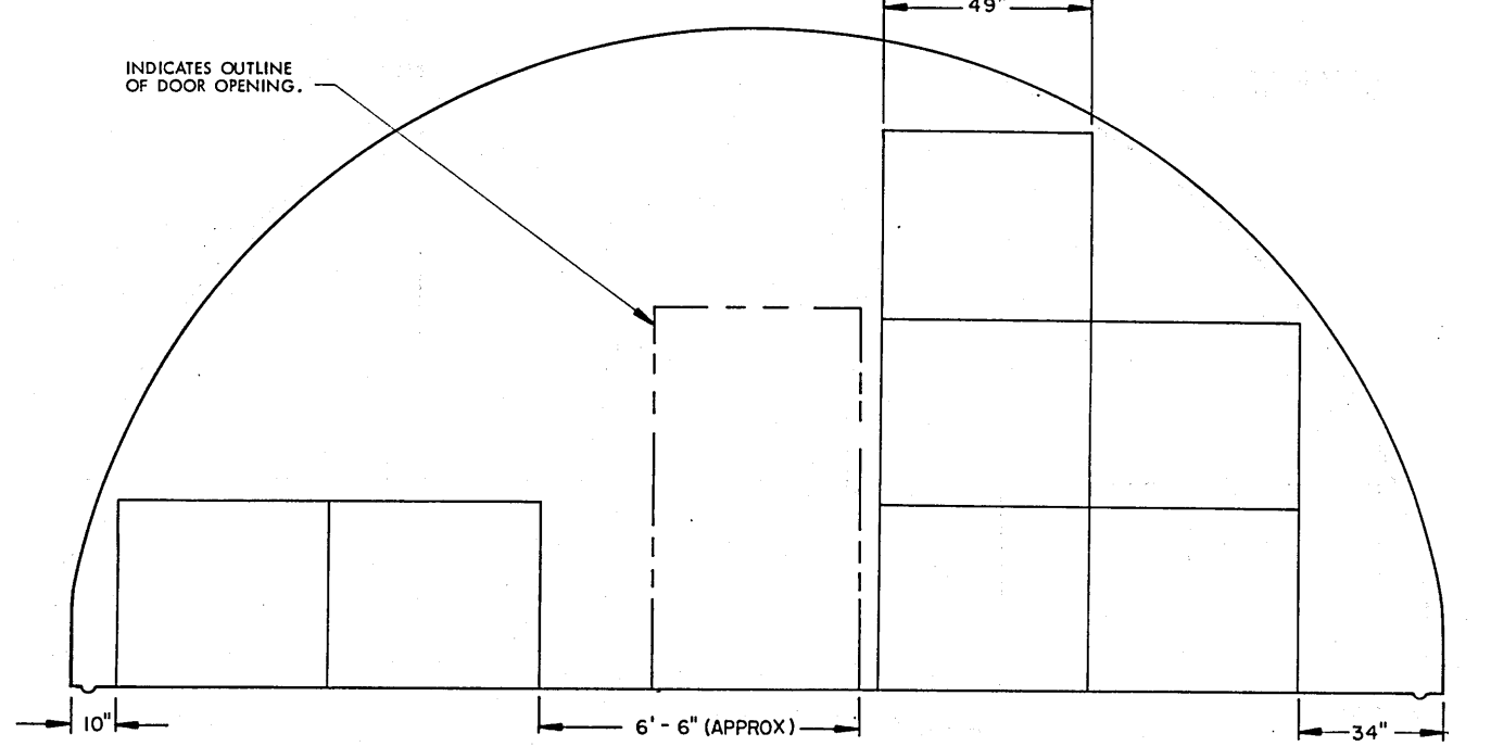
SECTION V3-V3 ( "C" STACK, 7 PALLET UNITS )
