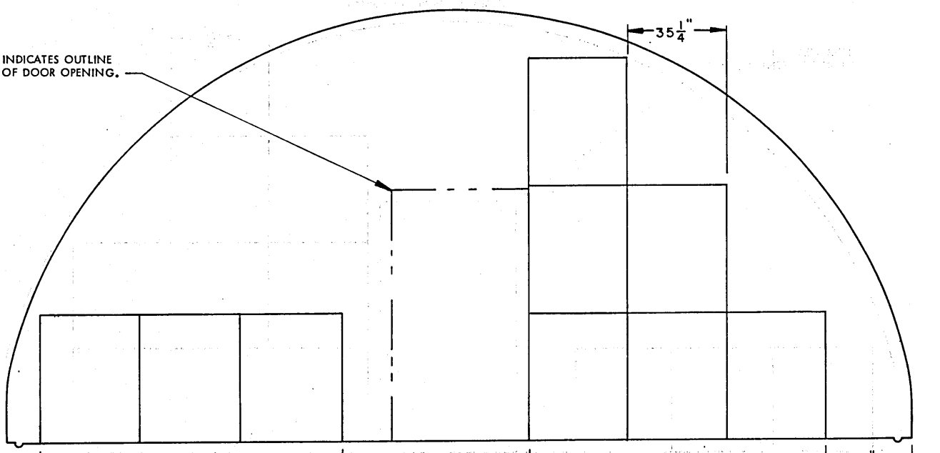
SECTION G7-G7 ( "C" STACK, 9 PALLET UNITS )
