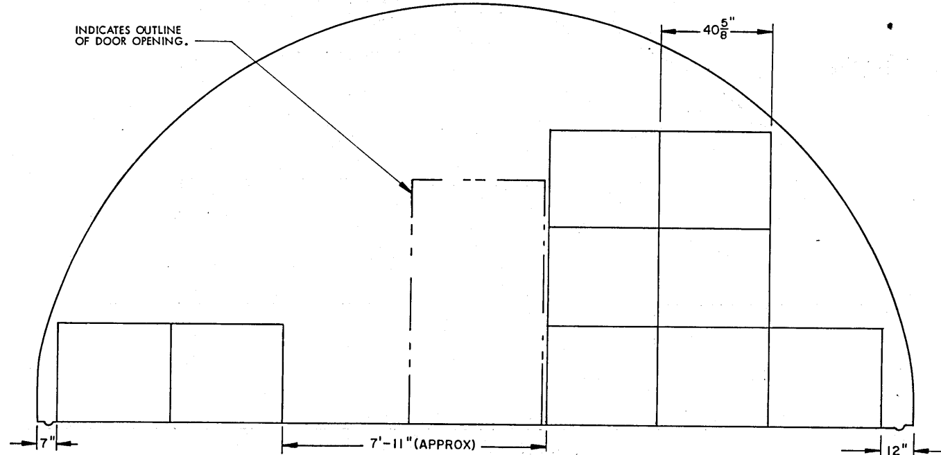
SECTION Q4-Q4 ( "C" STACK, 9 PALLET UNITS )
