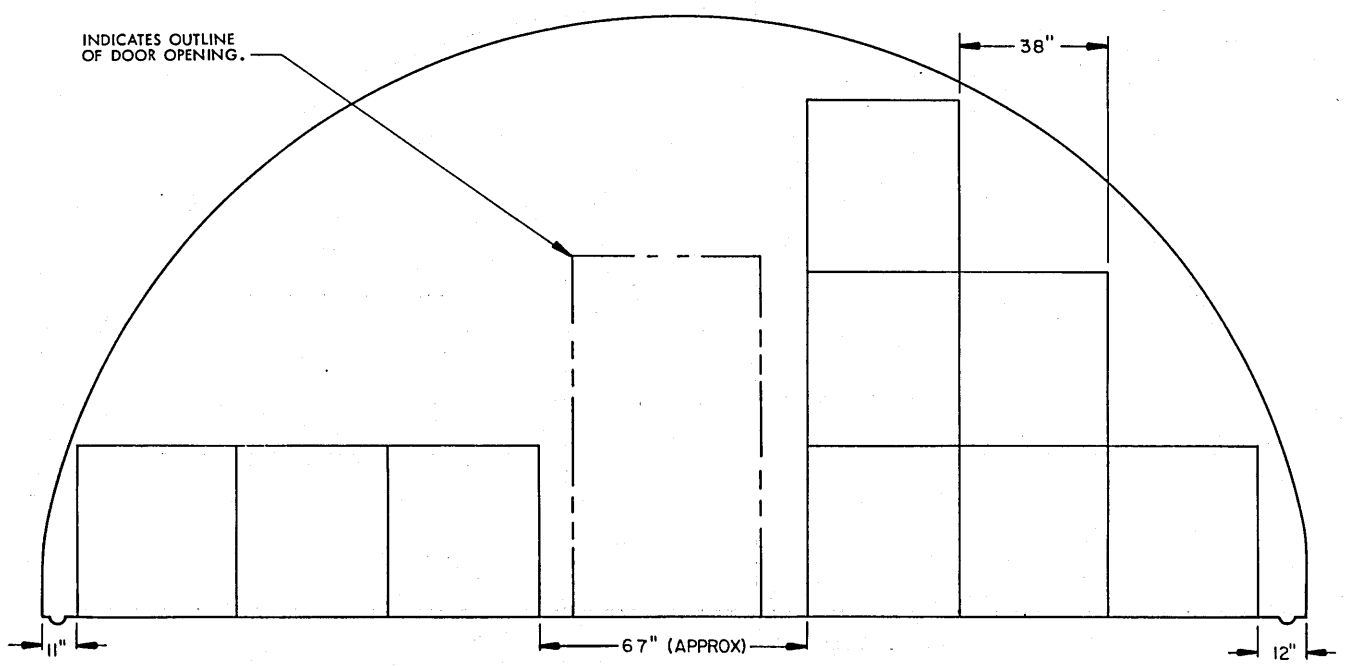
SECTION O6-O6 ( "C" STACK, 9 PALLET UNITS ) STORAGE PROCEDURES FOR UNIT NO. 56 ( INCREASED-HEIGHT UNIT )
