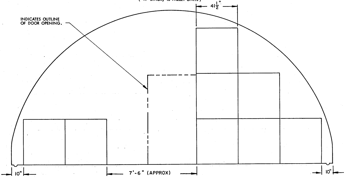
SECTION Y2-Y2 ( "C" STACK, 8 PALLET UNITS )
