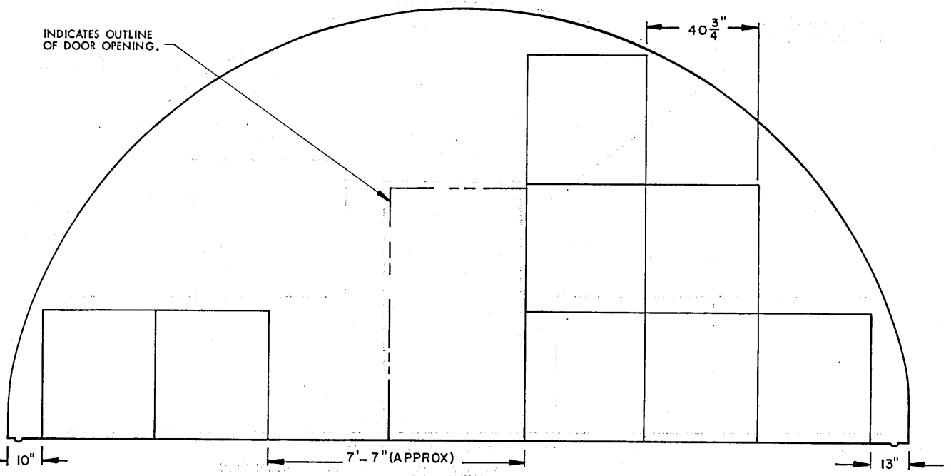
SECTION O2-O2 ( "C" STACK, 8 PALLET UNITS ) STORAGE PROCEDURES FOR UNIT NO. 31 ( INCREASED-HEIGHT UNIT )
