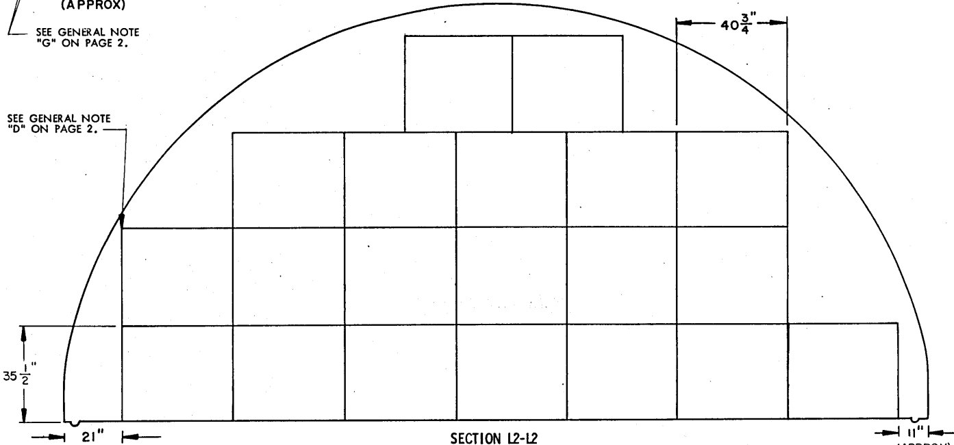
SECTION I2-I2 ( "A" STACK, 20 PALLET UNITS )
