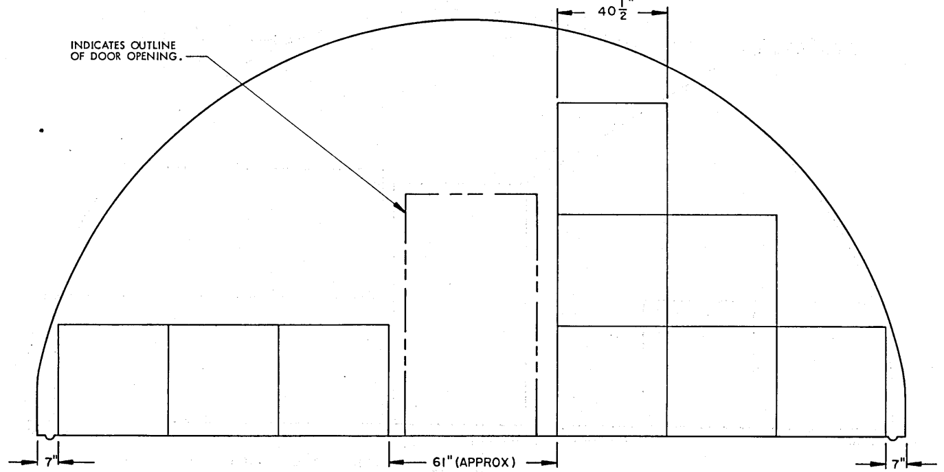
SECTION N3-N3 ("C" STACK, 9 PALLET UNITS)
