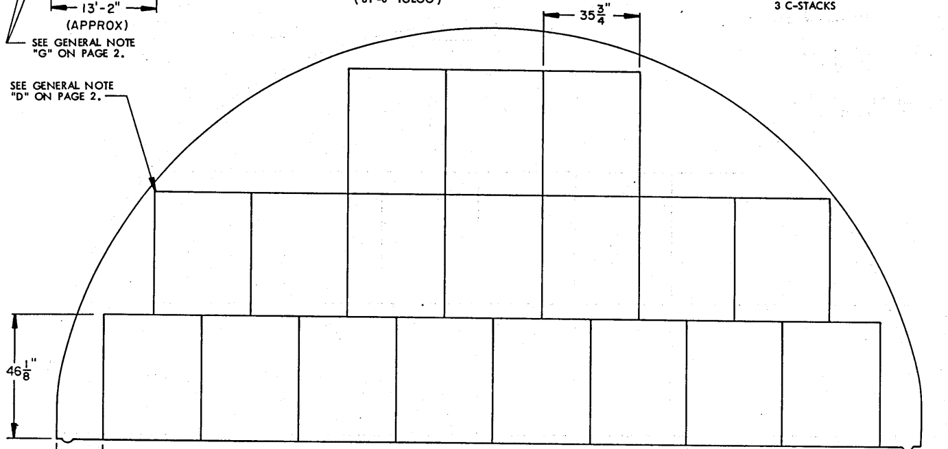
SECTION O5-O5 ( "A" STACK, 18 PALLET UNITS )
