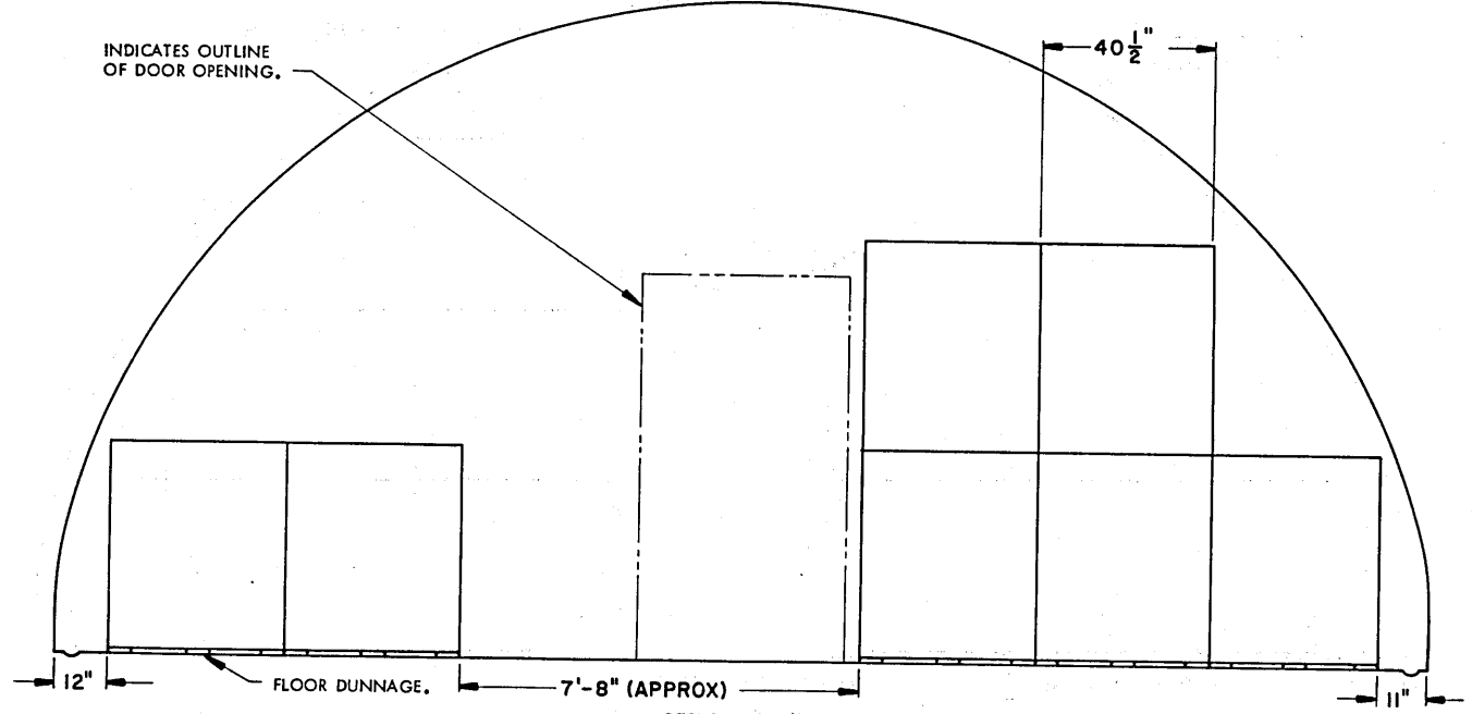
SECTION S-S ( "C" STACK, 7 PALLET UNITS ) STORAGE PROCEDURES FOR UNIT NO. 9
