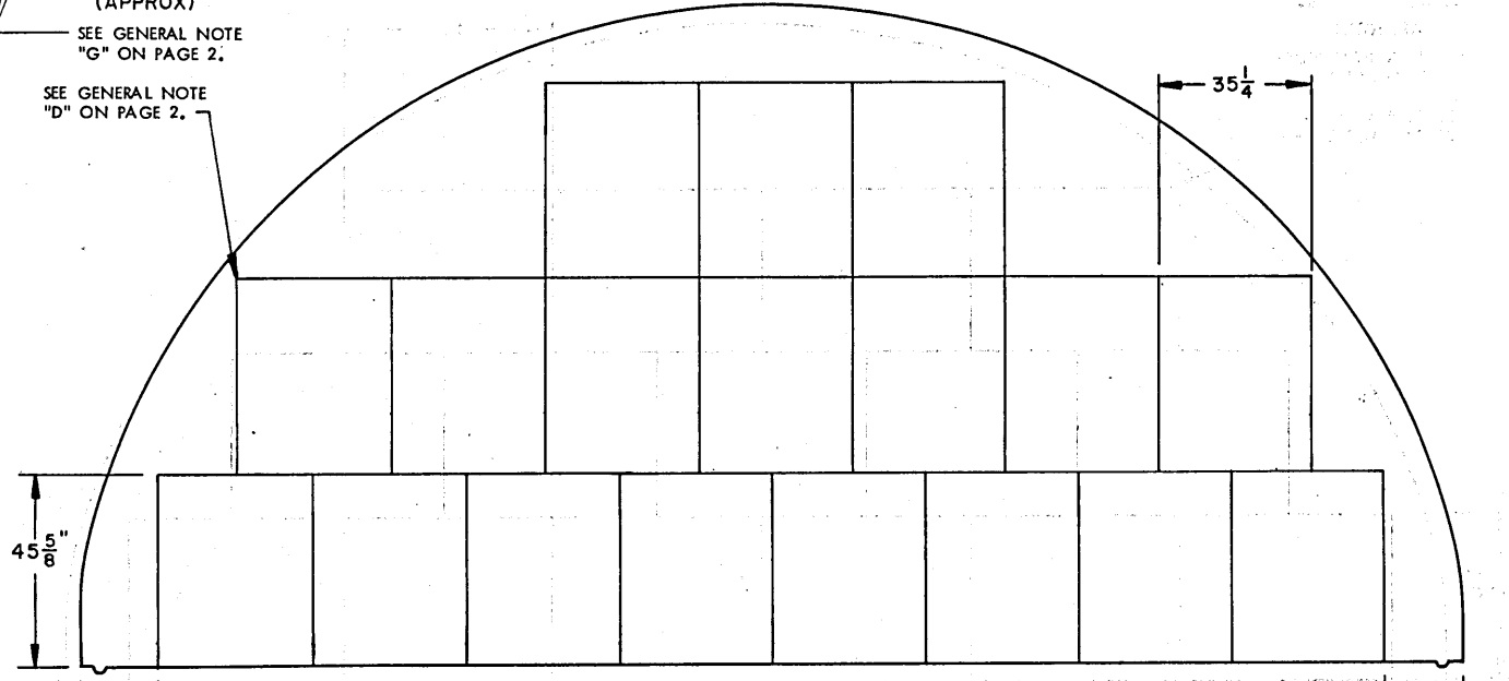
SECTION F7-F7 ( "A" STACK, 18 PALLET UNITS )
