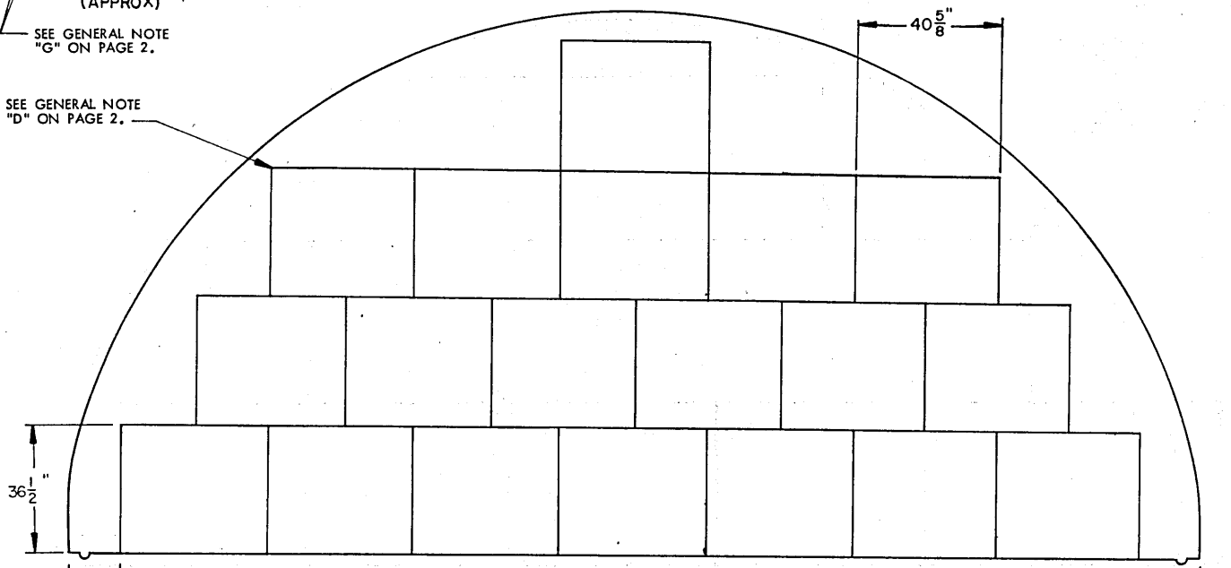
SECTION P4-P4 ( "A" STACK, 19 PALLET UNITS )
