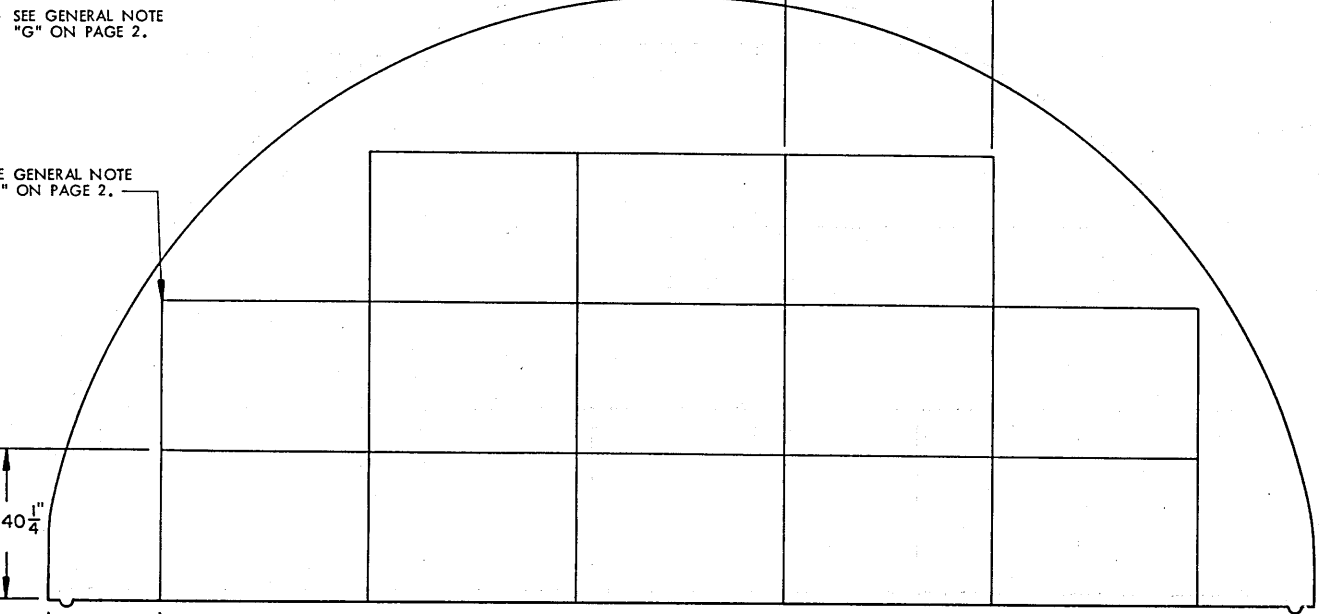
SECTION L4-L4 ( "A" STACK, 13 PALLET UNITS )
