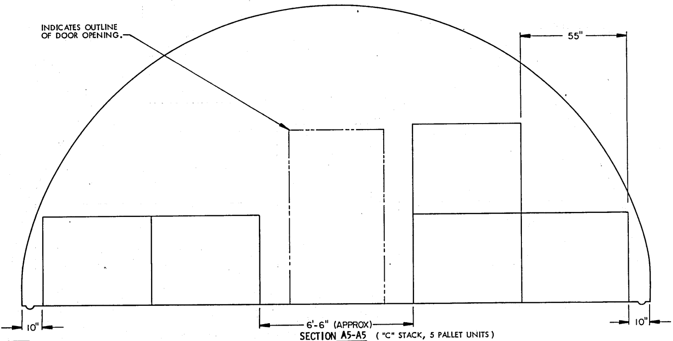
SECTION A5-A5 ("C" STACK, 5 PALLET UNITS) STORAGE PROCEDURES FOR UNIT NO. 47
