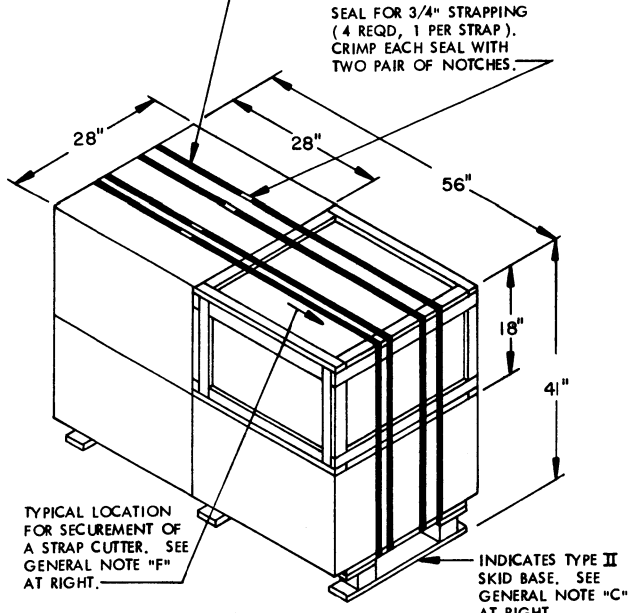
SKIDDED UNIT SEE GENERAL NOTE "B" AT RIGHT.
