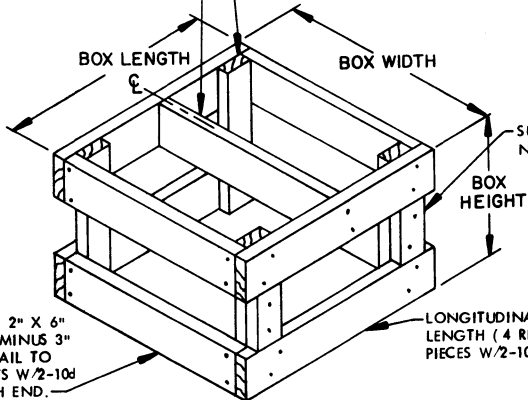
FILLER ASSEMBLY ( FOR MINUS ONE BOX )
