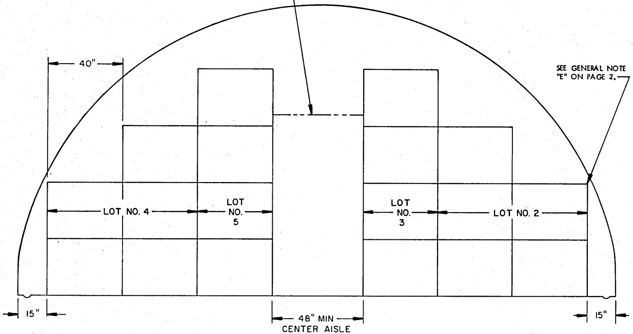
SECTION R-R
