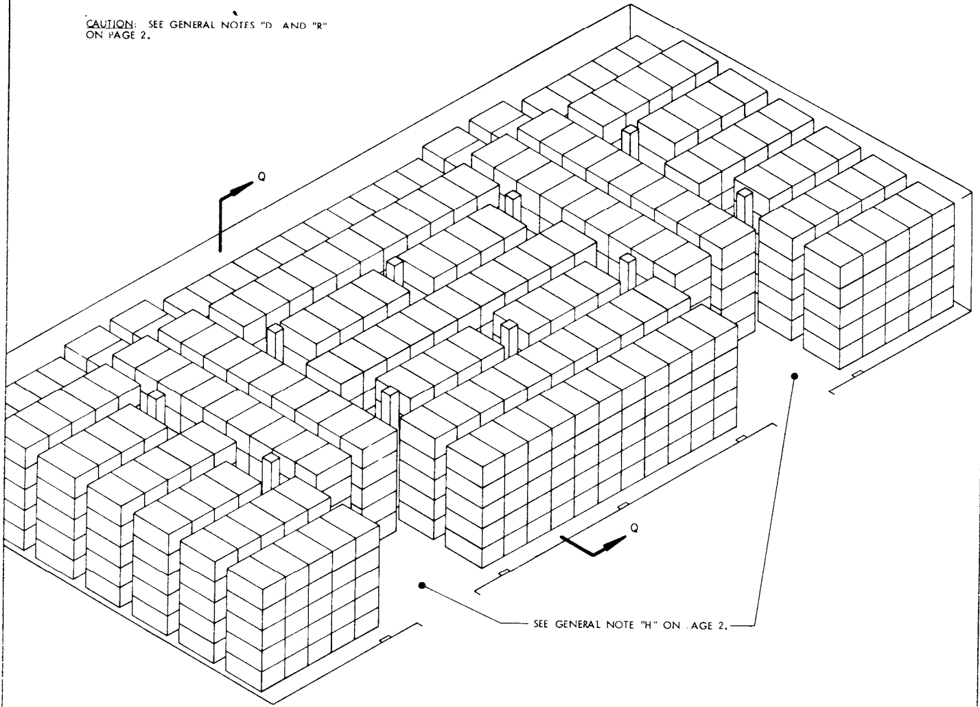
ISOMETRIC VIEW ( 100' X 50' MAGAZINE )
