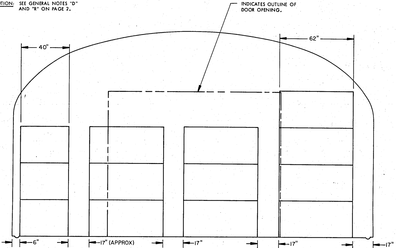
SECTION M-M
