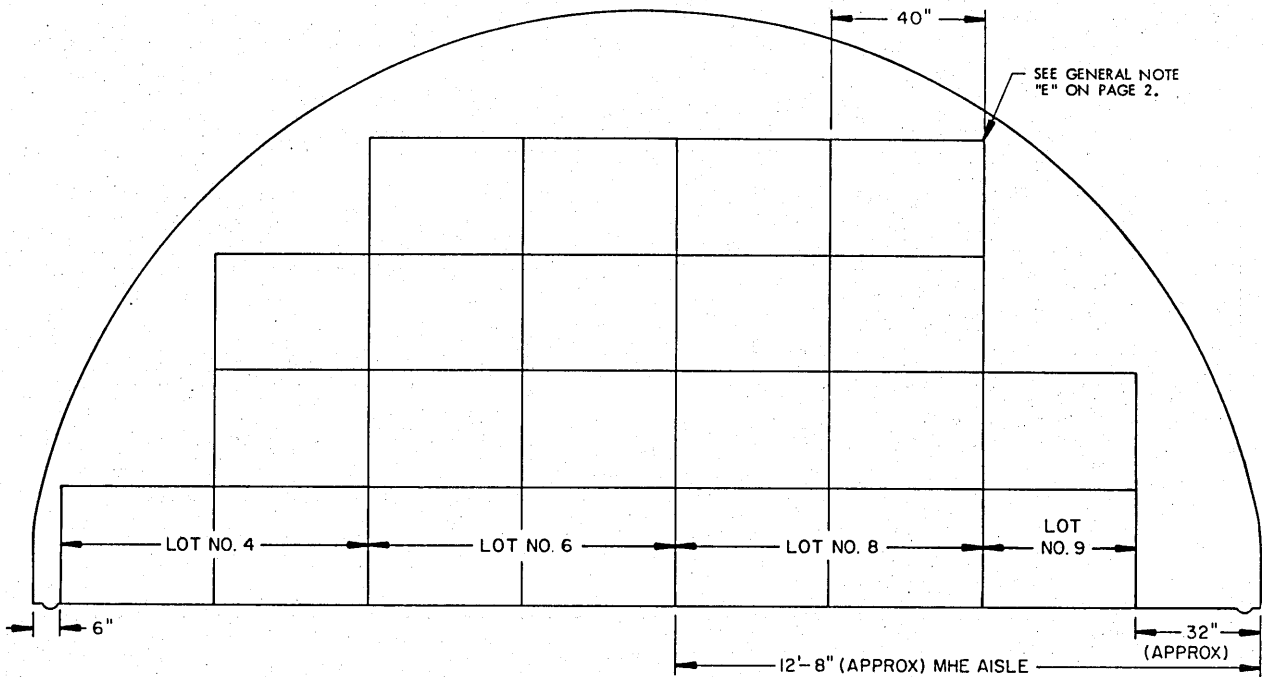
SECTION S-S
