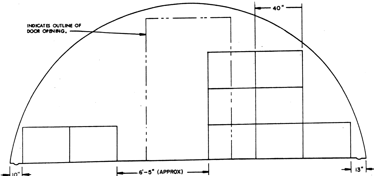
SECTION F-F
