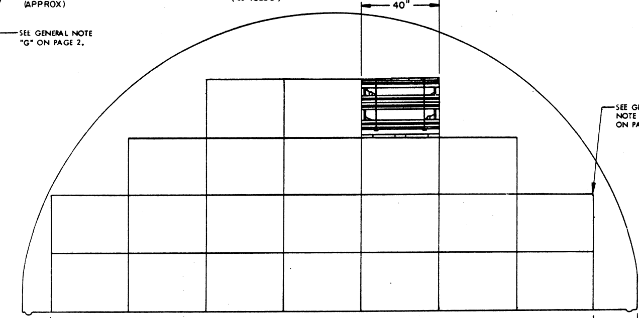
SECTION A-A ( "A" STACK, 22 PALLET UNITS )
