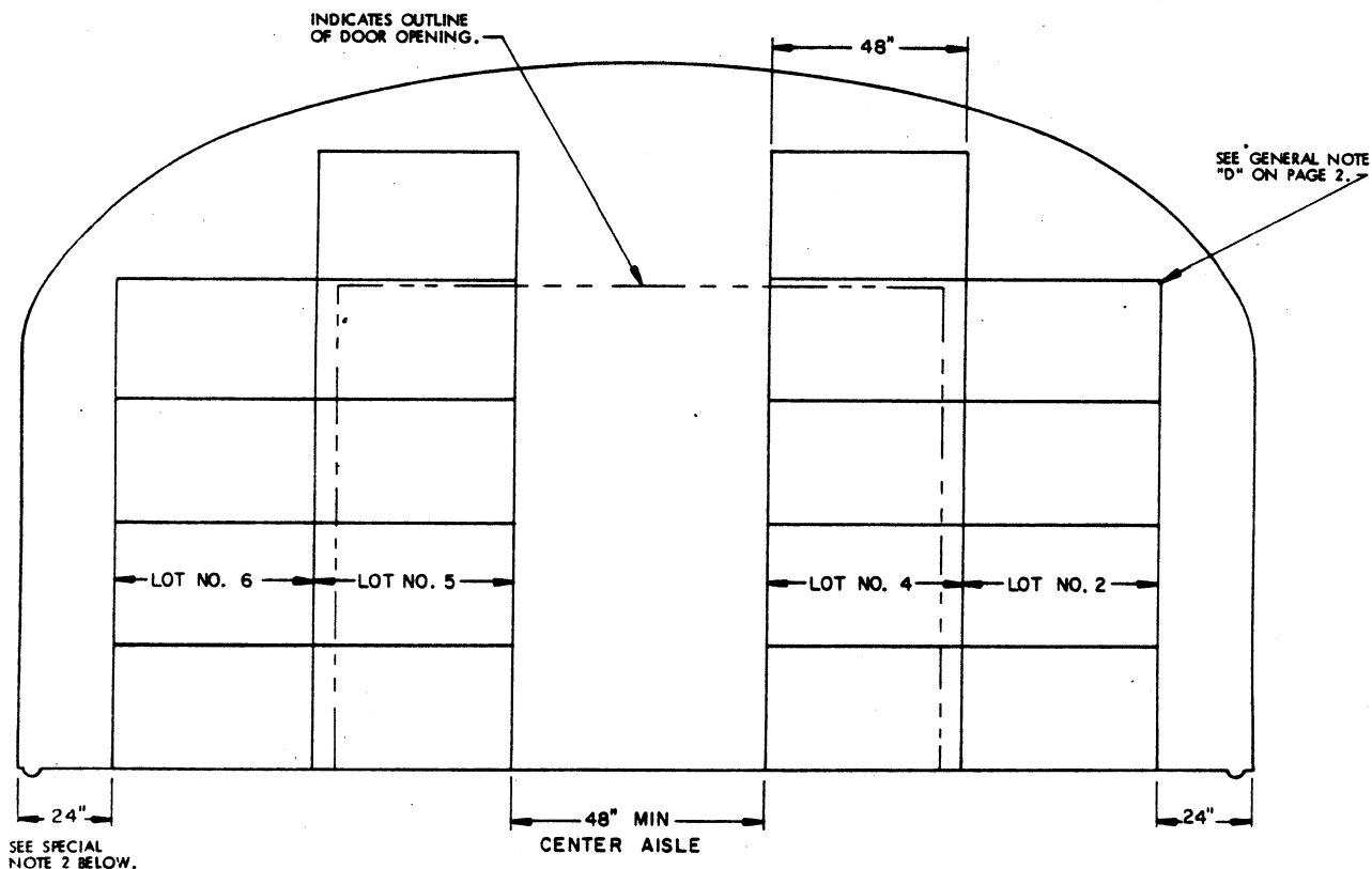
SECTION T-T
