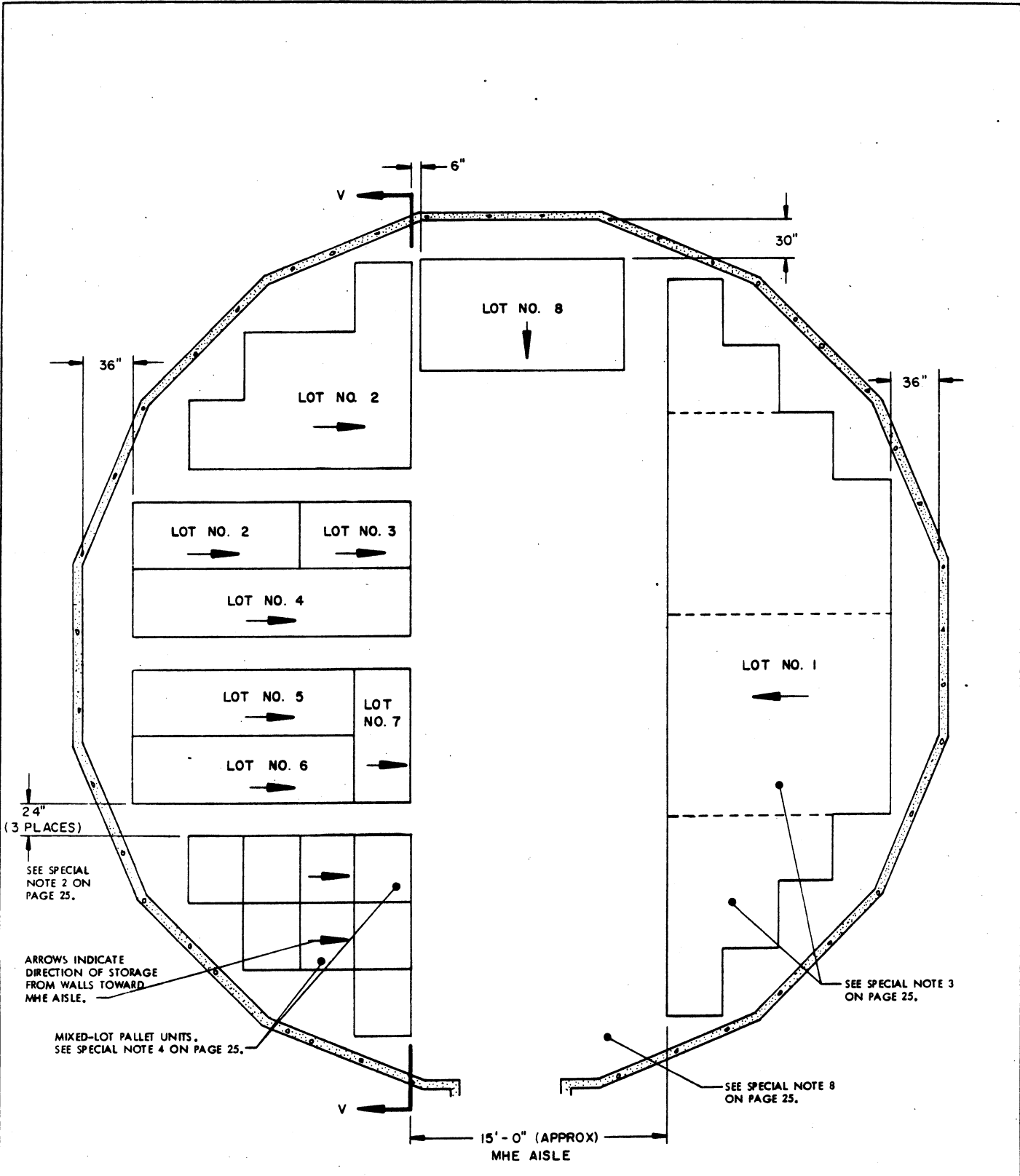
PLAN VIEW
