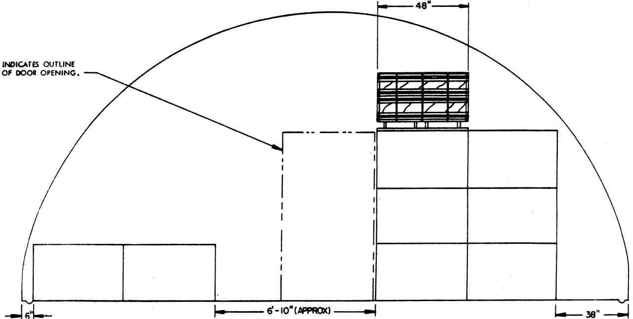
SECTION B-B ( "C" STACK, 9 PALLET UNITS )
