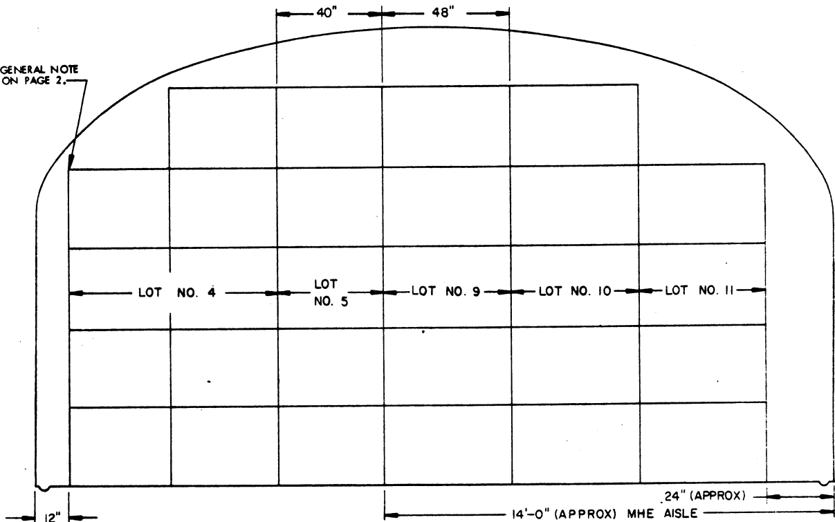
SECTION U-U
