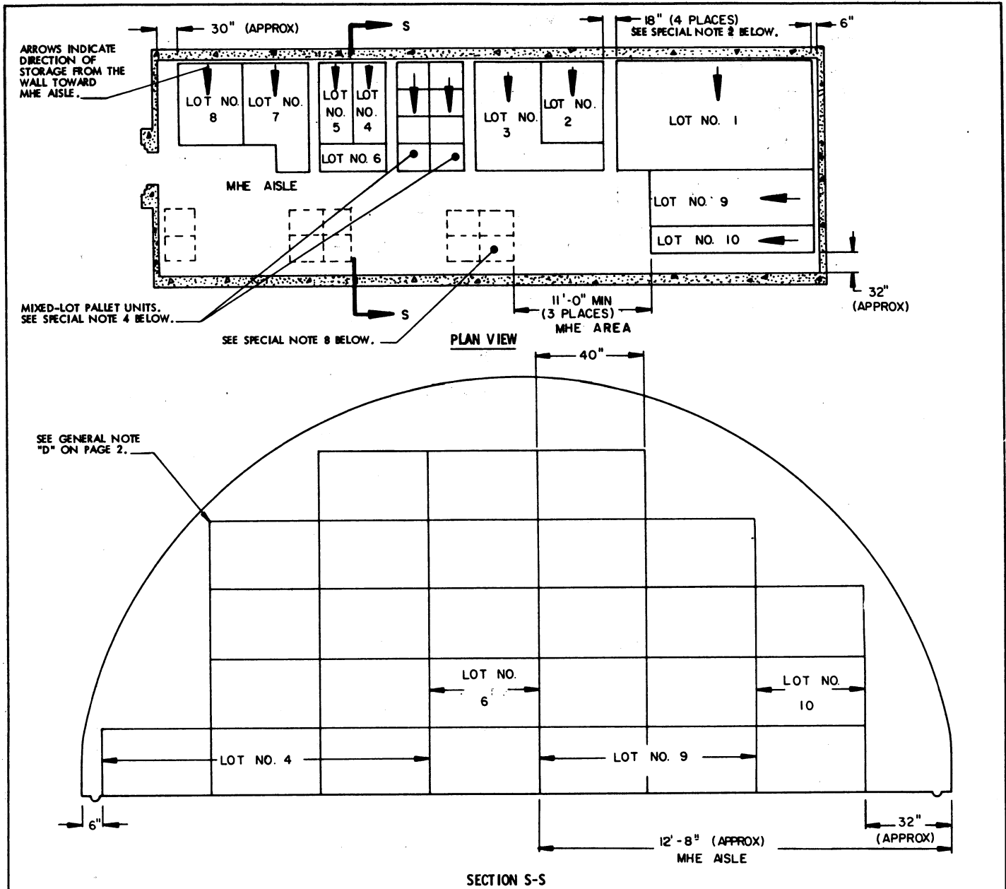
SECTION S-S
