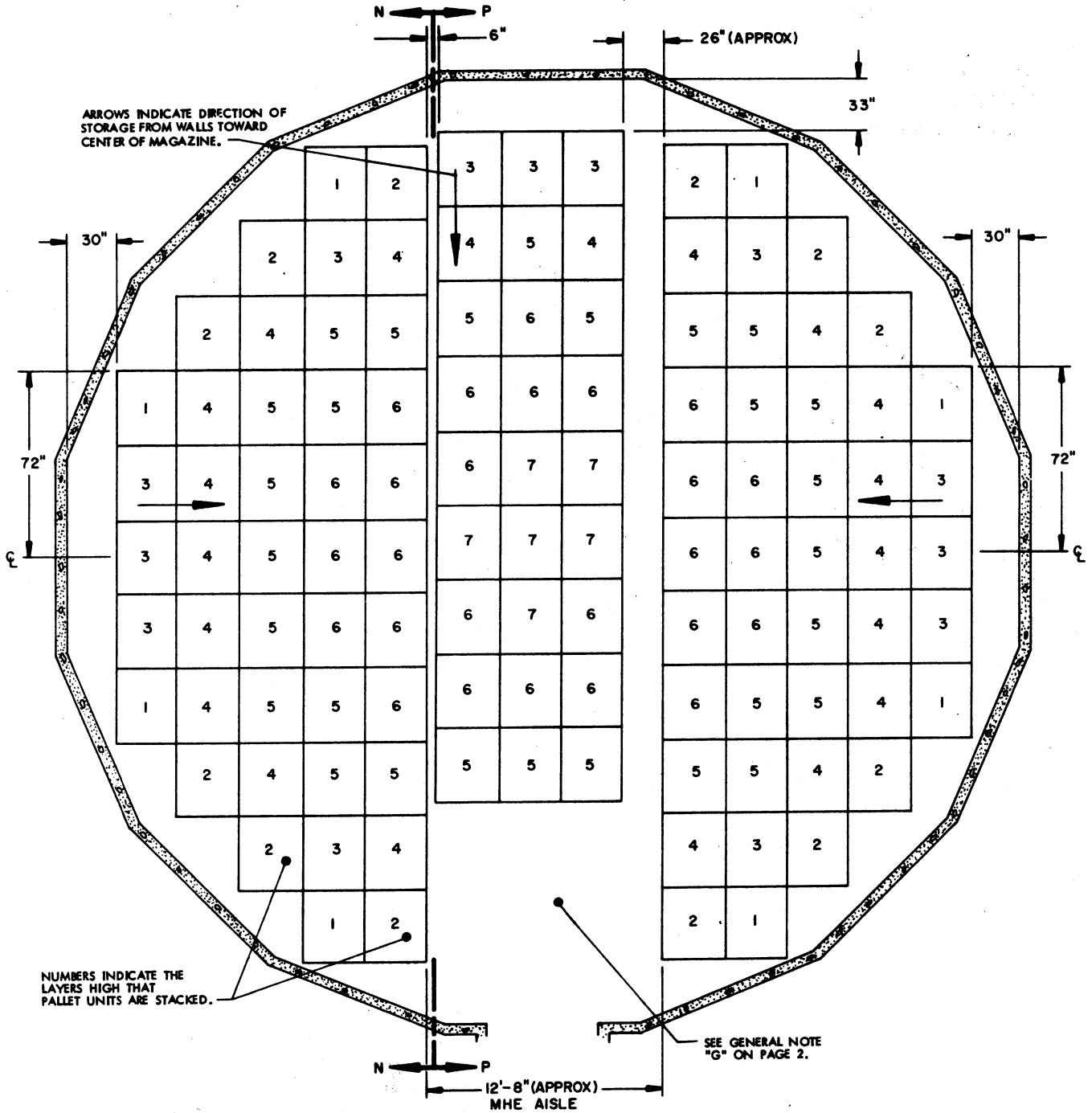
PLAN VIEW
