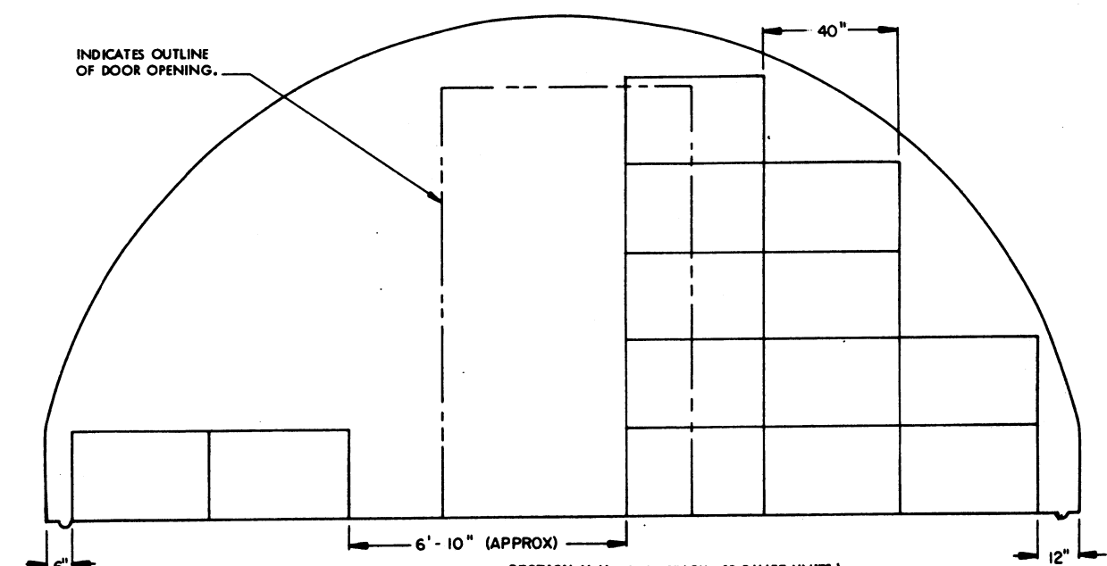
SECTION H-H ( "C" STACK, 13 PALLET UNITS )
