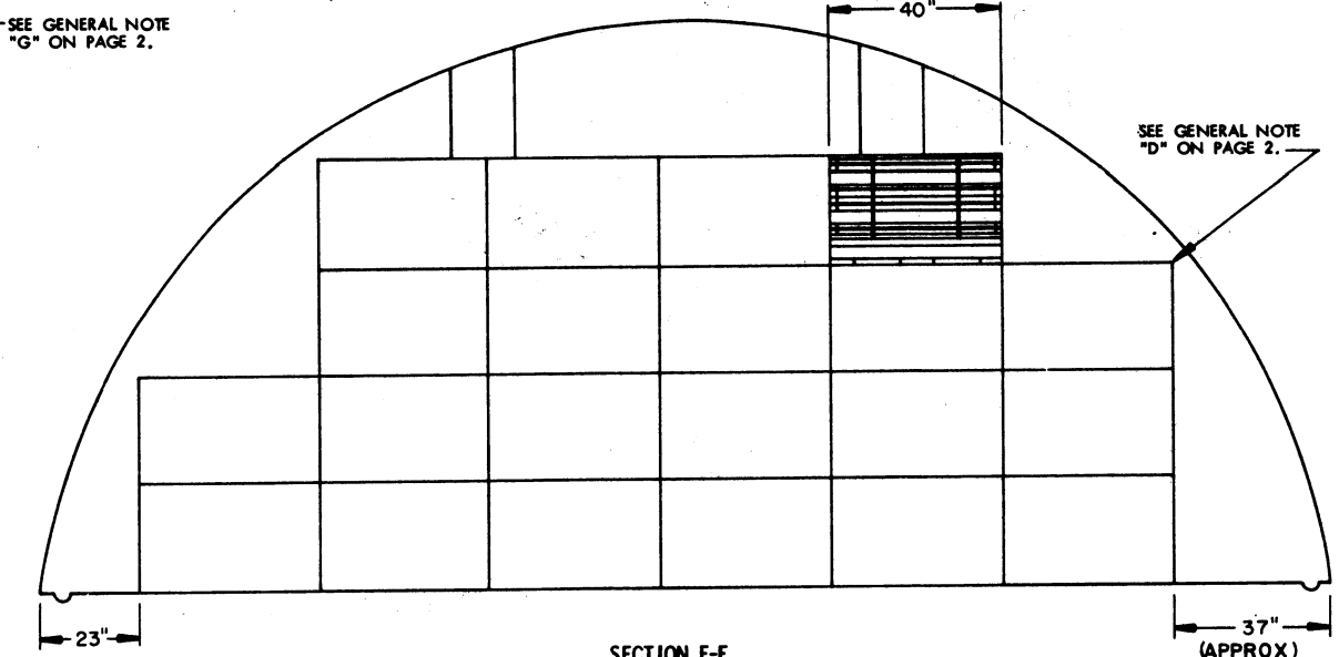
SECTION E-E ( "A" STACK, 21 PALLET UNITS )
