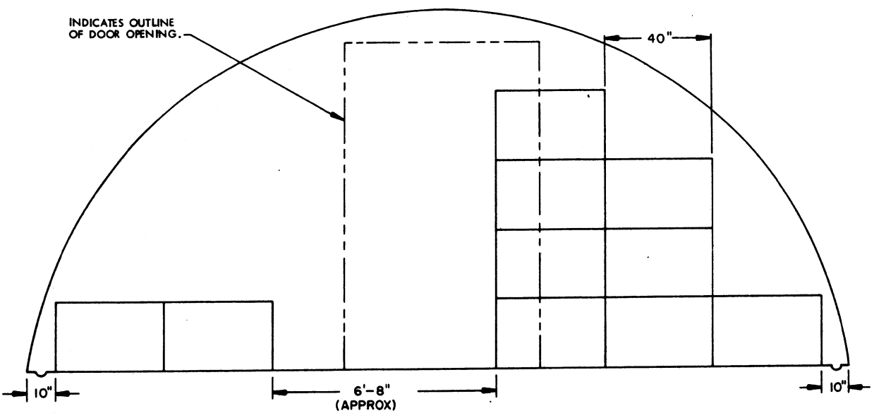
SECTION F-F ( "C" STACK, 10 PALLET UNITS )
