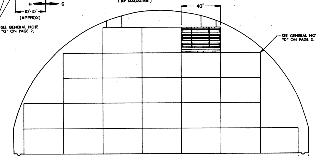
SECTION G-G ( "A" STACK, 26 PALLET UNITS )
