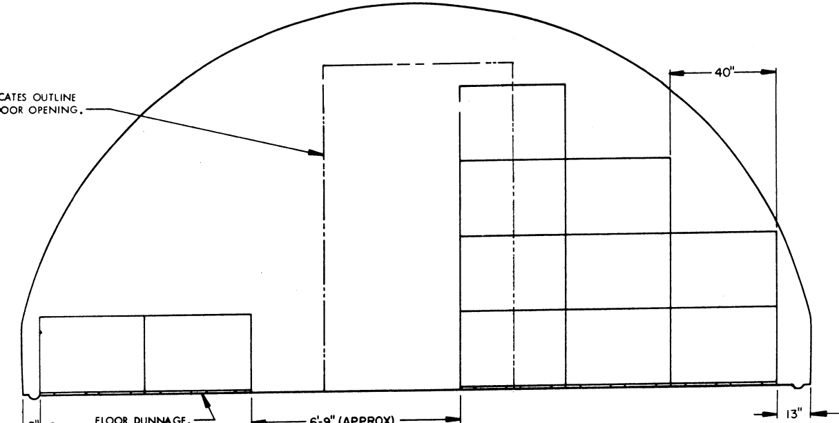
SECTION H-H ( "C" STACK, 11 PALLET UNITS )
