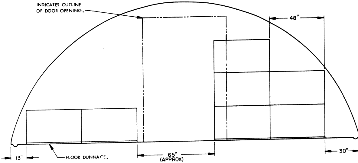
SECTION D-D ( "C" STACK, 7 PALLET UNITS )
