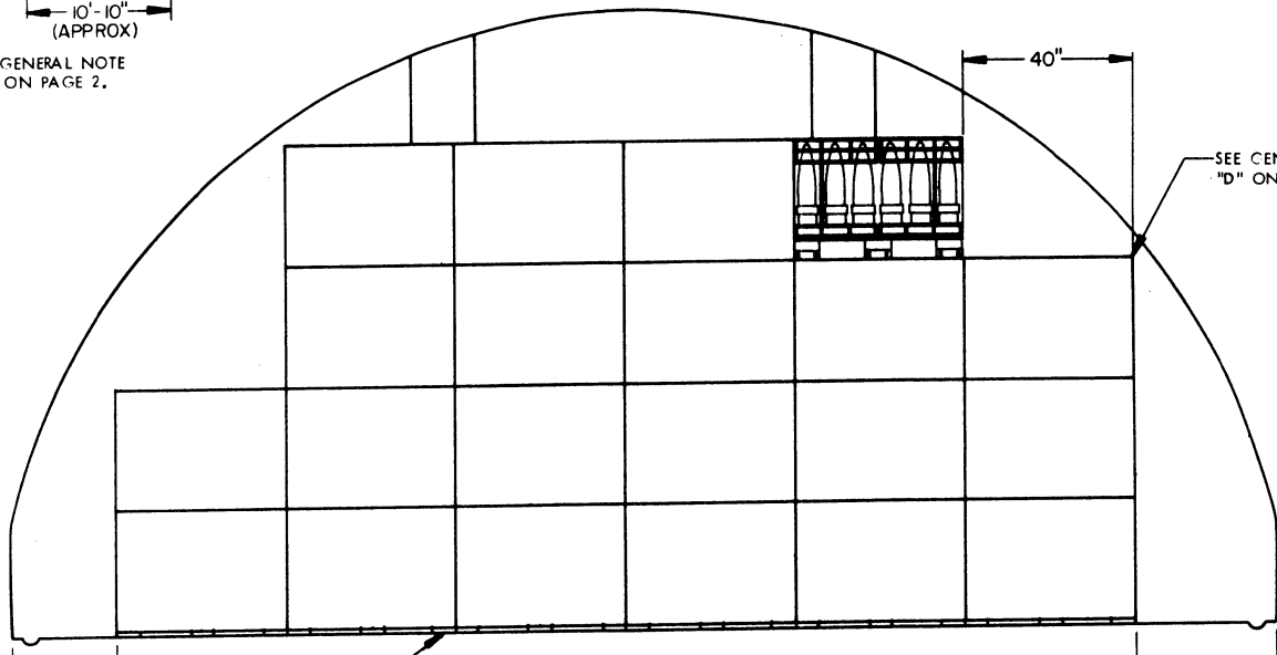
SECTION G-G ( "A" STACK, 21 PALLET UNITS )
