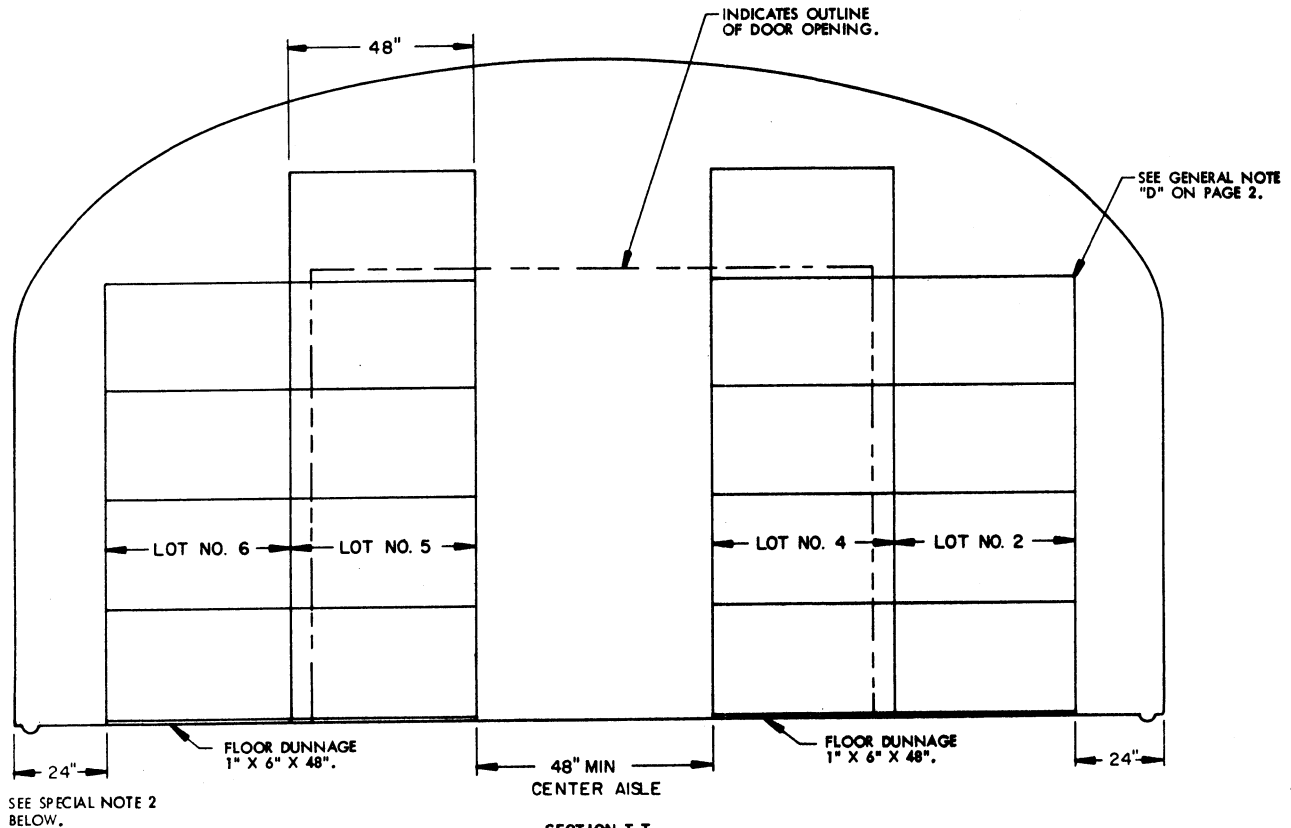
SECTION T-T
