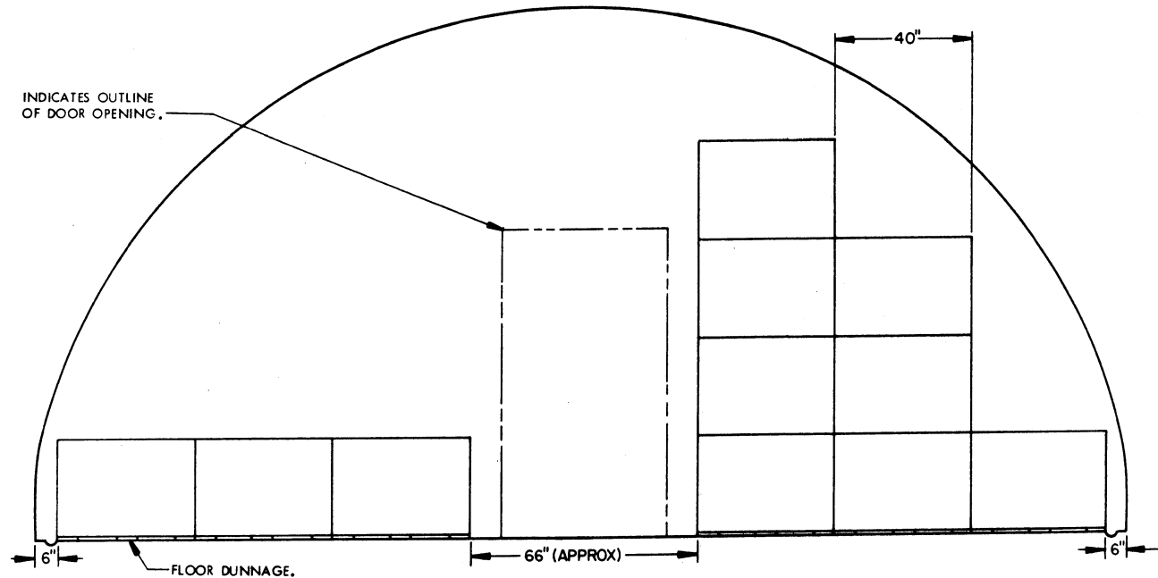
SECTION B-B ("C" STACK, 11 PALLET UNITS)
