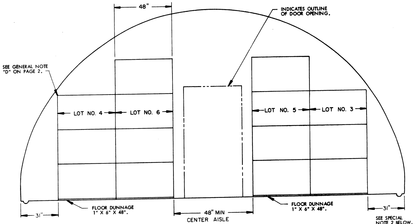
SECTION R-R
