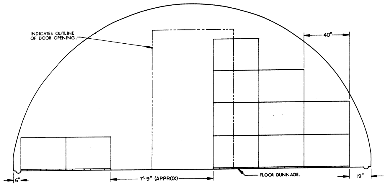
SECTION K-K ( "C" STACK, 11 PALLET UNITS )
