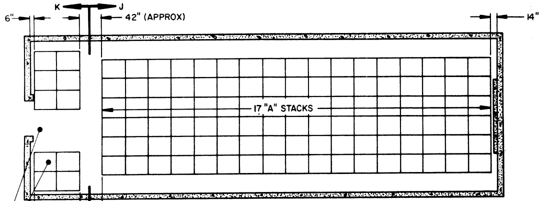
PLAN VIEW (81" MAGAZINE)
