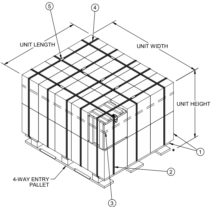
TYPICAL PALLET UNIT
