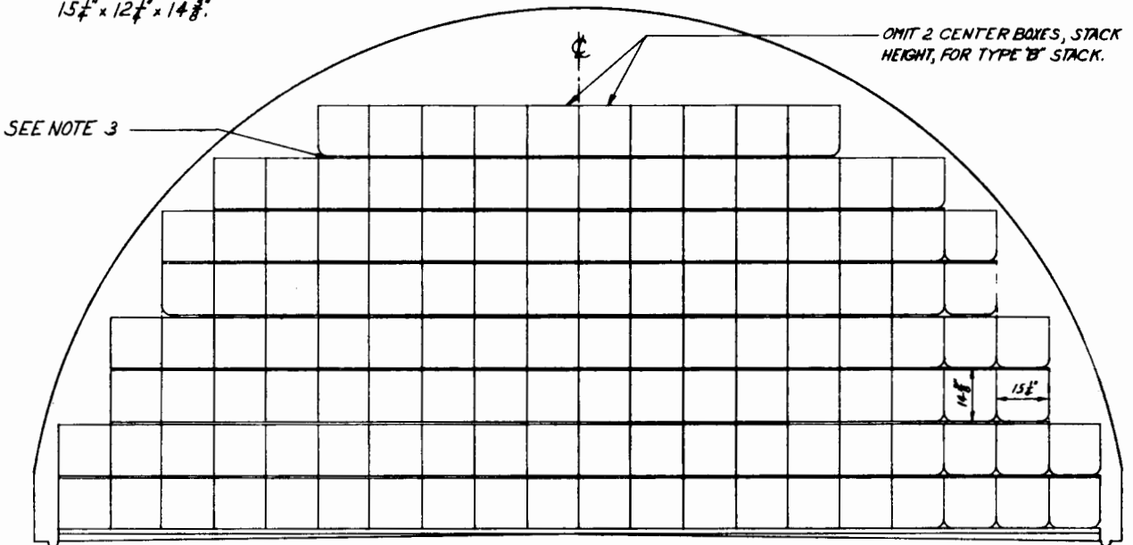
ELEVATION STACKS 'A' & 'B'
