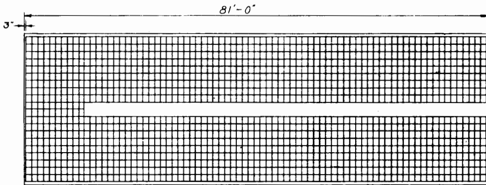
FLOOR PLAN STG. OF MK1 OR MK2 CNTRS.
