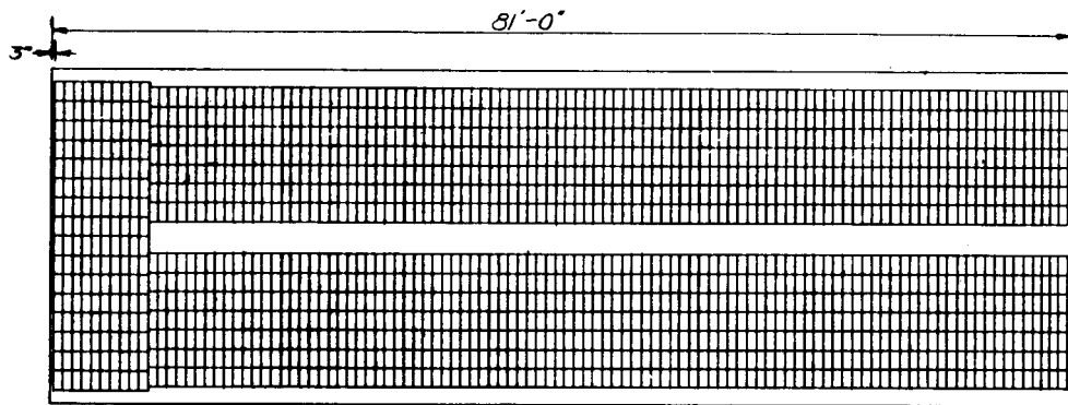
FLOOR PLAN - 80' IGL00 STG. OF MK3, MOD. 1 CNTRS.
