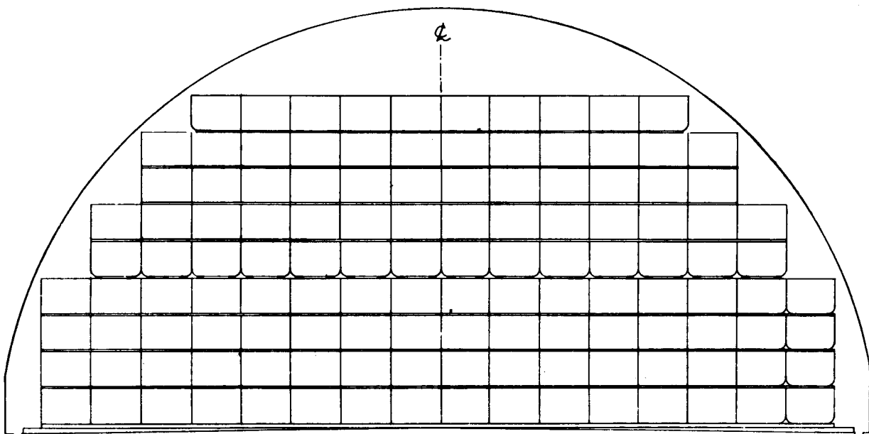
ELEVATION 'A' STACK
