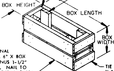
FILLER ASSEMBLY A (FOR MINUS ONE BOX)
