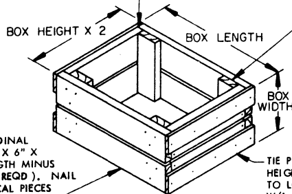
FILLER ASSEMBLY B (FOR MINUS 2 BOXES)
