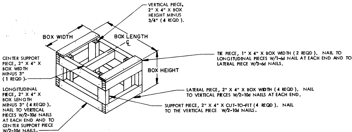
FILLER ASSEMBLY ( FOR MINUS ONE BOX )
