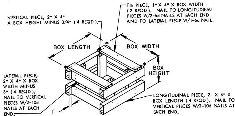
FILLER ASSEMBLY (FOR MINUS ONE BOX)
