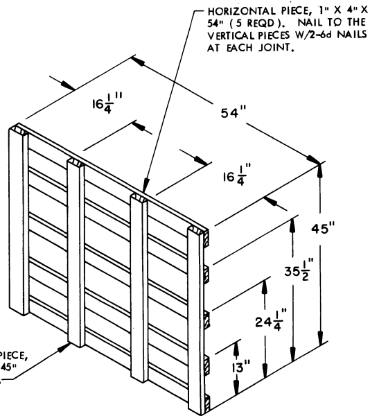
SPACER ASSEMBLY (ONE REQD)
