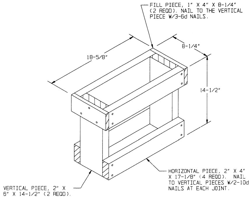
FILLER ASSEMBLY (FOR MINUS ONE BOX)
