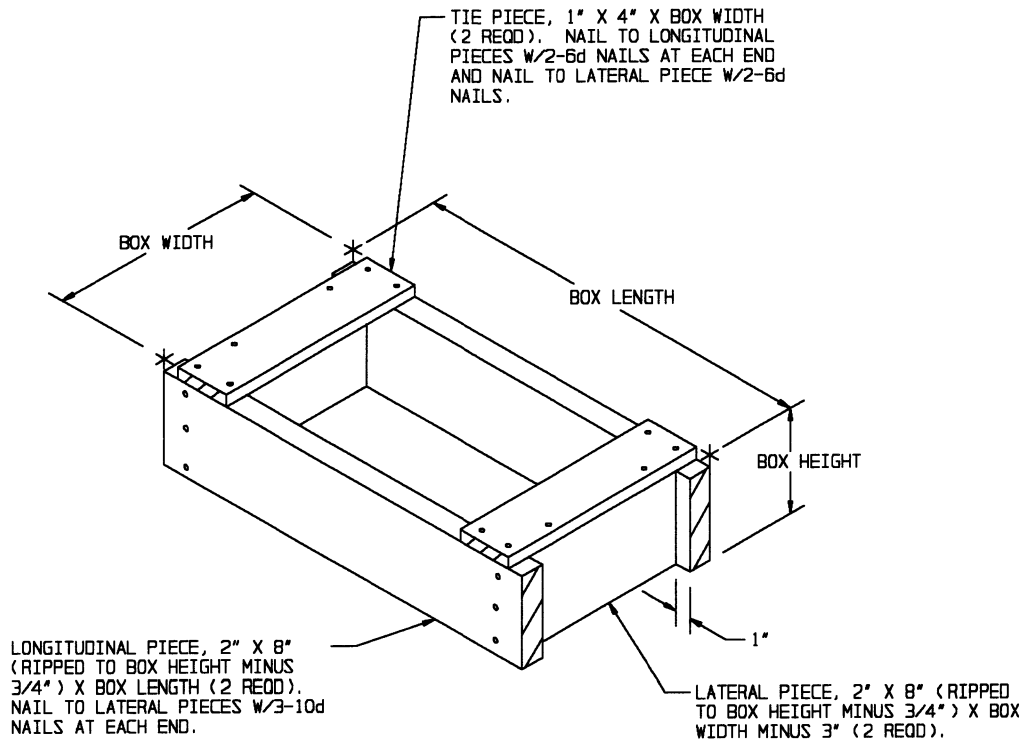
FILLER ASSEMBLY (FOR MINUS ONE BOX)
