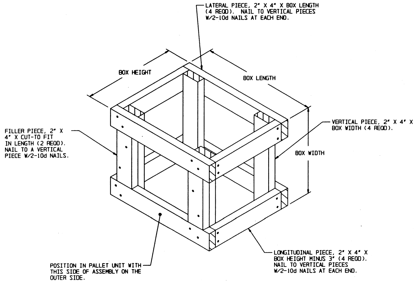
FILLER ASSEMBLY (FOR MINUS ONE BOX)
