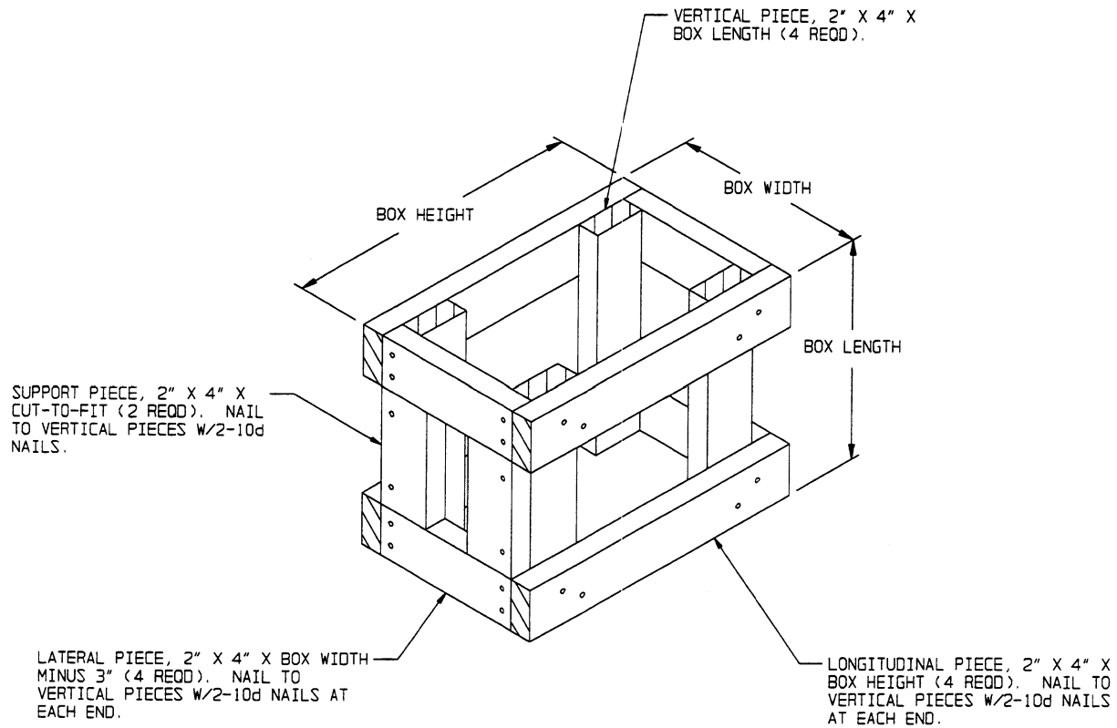
FILLER ASSEMBLY (FOR MINUS ONE BOX)
