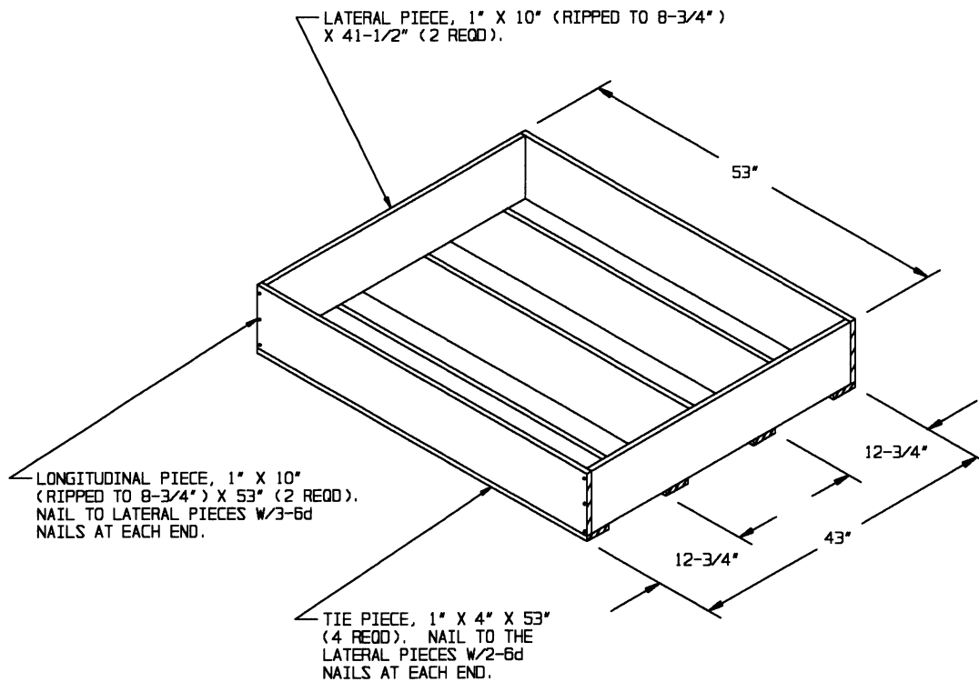
BASE ASSEMBLY
