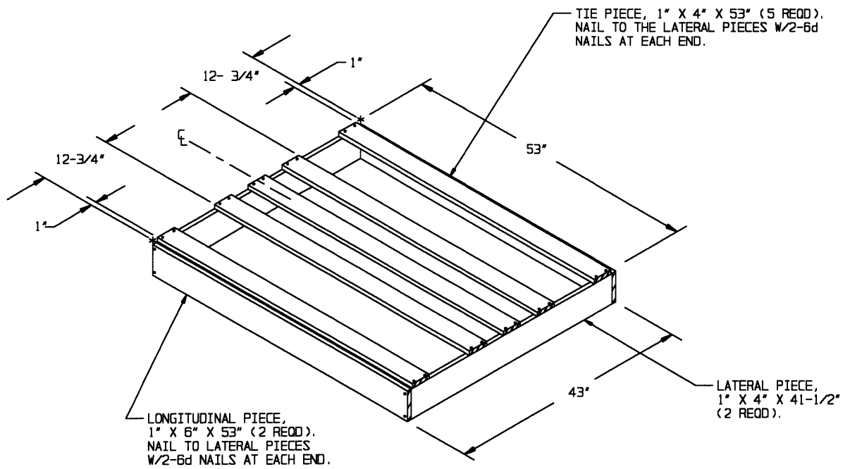
COVER ASSEMBLY
