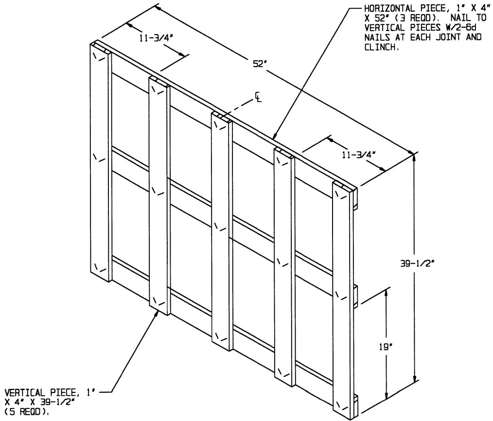
SPACER ASSEMBLY (2 REQD)
